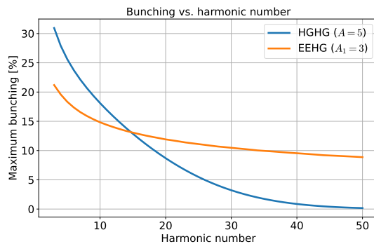
Figure 2: Comparison of the maximum obtainable bunching factor for HGHG and EEHG, according to the equations in [3, 4]. One can notice that for harmonic numbers \geq 15 , i.e., for shorter wavelengths, EEHG has significantly higher bunching, with reduced energy spread for better amplification. Parameters for HGHG: modulation amplitude A = 5 , chicane strength B optimized for maximum bunching. Parameters for EEHG: A_1 = 3 , B_1 = 32.1 , A_2 and B_2 optimized for maximum bunching.
