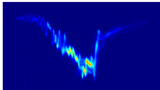
Figure 4: Heavily micro-bunched bunch prepared for accelerator studies.
