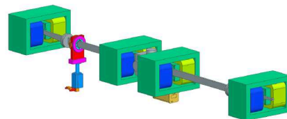
Figure 5: 3D CAD model of the bunching chicane CH2 .
