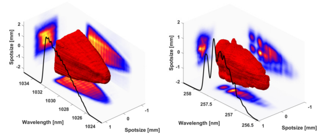
Figure 4: Spectrograph scans for triangle pulses with IR double shaper a) IR before conversion and b) after 2 consecutive conversions to UV.
