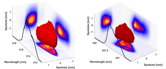
Figure 5: Spectrograph scans for triangle pulses with VIS single shaper a) VIS before conversion and b) after conversion to UV.
