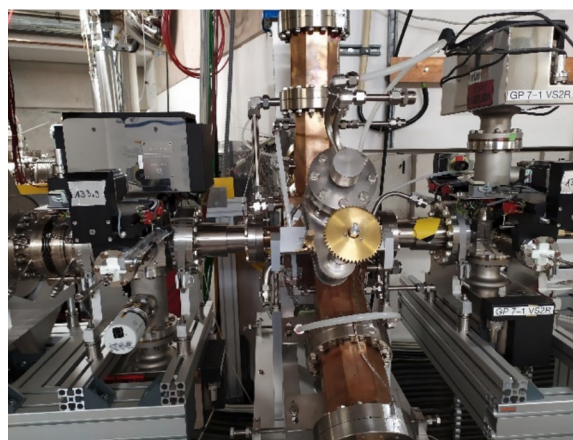
Figure 9: Third harmonic cavity installed in the BESSY II storage ring.
