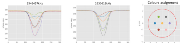
Figure 6: Measured data from two HOMs, for different bead pull position (mesh in the picture on the right, red circle is the vacuum chamber inner radius).
