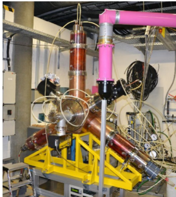
Figure 6: 500 MHz HOM BESSY-type damped cavity.
