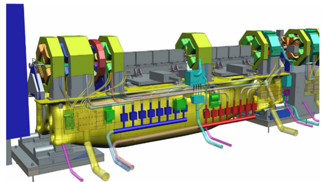
Figure 7: CAD model of fully loaded girders in the H6BA cell.
