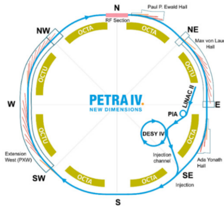
Figure 1: Layout of the PETRA IV accelerators and the experimental Halls.
