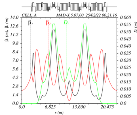
Figure 2: H6BA optics functions and layout from MAD-X.
