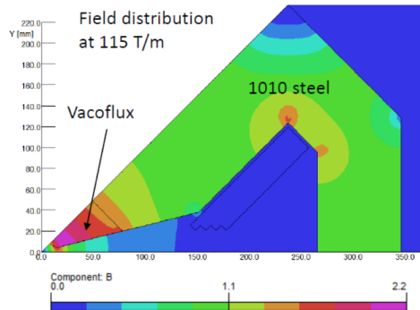
Figure 3: 2D cross section for the high gradient quadrupole PQA of PETRA IV.
