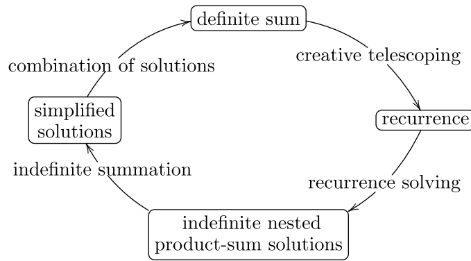
Figure 2. Sigma's summation spiral. Reproduced from [186]. CC BY 4.0.
