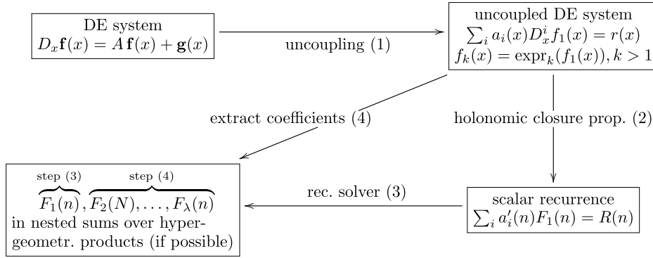
Figure 1. Solving systems.
