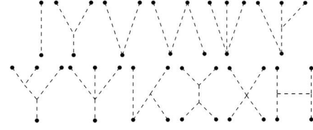
FIG. 1. Topologies needed for the N 2 LO potential (see text).
