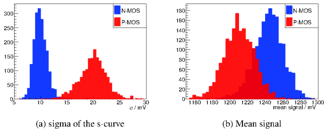
Figure 2: Results of the injection scans. Run2020-PMOS (Run2020-NMOS) in red (blue).
