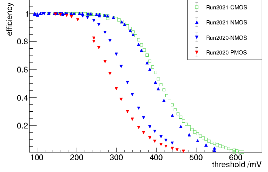
(a) Efficiency as a function of the detection threshold. Run2020 results from [11]. Statistical errors are too small to be seen.
