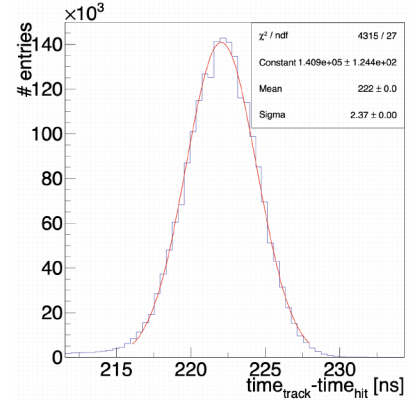
(b) Time resolution of the CMOS chip. Gaussian fit to the core of the distribution.
