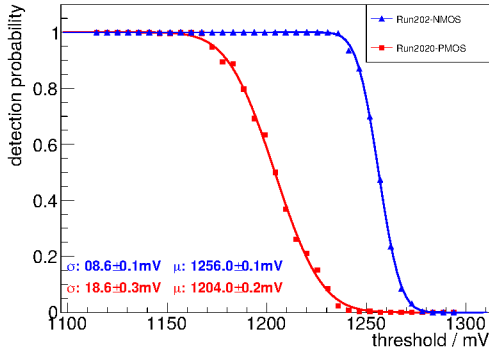
Figure 1: Exemplary response to the charge injection for Run2020-NMOS (blue triangles) and Run2020-PMOS (red squares). An s-curve is fitted to the data. The baseline is at 1 V.
