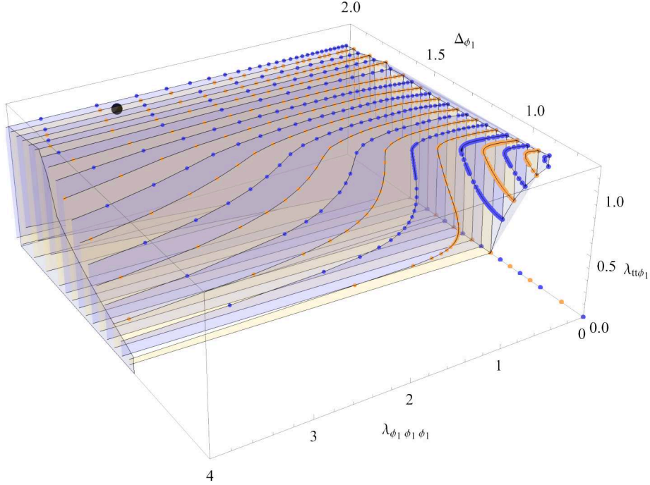
Figure 10. Bounds on the OPE coefficients \lambda_{t\bar{t}\phi_1} and \lambda_{\phi_1\phi_1\phi_1} as a function of the gap \Delta_{\phi_1} for the O(3) -breaking magnetic line defect. The black dot is the prediction from the \varepsilon -expansion. The gaps are given in eq. (4.10). \Lambda = 21, P = 41 .
