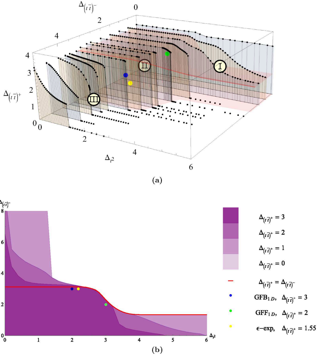
Figure 3. Bounds on the maximal gap on the dimension of the S -parity even scalar (t\bar{t})^+ (a) or S -parity odd scalar (t\bar{t})^- (b) vs. the S -parity odd (a) or even (b) scalar gap vs. the gap on the leading charged operator t^2 . \Lambda = 33, P = 53 . The green and blue dots correspond to the solutions for GFF and GFB, respectively. The yellow dot is the 1-loop \epsilon -expansion prediction for the magnetic line defect discussed in section 3.2. The solid red line in (b) is the ‘agnostic’ bound for \Delta_{(t\bar{t})^+} = \Delta_{(t\bar{t})^-} .
