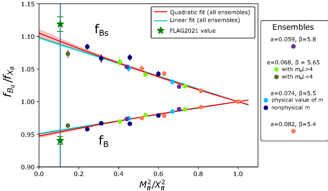
Figure 1: Fan plot of f_B/f_{B_x} and f_{B_s}/f_{B_x} , against the SU(3) breaking in the light quarks M_\pi^2/(1/3M_\pi^2 + 2/3M_K^2) .
