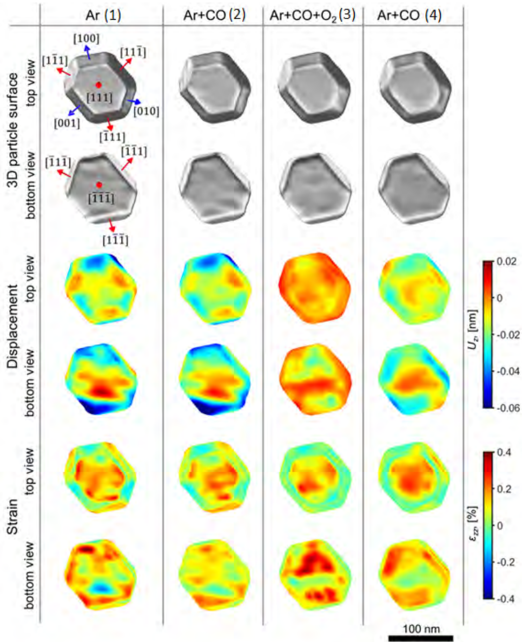
Figure 5.13.: Isosurface of the particle's electron density |\rho(\mathbf{r})| at 55% of its maximum value, superficial displacement U_z , and superficial strain \epsilon_{zz} for the respective gas dosing steps (compare steps 1-4 in Table 5.1). Displacement and strain values are projected onto the isosurface. Taken from supplemental material to [281].
