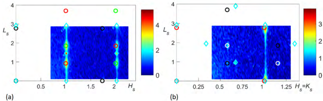
Figure 3.6.: 2D XRD maps in (a) H_S, K_S = 0, L_S and (b) H_S = K_S, L_S . Scans were taken with an integration time of 5 s. Calculated positions are indicated for \alpha - \text{Al}_2\text{O}_3 bulk (cyan diamonds), (111)-oriented Pt with ABC and CBA stacking (red and green circles, respectively), (111)-oriented Pt with 30^\circ rotation with respect to the surface normal (black and white respectively). Taken from [237].
