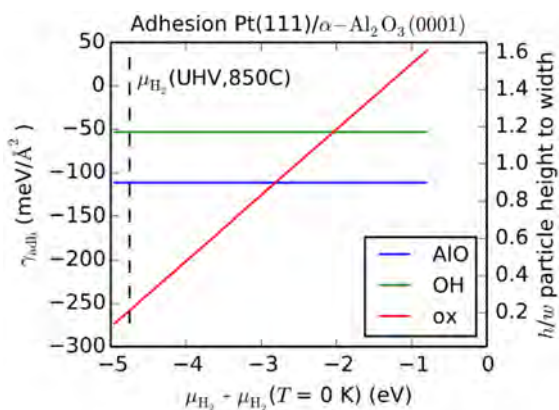
Figure 3.24.: Adhesion of Pt(111) on different surfaces/interfaces of \alpha\text{-Al}_2\text{O}_3 as a function of the hydrogen chemical potential. Figure through private communication, usage granted by P. Pleßow, see footnote 16.
