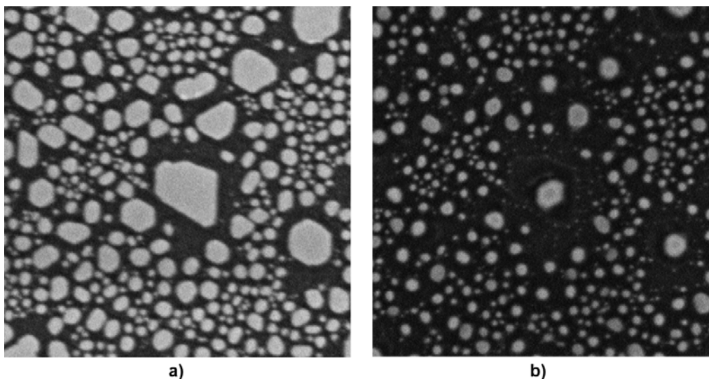
Figure 4.11.: Zoom-in of areas marked in orange in Figure 4.10. Corresponding SEM-images were taken after the catalytic experiments at 370 °C (a) and after 450 °C (b), respectively. The centred particle in (a) exhibits a lateral dimension of 180 nm along the horizontal plane of the image.
