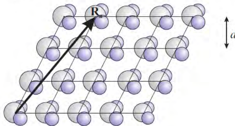
Figure 2.17.: Scattering scheme with objects on different length scales relating \mathbf{Q} , \mathbf{k} , and \mathbf{k}' : (a) single atom, (b) a molecule, and (c) a crystal composed of molecules at positions \mathbf{R}_n . The lattice spacing of the crystal is d . Figure taken from [205].
