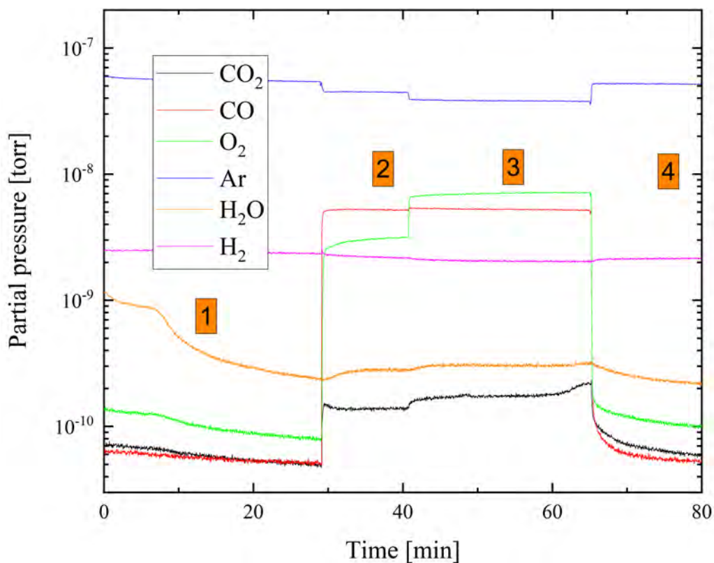
Figure C.14.: Catalytic test on a bare Nb-doped STO substrate. Highlighted numbers indicate following gas dosing steps (total flow 50 \frac{\text{ml}}{\text{min}} , total pressure 0.1 bar, temperature 450^\circ\text{C} ): (1) Ar only, (2) 4 \frac{\text{ml}}{\text{min}} CO and 4 \frac{\text{ml}}{\text{min}} \text{O}_2 with Ar carrier gas, (3) 4 \frac{\text{ml}}{\text{min}} CO and 8 \frac{\text{ml}}{\text{min}} \text{O}_2 with Ar carrier gas, and (4) Ar only.
