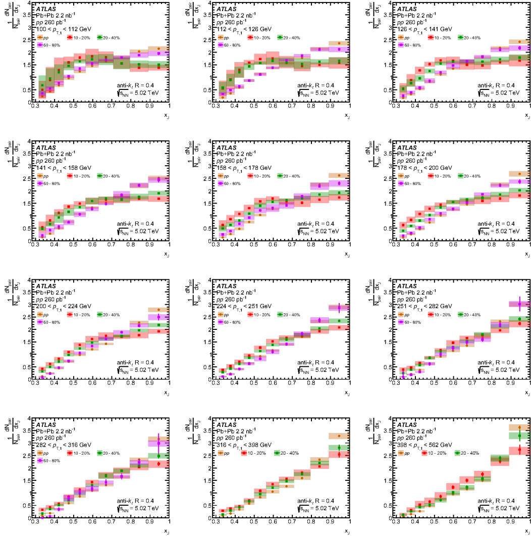
Figure 16: The unfolded dijet-yield-normalized x_J distributions in both Pb+Pb and pp collisions for twelve p_{T,leading} selections from 100 GeV to 562 GeV. The results in Pb+Pb collisions are shown in three centrality selections, 10–20%, 20–40% and 60–80%. Statistical uncertainties are shown as error bars and systematic uncertainties are shown as boxes.
