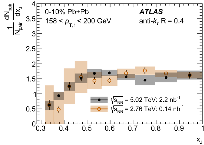
Figure 10: Comparison of the measured x_J distribution at 5.02 TeV in 0–10% centrality collisions for 100 < p_{T,1} < 126 GeV (top), 126 < p_{T,1} < 158 GeV (middle), and 158 < p_{T,1} < 200 GeV (bottom) with those at 2.76 TeV from Ref. [11]. Statistical uncertainties are shown as error bars (which are smaller than the markers in many cases) and systematic uncertainties are shown as boxes.
