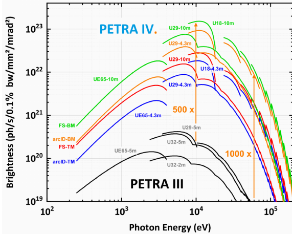
Fig. 4 Spectral brightness of PETRA IV (H6BA lattice) compared to PETRA III. The colours denote different modes of operation and ID-cell lengths. The green, orange, red, and blue colours correspond to a 10 m insertion device (ID) in brightness mode, a 4.3 m ID in brightness mode, a 10 m ID in timing mode, and a 4.3 m ID in timing mode, respectively.
