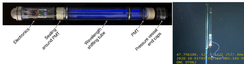
Figure 16. A demonstrator device made in the prototype configuration and photographed under UV illumination (left). The electronics comprise a PMT pulse readout, environmental sensors, and communication. After deployment, a photograph was taken by a robot in the Ocean Network Canada. (right). Right picture: Courtesy of the ONC.
