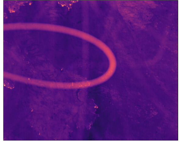
(b) Daytime TIR imagery of wildfires taken on July, 28th 2021 at 06:29:59 UTC over central Siberia, Russia.
