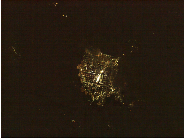
Figure 15: TUBIN night time VIS image of Las Vegas in the United States taken on November, 2nd 2021 at 09:23:16 UTC.
