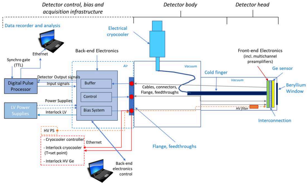
Figure 1: General layout of the XAFS-DET detector with main components.
