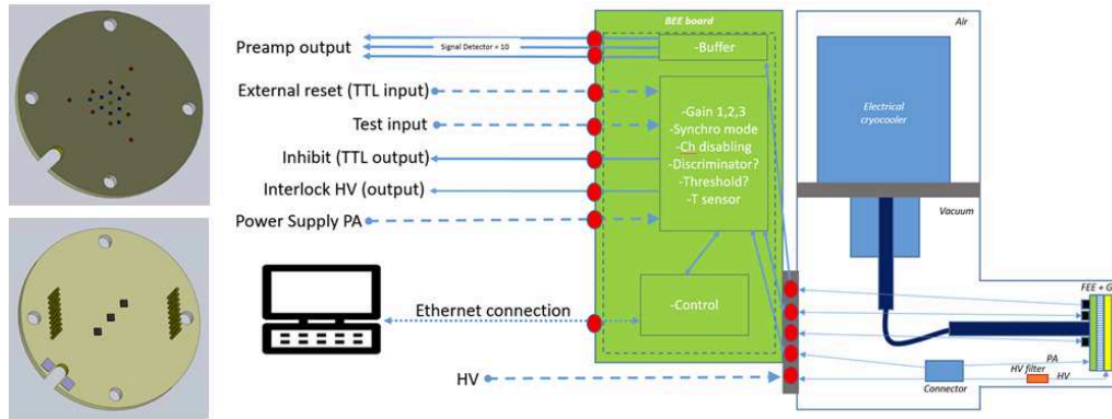
Figure 3: Overview of the front-end board electronic (left): top side of the board matching both the small and large pixels arrangement (top-left) and its back side (bottom-left); Schematic overview of the functionalities of the back-end electronics (right).
