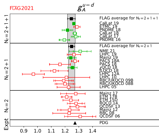
Fig. 43 Lattice results and FLAG averages for the isovector axial charge g_A^{u-d} for N_f = 2, 2+1 and 2+1+1 flavour calculations. Also shown is the experimental result as quoted in the PDG [165]
