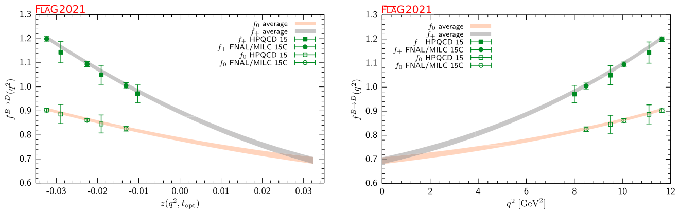
Fig. 34 The form factors f_+(q^2) and f_0(q^2) for B \rightarrow D\ell\nu plotted versus z (left panel) and q^2 (right panel). See text for a discussion of the data sets. The grey and salmon bands display our preferred N^+ = N^0 = 3 BCL fit (five parameters)
