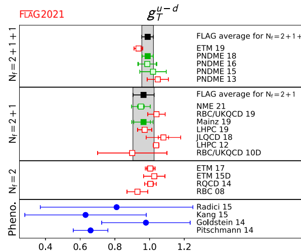
Fig. 45 Lattice results and FLAG averages for the isovector tensor charge g_T^{u-d} for N_f = 2, 2 + 1 , and 2 + 1 + 1 flavour calculations. Also shown are phenomenological results using measures of transversity [986–990] (circles)
