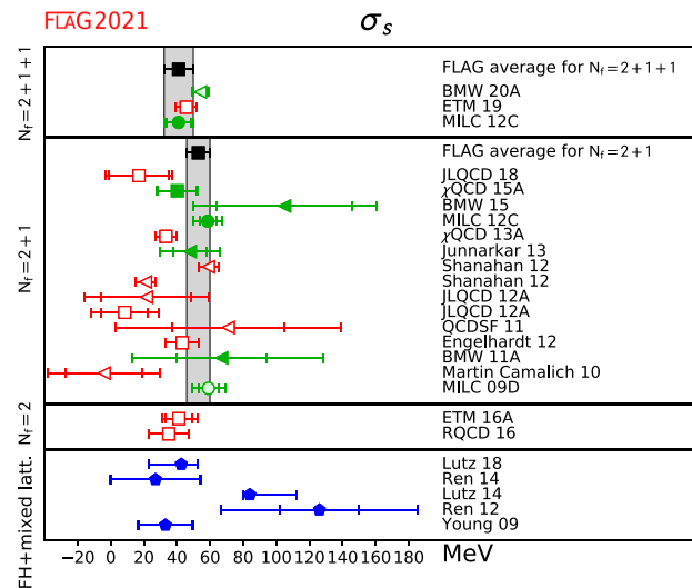
Fig. 48 Lattice results and FLAG averages for \sigma_s for the N_f = 2, 2 + 1 , and 2 + 1 + 1 flavour calculations. Determinations via the direct approach are indicated by squares, the Feynman–Hellmann method by triangles and the hybrid approach by circles. Results from calculations which analyze more than one lattice data set within the Feynman–Hellmann approach [1022, 1023, 1025, 1026, 1029] are shown for comparison (pentagons)
