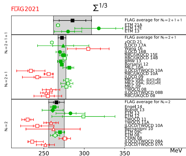
Fig. 14 Cubic root of the SU(2) quark condensate \Sigma \equiv -\lim_{m_u, m_d \rightarrow 0} \langle \bar{u}u \rangle in the \overline{\text{MS}} -scheme, at the renormalization scale \mu = 2 \text{ GeV} . Square symbols indicate determinations from correlators in the p -regime, up triangles refer to extractions from the topological susceptibility, diamonds to determinations from the pion form factor, and bullet points refer to the spectral density method
