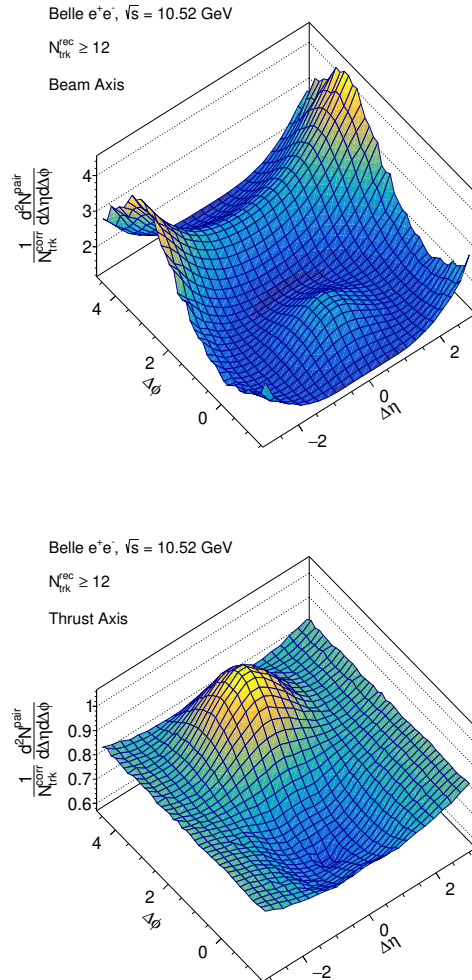
FIG. 1: Two-particle correlation functions for beam (top) and thrust (bottom) axis analyses with the multiplicity N_{\text{trk}}^{\text{rec}} \geq 12 .
