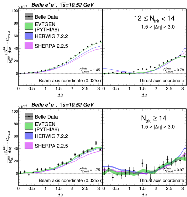
FIG. 2: Comparison of ZYAM-subtracted Y(\Delta\phi) in the range 1.5 < |\Delta\eta| < 3.0 for the multiplicity 12 \leq N_{\text{trk}}^{\text{rec}} < 14 (top) and N_{\text{trk}}^{\text{rec}} \geq 14 (bottom), where subtracted constants of data C_{ZYAM}^{\text{Data}} are quoted. In each panel, results for beam (left) and thrust (right) axis analyses are displayed. The colored bands show simulation predictions from Belle MC (green), HERWIG (blue), and SHERPA (violet). The error bars on the data represent the statistical uncertainties, and the gray boxes are systematic uncertainties. For visual purposes, the minimal statistical uncertainty of the MC colored bands is set to be 3 \times 10^{-4} , and beam-axis ZYAM-subtracted yields are scaled by a factor of 0.025.
