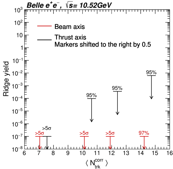
FIG. 3: Upper limits of the ridge yield as a function of \langle N_{\text{trk}}^{\text{corr}} \rangle in beam axis (red) and thrust axis (black) coordinate frames. Thrust axis limits are shifted to the right by 0.5 for presentation purposes. The label “ > 5\sigma ” indicates the 5\sigma confidence level upper limit.
