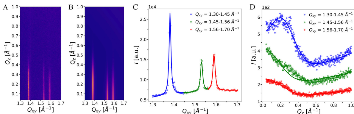
Fig. 3 (A) GIXD pattern (intensity vs. Q_{xy} and Q_z ) of an OL monolayer at 20 \text{ mN m}^{-1} on water subphase at pH 3. (B) Modeled intensity. (C) Q_z -integrated intensity vs. Q_{xy} . The lines represent fits to the data points. (D) Piece-wise Q_{xy} -integrated intensity vs. Q_z . The integration ranges are given in the legend. Data and fits are shifted vertically for clarity.
