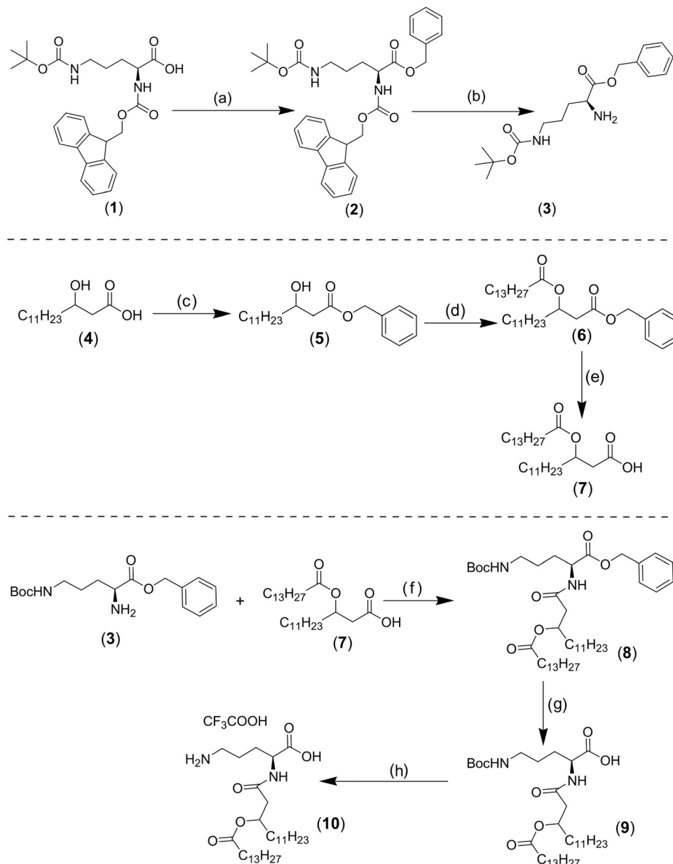
Fig. 2 OL synthesis. Reagents and conditions: (a) DCC, DMAP, CH 2 Cl 2 , 0 °C, 24 h; (b) pyrrolidine, CH 2 Cl 2 , RT, 1 h; (c) benzyl bromide, Bu 4 NI, TEA, EtOAc, RT, 24 h; (d) myristoyl chloride, pyridine, CH 2 Cl 2 , 0 °C then RT; (e) Pd/C, H 2 , RT, 3 h; (f) i -BuOCOCl, N -methylmorpholine, THF, 30 min at −15 °C then RT 24 h; (g) Pd/C, H 2 , RT, 2 h; (h) CF 3 COOH.
