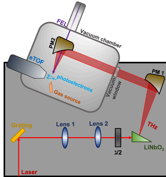
Figure 3.3: Schematic layout of the THz-streaking setup installed at the FL21 beamline of FLASH2. It consists of two parts, the THz production via tilted pulse-front in a \text{LiNbO}_3 crystal using an IR laser and the UHV chamber located above the optical table, where the FEL and THz beams are collinearly overlapped and focused in the interaction region.
