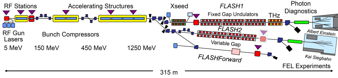
Figure 3.1: Schematic view of the Soft-X-ray FEL FLASH in DESY. It shows the main components of an FEL, the electron bunch injector, acceleration cavities, undulator section to produce FEL radiation and the 2 experimental halls.
