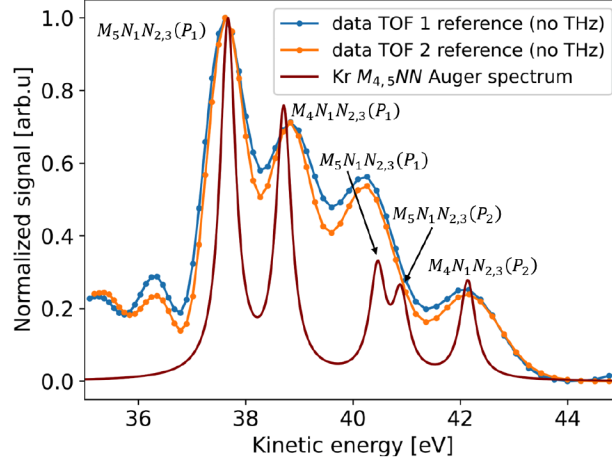
Figure 4.5: Reference spectra (without THz field) measured simultaneously with TOF1 and TOF2. Each spectrum consists of an average of \sim 200 FEL pulses. Five Kr (MNN) Auger transitions are plotted in red using the data from [107, 108] in order to identify the Auger peaks.
