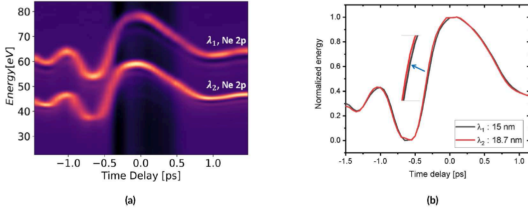
Figure 4.1: (a) Kinetic energy of neon 2p photoelectrons in the presence of the THz field as a function of the time delay between the FEL and THz pulses. The spectra were taken simultaneously for the two colors delivered at FLASH2 ( \lambda_1 : 83 eV and \lambda_2 : 66 eV). (b) Streaking traces of the two colors normalized to their maximum. It reveals that the relative average arrival time between the two photoelectrons is shifted by \sim 15 fs.
