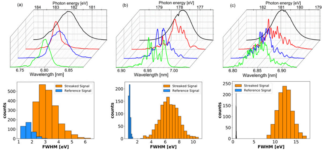
Figure 6. Upper row: XUV spectra for different pulse duration settings. Column (a): represents the case \tau_{\text{XUV}} < 30 fs; (b): 30 \text{ fs} < \tau_{\text{XUV}} < 150 fs; (c): \tau_{\text{XUV}} > 150 fs. Green, blue and red lines are examples of single-shot spectra measured with the PG spectrometer. Black curves represent the average spectra. One can clearly see the different number of spectral spikes/modes for the different settings. The lower row shows the corresponding histograms for the eTOF spectral width (FWHM in eV) for streaked and un-streaked (reference) spectra. While for the long pulse duration (column (c)) the width fluctuations of the reference (un-streaked) spectra is negligible, for the short pulses (column (a)) there is a significant overlap showing the need of a careful consideration of the reference pulses.
