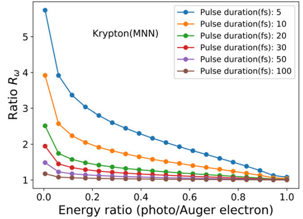
Figure 4. The same as in figure 1 but for the krypton Auger spectral line M_{5,2,3}N_{2,3}(^1P_1) .
