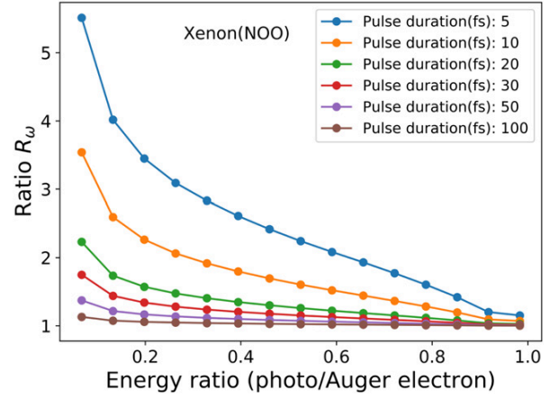
Figure 3. The same as in figure 1 but for the xenon Auger spectral line N_{5,2,3}O_{2,3}(^1S_0) .
