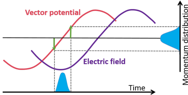
Figure 2.4: Streaking of a Fourier limited XUV pulse. The photoelectron distribution produced via photoionization by an XUV pulse is probed around the zero-crossing of the streaking vector potential. The photoelectrons emitted before and after the zero-crossing are decelerated and accelerated respectively by the streaking field. This results in a broader spectrum as compared to the field-free case.
