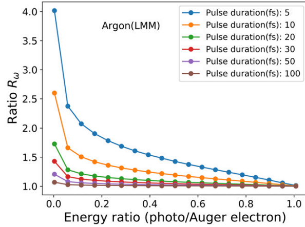
Figure 2. The same as in figure 1 but for the argon Auger spectral line L_{3,2,3}M_{2,3}(^1S_0) .
