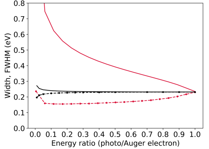
FIG. 7. The widths of the Auger line calculated for the emission in the forward (solid lines) and the backward (dashed lines) directions as a function of the ratio of the excess and Auger electron energies. The calculations have been performed for the zero crossing point of the THz vector potential. The result of the calculations using the present quantum mechanical model are shown as black lines, the results of the analytical semiclassical model of Ref. [29] are shown as red lines (lighter gray). The calculations have been done for an XUV pulse duration of 5 fs for an excess energy of 1 eV and THz field strength of 60 kV/cm.
