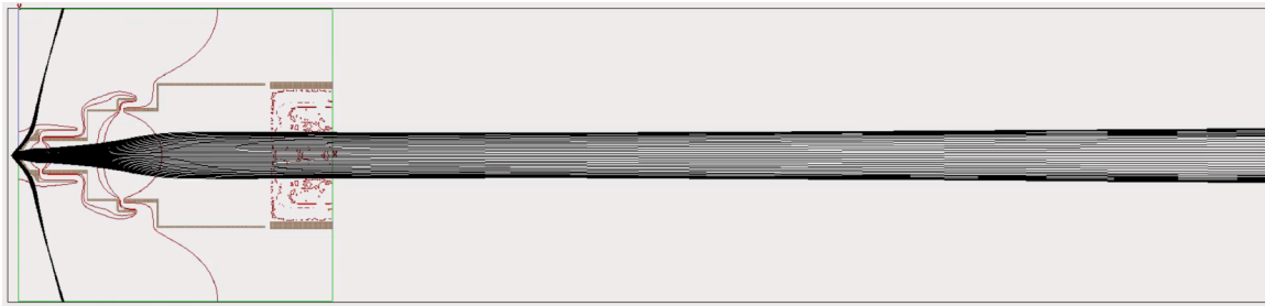
Figure 3.5: SIMION screenshot of electron trajectories in the eTOF spectrometer. The electrons (black lines) enter the eTOF on the left side and arrive to the MCP detector at the end of the right side. The photoelectrons' kinetic energy was set to 64 eV, the lens voltage to 430 V and the retardation voltage to 30 V.
