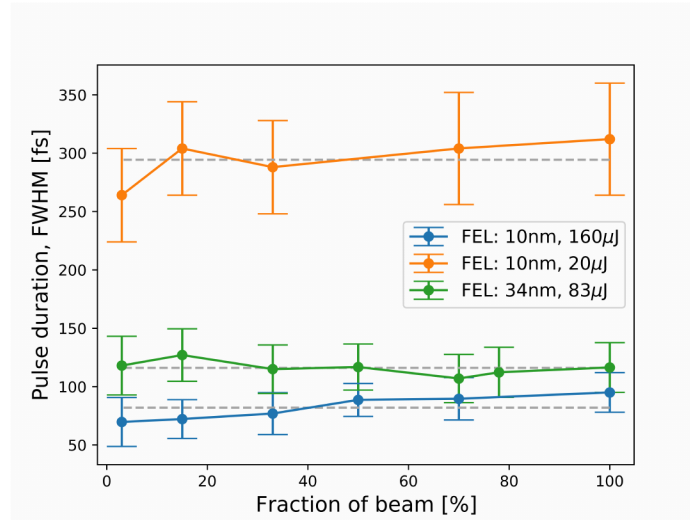
Figure 3.9: Average pulse duration measurements over \sim 3000 shots at different mirror positions for different FEL settings. The bar in each point indicates the distribution of the measurement. The dotted line depicts the average value of all measurements for a fixed FEL setting.
