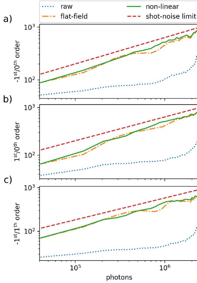
Fig. 7. SNR (Inverse of the standard deviation) of the data binned as a function of the intensity in the 0 th order for a) the -1 st /0 th order, b) the +1 st /0 th order and, c) the -1 st /+1 th order. Data that are only dark-corrected are shown as dotted blue lines. Data that are also flat-field corrected are shown as dotted-dashed orange lines. Data that are also corrected for non-linearity are shown as continuous green lines. The photon shot-noise limit is shown as dashed red lines.
