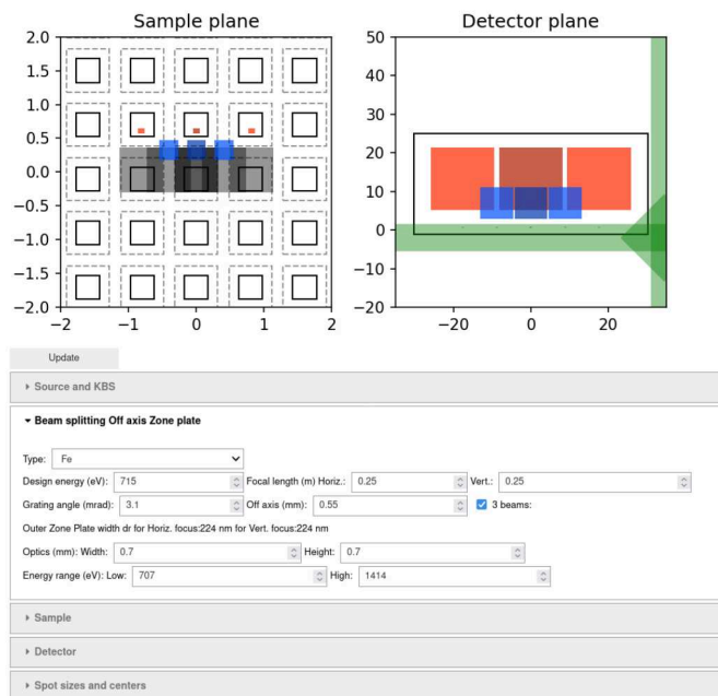
Fig. 3. BOZ calculator showing the beams at the sample and detector planes as well as the control settings below. The focused 1 st zone-plate order beam footprint at the respective positions is shown as red for the fundamental and blue for the second harmonic. The 0 th zone plate order is shown as gray. Individual membrane windows and the etching lines are shown in the sample plane figure as continuous and dashed lines, respectively. In the detector plane figure, the DSSC sensor is represented by the black rectangle and the DSSC filter mount is represented by the green shapes. Dimensions in both figures are in millimeters.
