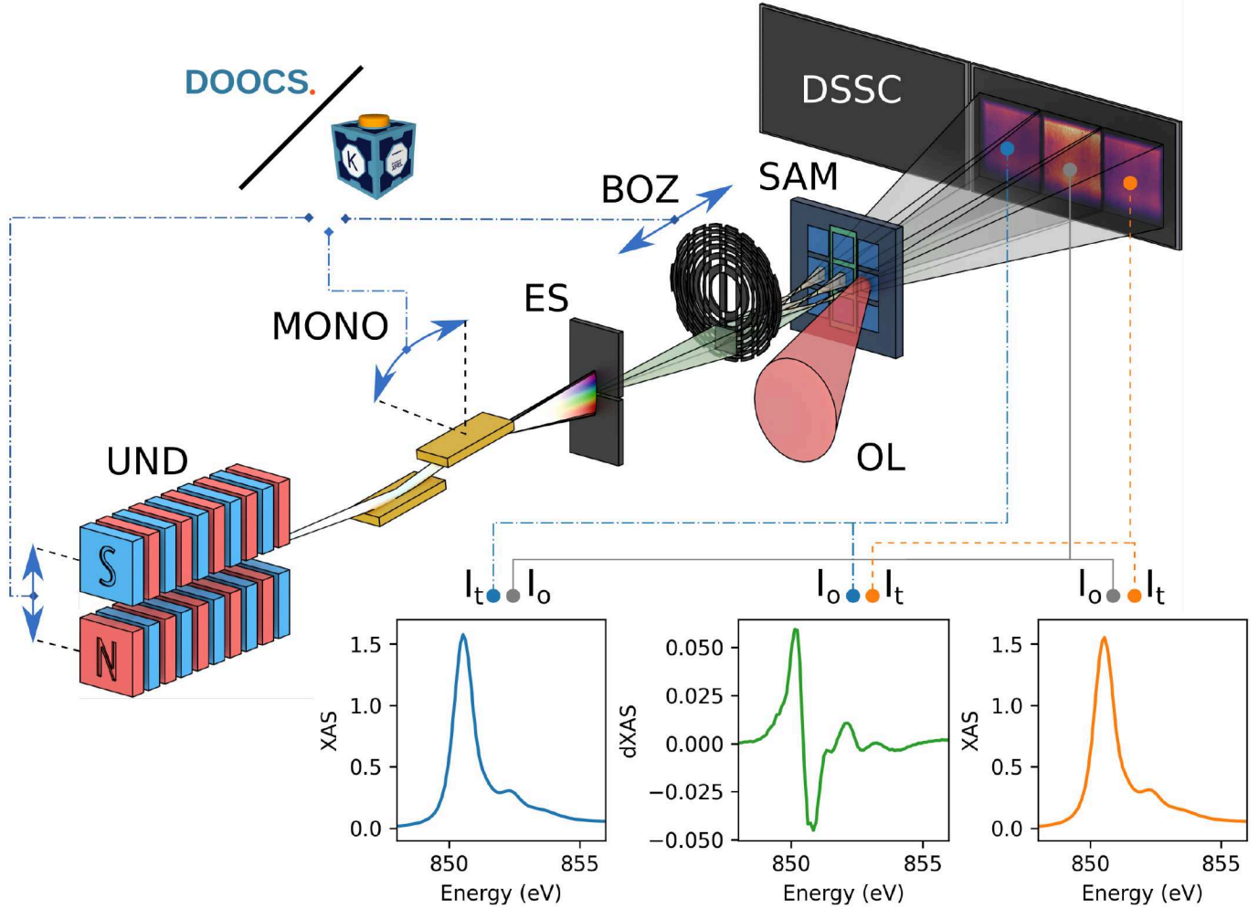
Fig. 1. Scheme of the beam-splitting off-axis zone plate (BOZ) setup. SASE FEL pulses are produced in the SASE3 undulators (UND). A variable line spacing plane grating (MONO) is placed 130 m downstream and disperses the SASE pulses on the exit slit (ES) placed 100 m further downstream. The monochromatic X-rays then propagate 30 m further and are split into three beams of equal intensity and focused down in front of the sample by the beam-splitting off-axis zone plate (BOZ). The sample (SAM) consists of three X-ray transparent membranes that are aligned on these three beams. The X-ray spot size on the membrane is typically 50 \times 50 \mu\text{m}^2 . The middle membrane is used as a reference and is either a clear aperture or a bare membrane, while the other membranes contain the sample of interest, here a NiO thin film. The three beams further propagate and expand onto one sensor of the DSSC detector placed 5.4 m downstream. At the bottom of the figure, the resulting XAS spectra at the Ni L_3 edge are shown for the unexcited sample on the left, the sample excited by the optical laser (OL) on the right, as well as their measured difference in the middle. Above each of the three XAS plot, we identify the beam used as reference ( I_o ) and the beam used as transmission ( I_t ). During an energy scan, the DOOCS and Karabo control systems ensure that the gap size of the 120 m long undulator follows the monochromator photon energy. Similarly, the zone plate
