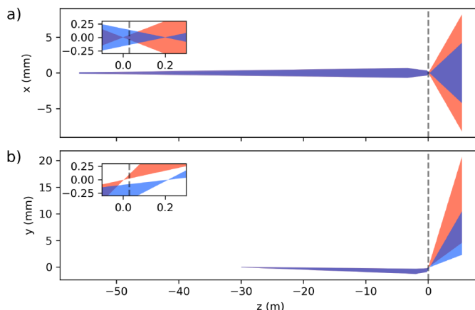
Fig. 2. a) Horizontal and b) vertical beam propagation from the intermediate source point to the detector. The position of the sample is shown as a dashed vertical line. The inset in each figure shows a zoomed-in region around the sample position. The red-filled areas represent the 707 eV photon beams from the fundamental harmonic of the undulators. The blue-filled areas represent the beams at 1414 eV photon energy originating from the second harmonic of the undulators. The vertical separation between fundamental and second harmonic beams near the zone-plate focus arising from the off-axis component of the diffractive optics can be used to block the unwanted radiation.
