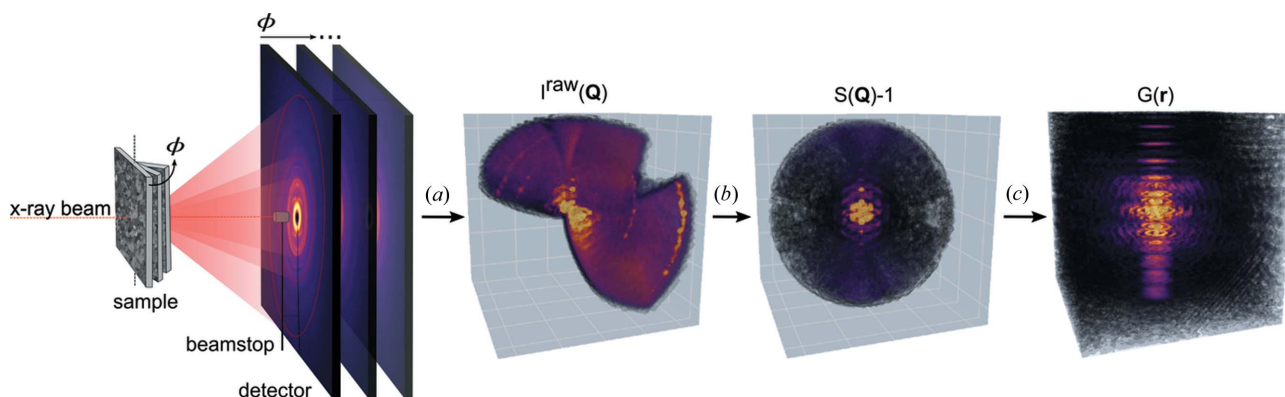
Figure 4 The experimental and data-processing procedure. (a) Reconstruction of a tilt series of 2D scattering images to a 3D scattering volume I(\mathbf{Q}) . (b) Processing to the total scattering structure function S(\mathbf{Q}) , with application of symmetry averaging, interpolation, and cutoff beyond Q_{\min} and Q_{\max} . (c) Fourier transformation to the txPDF G(\mathbf{r}) .
