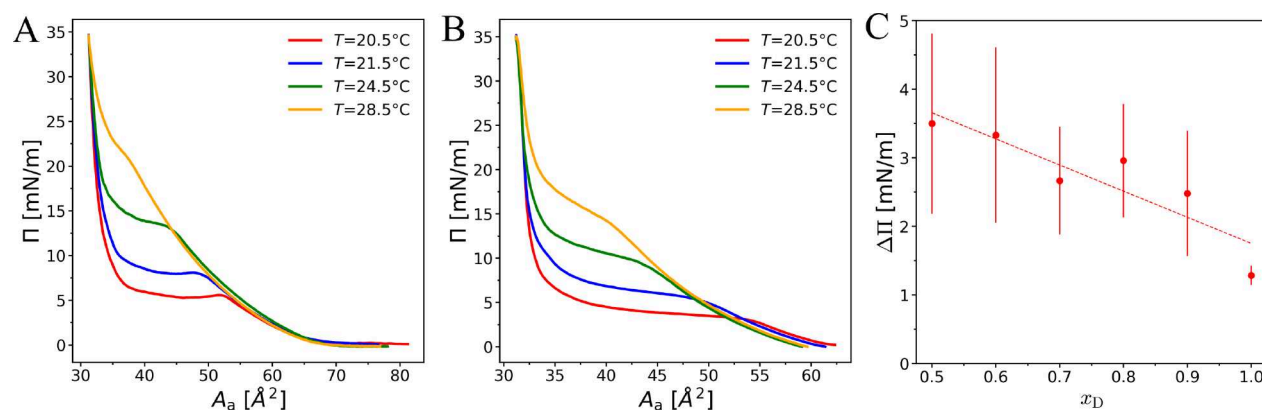
Figure 2. (A and B) Temperature-dependent pressure–area isotherms of an N -stearoyl-threonine monolayer with x_D = 0.9 at compression (A) and at expansion (B). The hysteresis between compression and decompression curves is clearly visible. (C) The difference in transition pressure between compression and expansion, \Delta\Pi , as a function of x_D . The values were taken at A_a = 40 \text{ \AA}^2 and averaged over four temperatures. The error bars are the standard derivation of the data points at different temperatures. The dotted straight line represents a linear fit to the data points.
