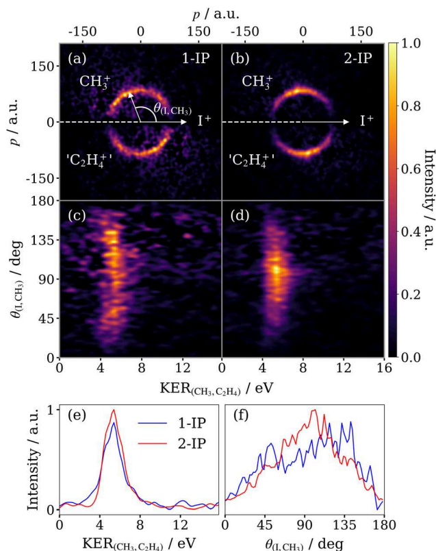
Fig. 7 Newton diagrams for the sequential breakup of (a) 1-IP 3+ and (b) 2-IP 3+ into ( \text{I}^+ + \text{CH}_3^+ + \text{C}_2\text{H}_4^+ ) in the COM frame of the secondary dissociation \text{C}_3\text{H}_7^{2+} \rightarrow \text{CH}_3^+ + \text{C}_2\text{H}_4^+ . The Newton diagrams are displayed in polar coordinates in (c) and (d) respectively, where \text{KER}_{(\text{CH}_3, \text{C}_2\text{H}_4)} is the KER of the secondary products and \theta_{(\text{I}, \text{CH}_3)} is the angle between the momenta of the iodine and methyl ions. Each panel is normalised separately. Below are overlaid the integrated KER (e) and angular distributions (f) for both isomers, normalised to unit area.
