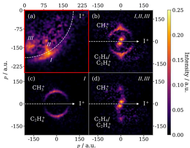
Fig. 6 (a) Momentum distribution of \text{I}^+ covariant with \text{CH}_3^+ , produced from the three-body breakup of 2-IP 2+/3+ . The red box around this panel is to highlight the different scale for the momentum axes, and the different frame in which these data are presented. The three dissociation channels are as follows: (I) sequential three-body breakup of 2-IP 3+ , (II) concerted three-body breakup of 2-IP 3+ , (III) three-body breakup of 2-IP 2+ . (b) Newton diagram for the same process, displaying the \text{CH}_3^+ momentum in the COM frame of the charged propyl intermediate. Filtering based on the absolute \text{I}^+ momentum has been used to isolate (c) the sequential breakup channel of 2-IP 3+ ( 190 < p_{\text{I}^+} < 225 a.u.) from (d) the signal due to concerted breakup of 2-IP 3+ as well as three-body breakup of 2-IP 2+ ( 120 < p_{\text{I}^+} < 190 a.u.).
