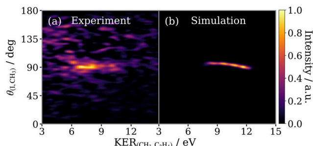
Fig. 8 Experimental (a) and simulated (b) covariance maps for concerted three-body breakup of 2\text{-IP}^{3+} as a function of KER of the secondary products ( \text{KER}_{(\text{CH}_3, \text{C}_2\text{H}_4)} ) and the relative recoil angle between the iodine and methyl ions ( \theta_{\text{I}, \text{CH}_3} ). Each panel is normalised separately.
