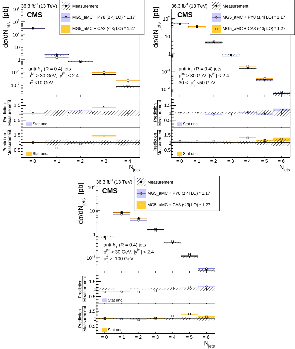
Figure 4: Jet multiplicity in three different regions of p_T(Z) : p_T(Z) < 10 GeV (upper left), 30 < p_T(Z) < 50 GeV (upper right), p_T(Z) > 100 GeV (lower). The error bars on the data points represent the statistical uncertainty of the measurement, and the hatched band shows the total statistical and systematic uncertainties added in quadrature. Predictions from MG5_AMC+PY8 ( \leq 4j LO) and MG5_AMC+CA3 ( Z \leq 3j LO) are shown. Different normalization factors are applied, as described in the text.
