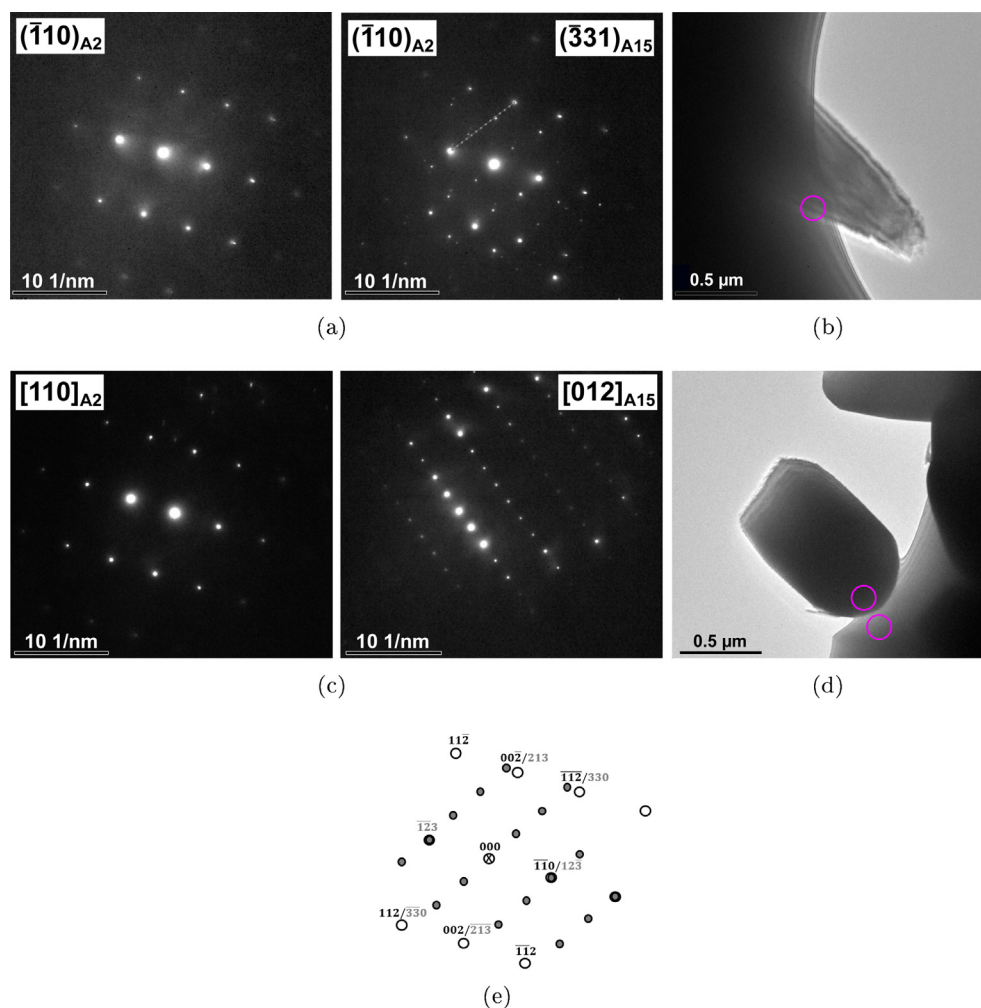
Fig. 7. In (a) and (c) selected SADPs of \text{Cr}_{91}\text{Si}_7\text{Pt}_2 after 100 h at 1200^\circ\text{C} annealing are shown. In (b) and (d) the corresponding microstructures of the ternary alloy are shown and the areas from which the SADP were taken are marked. In (a) the pattern is taken from the \text{Cr}_{ss} matrix and at the \text{Cr}_{ss}/\text{A15} interface, where patterns of both phases are observed. The patterns in (c) are received in the \text{Cr}_{ss} matrix and, with the same sample tilt, of the interior of an A15 precipitate in the vicinity. In (e) an indexed schematic of (a) is shown.
