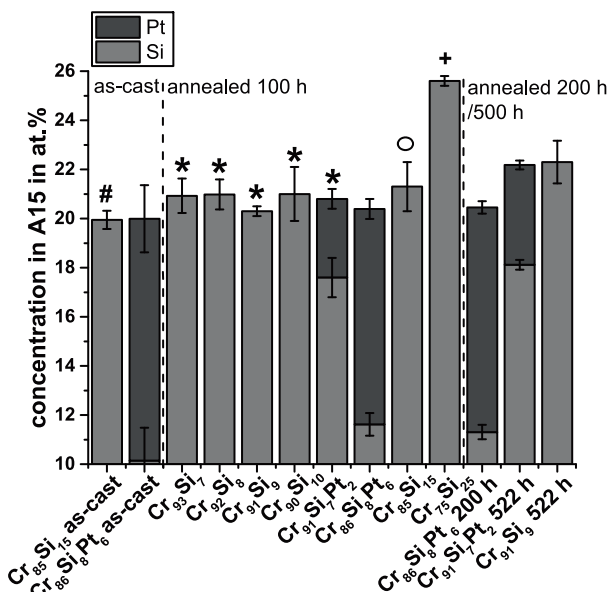
Fig. 3. Concentration of the A15 phase former Si and Pt over alloy composition and heat treatment. The results obtained in this work are compared to other previous studies [32], [33], [6], and [10]. In all cases a sub-stoichiometric composition of the A15 phase is found except for the pure A15 phase alloy ( \text{Cr}_{75}\text{Si}_{25} in at.%).
