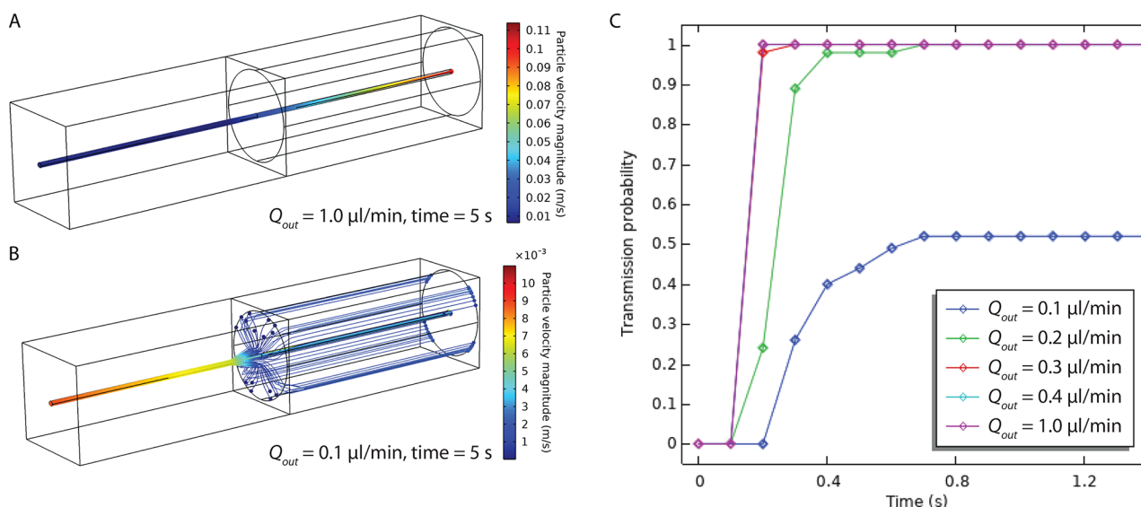
Figure 9. Particle tracing simulation of focusing at 40 \mu\text{L/min} and injection to a small-bore capillary ( 20 \mu\text{m} ) aligned with the acoustic focus. (A) With an outflow of 1 \mu\text{L/min} , all particles entering the system within the acoustic focus go to the center outlet, and (B) with an outflow of 0.1 \mu\text{L/min} , half of the particles go to the center. (C) The transmission probability (acoustic focus to central outlet) goes to 1 for outflows above 0.2 \mu\text{L/min} . With this outflow and the acoustic focus presented herein, it is therefore possible to achieve enrichment factors of around 200 with optimal alignment.
