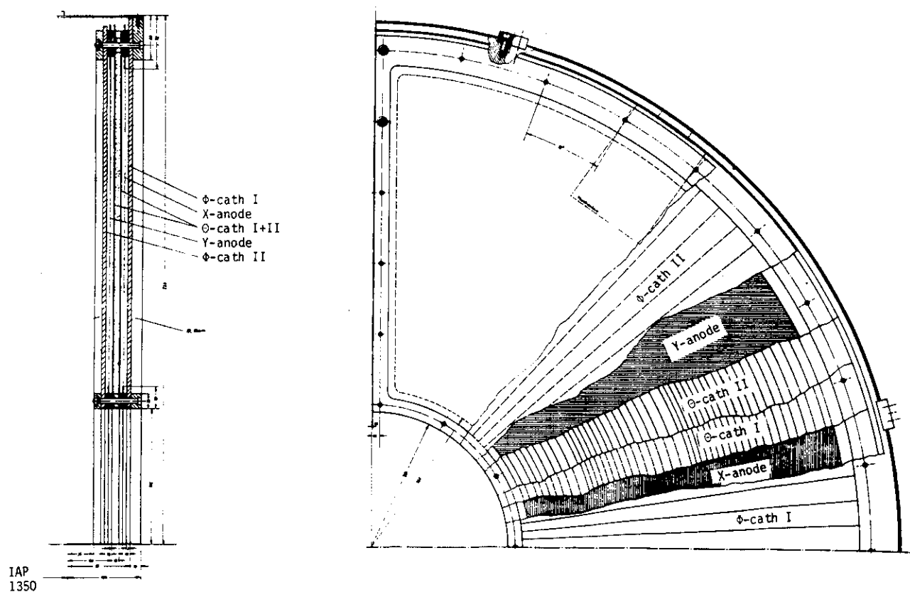
Fig. 10: Layout of the Endcap Multiwire Proportional Chambers
