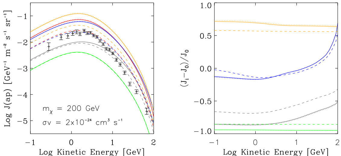
FIG. 5: Left panel : Comparison of the local spectrum of antiprotons from 200 GeV Wino DM ( \langle\sigma v\rangle = 2 \times 10^{-24} \text{ cm}^3 \text{ s}^{-1} ) for different propagation models (the color coding is the same as in Fig. 2), assuming a modulation potential as given in Table II and the three spherical halo model profiles introduced in Table I (solid: Einasto profile, dotted: NFW, dashed: Burkert). Right panel : Fraction ratio between the different local spectrum and the KRA model. In some cases solid and dotted curves coincide.
