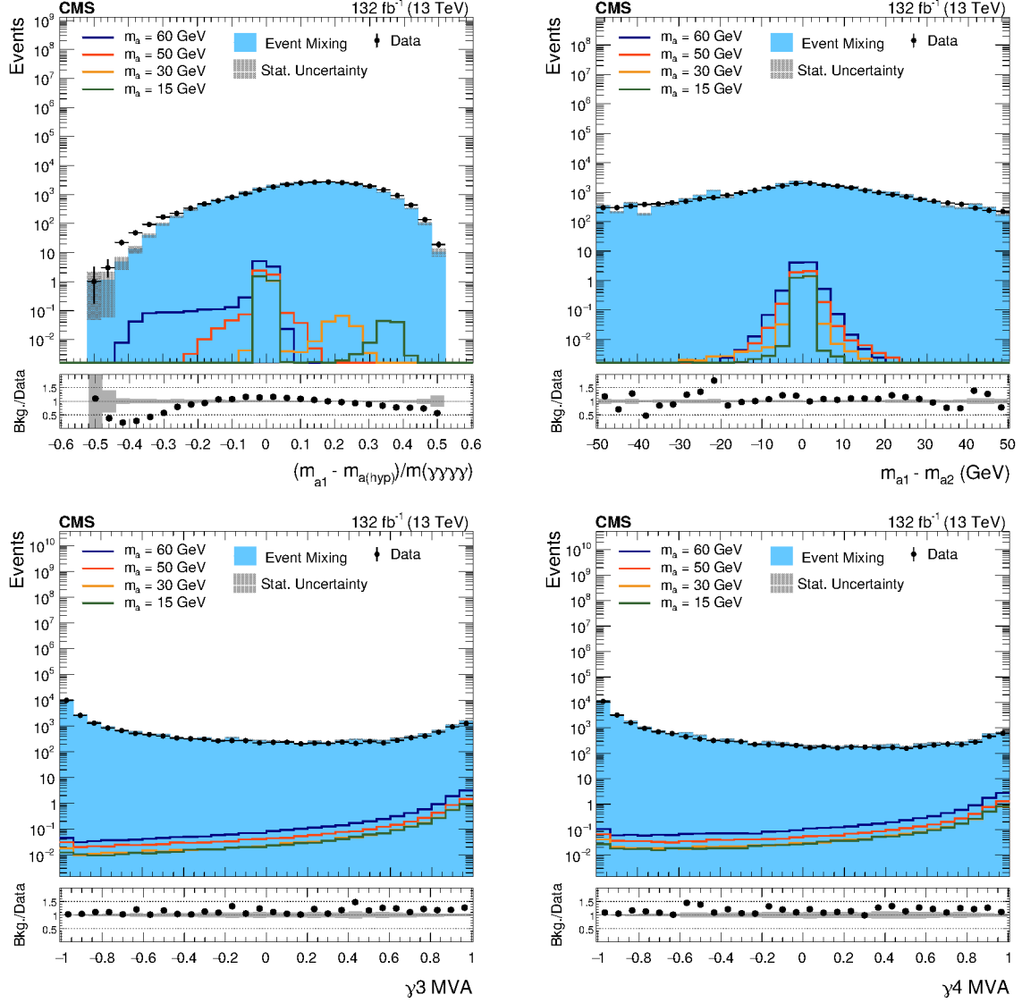
Figure 2: Distributions of the four most highly ranked discriminating variables: the difference between the invariant masses of the pseudoscalar bosons and the m_{a,hyp} parameter, divided by the invariant mass of the four-photon system (upper left), with off-zero signal peaks from photon pairing mismatches; the difference between the invariant masses of the pseudoscalar boson (upper right); the photon identification BDT score of the third leading, \gamma_3 (lower left) and the fourth leading, \gamma_4 (lower right) photons. The events shown are selected from the m_{\gamma\gamma\gamma\gamma} sidebands ( 110 < m_{\gamma\gamma\gamma\gamma} < 115 GeV or 135 < m_{\gamma\gamma\gamma\gamma} < 180 GeV) for event mixing and data after fulfilling the selection criteria described in Section 4, while the signals are scaled with a cross-section of 1 pb.
