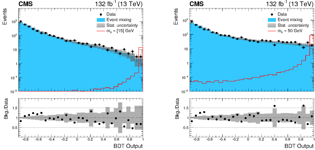
Figure 3: Distribution of the BDT output for m_a = 15 \text{ GeV} (left) and 50 \text{ GeV} (right) in data and simulated signal and event mixing (after smoothing) events. Events shown are selected after fulfilling the selection criteria described in Section 4 in the mass window 110 < m_{\gamma\gamma\gamma\gamma} < 180 \text{ GeV} , while the signal is scaled with a cross-section of 1 \text{ pb} .
