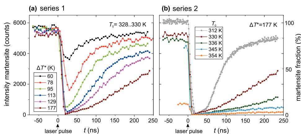
Figure 2. Probing the time dependency of a martensitic transformation while heating with a laser pulse and subsequent cooling. The summed up intensity of the (16\ 2\bar{0})_{MM} peak allows to determine the martensite fraction, which reduces sharply during heating with the 7 ns laser pulse and increases afterwards when the sample cools down. Two series with different experimental conditions were investigated: (a) Nearly the same base temperature of around T_0 = 329 K was used for all measurements and the laser fluence was varied to obtain temperature rises \Delta T^* between 60 K and 177 K. (b) the laser fluence and therefore \Delta T^* was kept constant at 177 K, but the base temperature was varied between 312 K and 354 K.
