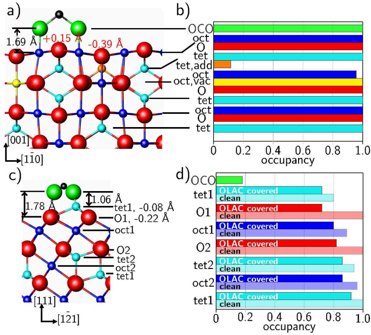
Figure 2: Structural changes upon OLAC adsorption. Structural model obtained from SXRD fit of magnetite (001) (a) and (111) (c) with atomic displacements with respect to the bulk positions. Figs. b) and d) show the occupancy profiles obtained from the SXRD fits which correspond to the respective atomic layer of the unit cell in a) and c) for magnetite (001) and (111), respectively. Magnetite oxygen is shown in red, carboxylate oxygen in green, carbon in black, octahedral iron in blue, tetrahedral iron in light blue, octahedral vacancy sites in yellow and tetrahedral interstitial ions in orange.
