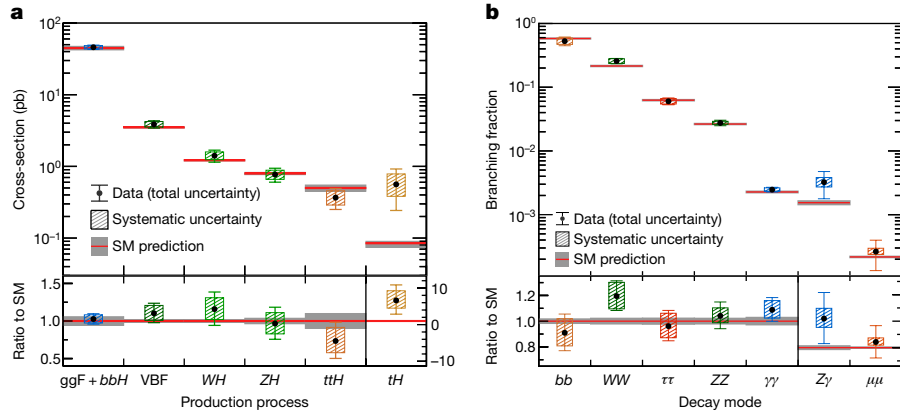
Fig. 2 | Observed and predicted Higgs boson production cross-sections and branching fractions. a , Cross-sections for different Higgs boson production processes are measured assuming standard model (SM) values for the decay branching fractions. b , Branching fractions for different Higgs boson decay modes are measured assuming SM values for the production cross-sections.
