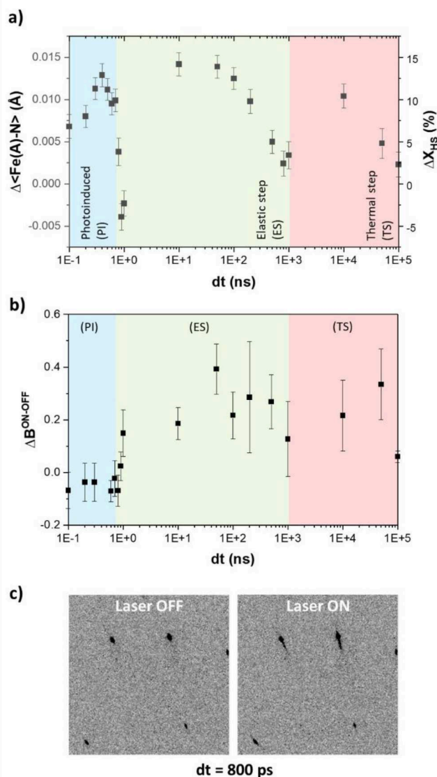
Figure 2 a) Time-delay dependence of \Delta\langle\text{Fe(A)-N}\rangle associated with the variation of the HS fraction, \Delta X_{\text{HS}} . b) Time dependence of the isotropic thermal factor, \Delta B_{\text{ON-OFF}} . Photoinduced (PI), elastic (ES) and thermal (TS) steps are shown in blue, green and red, respectively. c) Crystallographic images of the 800ps data set, showing a deformation of the Bragg peaks between the laser-OFF and laser-ON.
