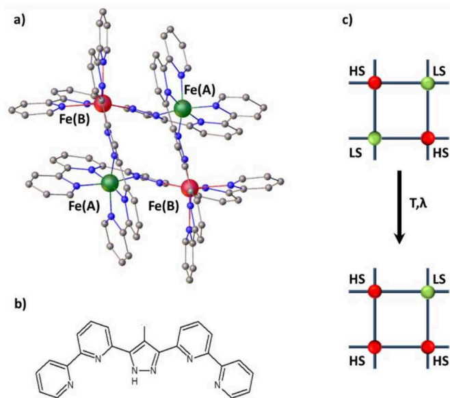
Figure 1 a) Molecular representation of the [\text{Fe}_4\text{L}_4]^{4+} grid. Fe(A) ions are in LS state and Fe(B) ions are in HS states. Counter ions, solvent molecules and hydrogen atoms are omitted for clarity. b) Pyrazole-bridged compartmental ligand \text{HL}^{\text{Me}} . c) Schematic representation of the 2HS-2LS to 3HS-1LS transition in the FE4 grid. LS and HS ions are shown in green and red, respectively.
