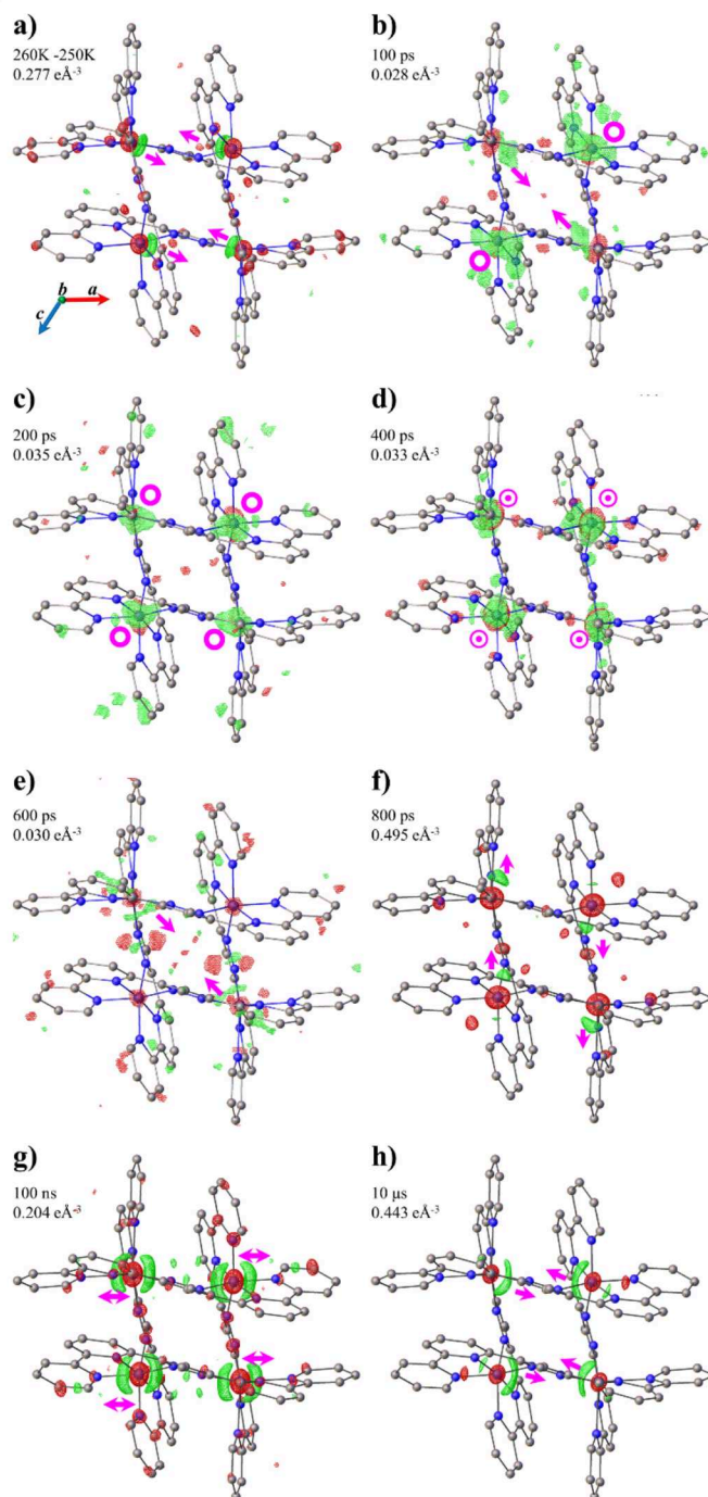
Figure 3 a) Thermal difference Fourier maps of FE4 between 260 and 250K. b-h) Photodifference maps of FE4 along the b axis. Isosurfaces (green positive, red negative) and delay times are shown on each figure. Arrows give approximate directions of the electron density shift. The symbol \ominus indicates an outside and inside of the plane electron density shift, while \odot symbols indicate only out-of-the-plane electron density shifts.
