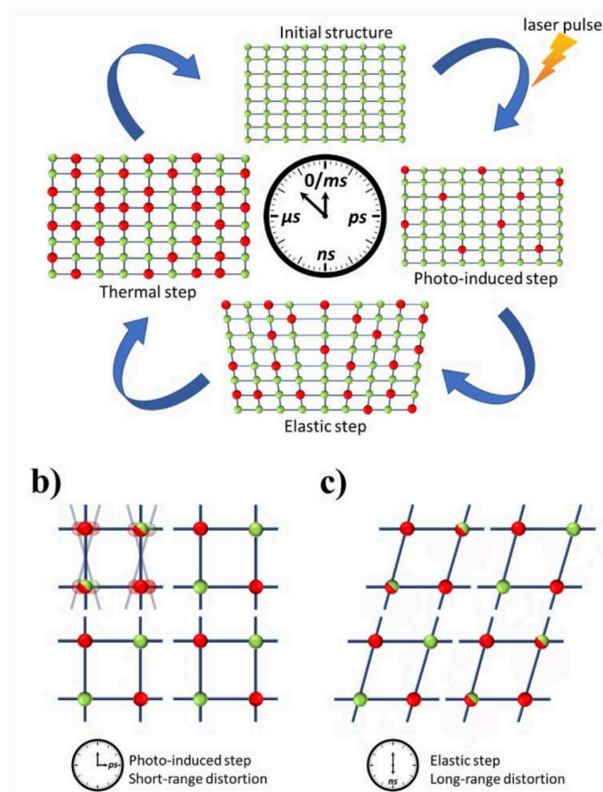
Figure 6 Schematic representation of a) the out-of-equilibrium process in SCO complexes, b) the short-range distortion in FE4 and c) long-range distortion in FE4 . Green and red spheres represent LS and HS Fe II ions, respectively. Half-red half-green spheres represents the transiting metal centre in two crystallographically identical sites.
