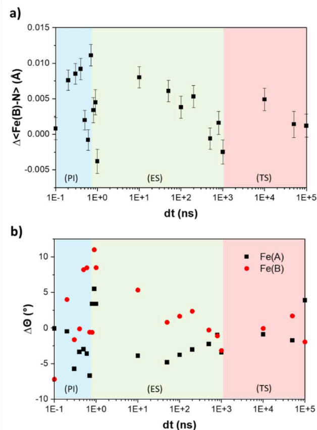
Figure 4 Time-delay dependence of a) \langle\text{Fe(B)-N}\rangle and b) the variation of the trigonal distortion parameter, \Delta\Theta , of both the Fe(A) and Fe(B) ions. Photoinduced (PI), elastic (ES) and thermal (TS) steps are shown in blue, green and red, respectively.
