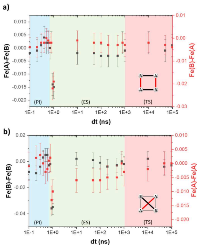
Figure 5 Time dependence of the Fe - Fe distances in FE4 grid: a) Fe(A)-Fe(B) and Fe(B)-Fe(A), and b) Fe(B)-Fe(B) and Fe(A)-Fe(A). Photoinduced (PI), elastic (ES) and thermal (TS) steps are shown in blue, green and red, respectively.
