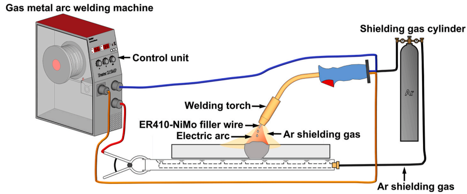
Fig. 1. Schematic of the gas metal arc welding set-up used in this work.
