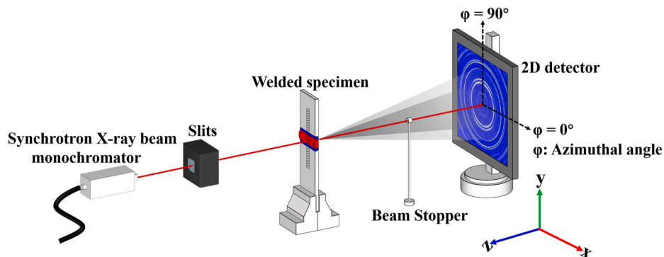
Fig. 3. Synchrotron X-ray diffraction set-up (not to scale).
