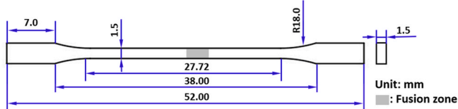
Fig. 2. Geometry and dimensions of specimens used for uniaxial tensile testing.
