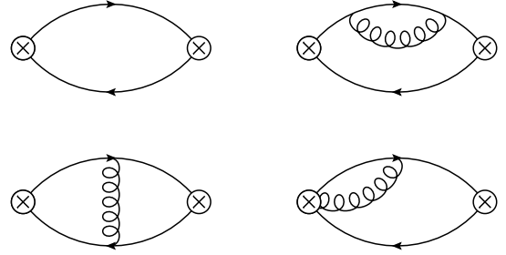
Fig. 1. Feynman diagrams for the calculation of \gamma_{22}^{(2)} .
