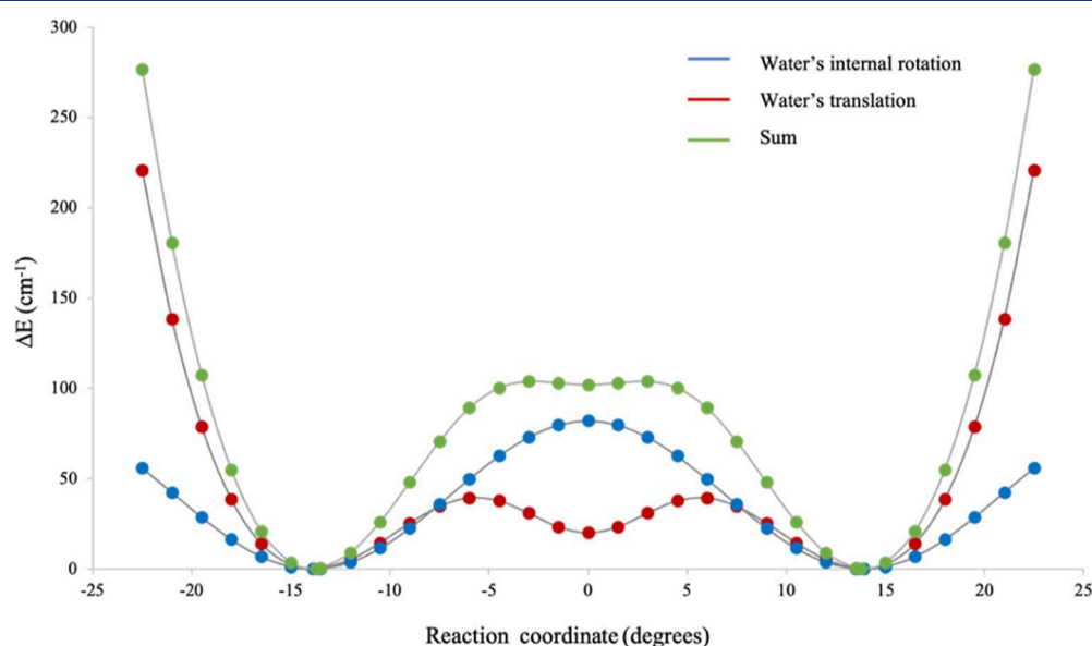
Figure 6. Potential energy curves describing water's translation motion (red), its internal rotation (blue), and the combination of the two motions (green).
