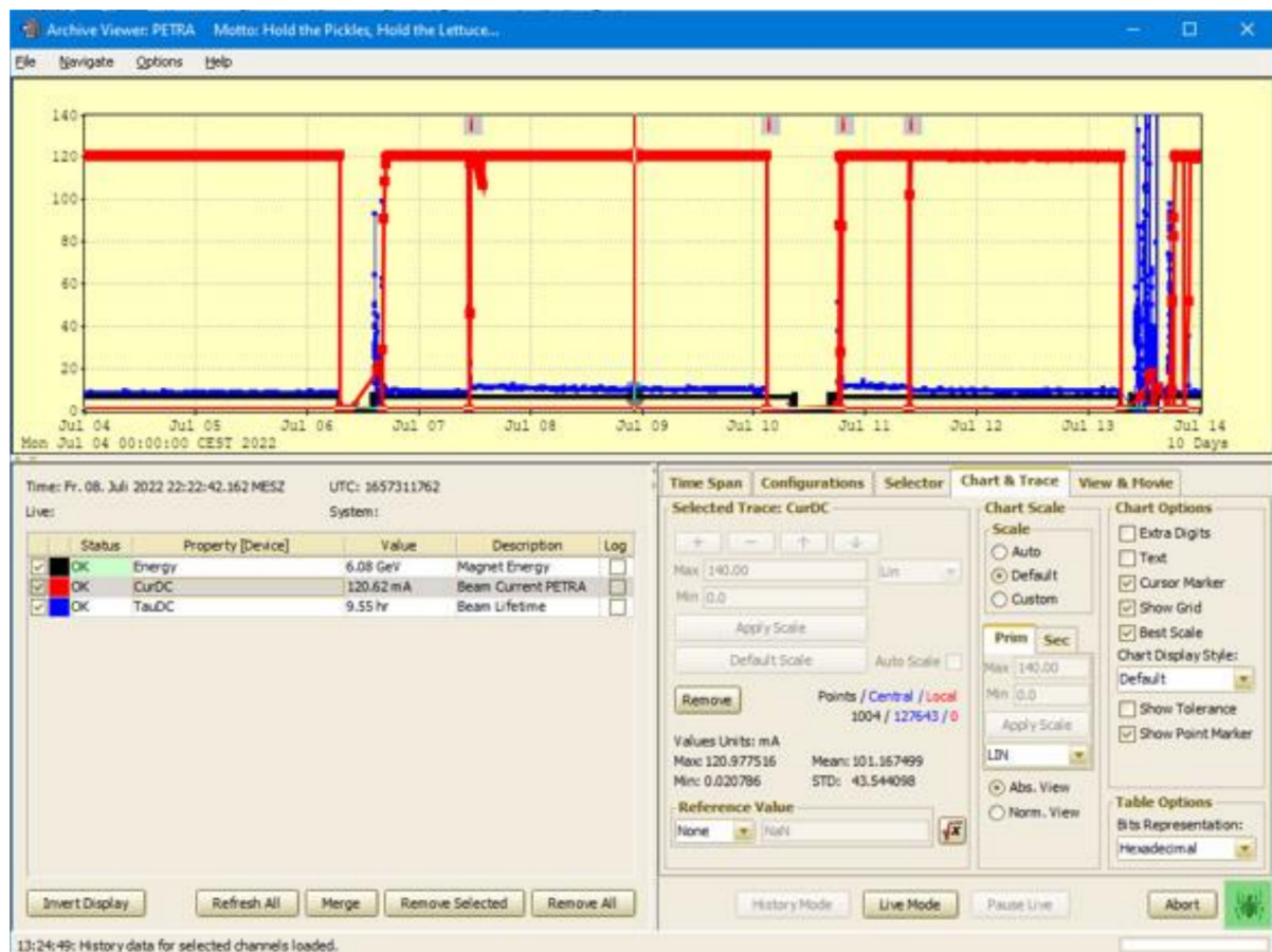
Figure 2: Archive data viewer (PETRAIII).
