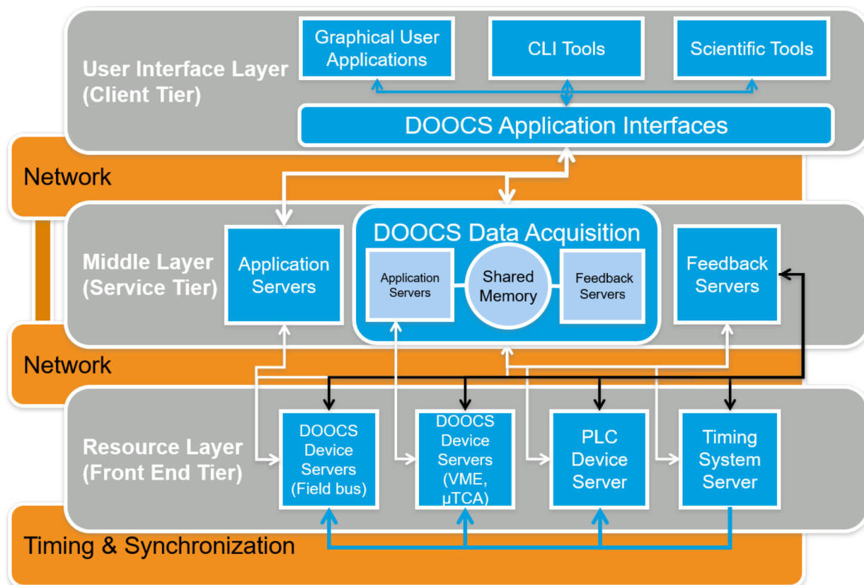
Figure 1: DOOCS control system layout.
