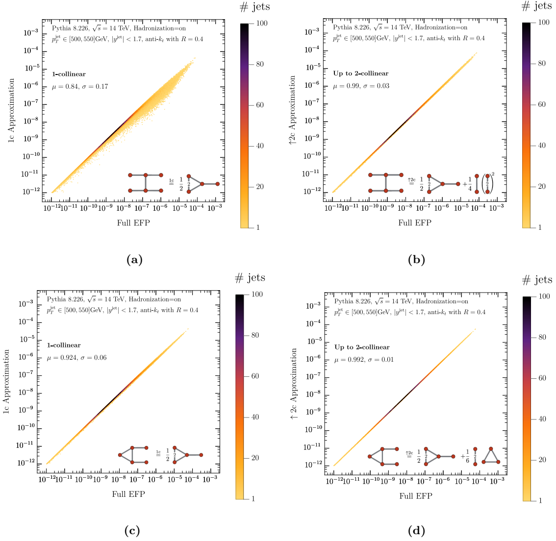
Figure 7. Testing the relationship for the “H” EFP in eq. (2.25) (top row) and “A” EFP in eq. (2.28) (bottom row) in the 1-collinear approximation (left column) and including the 2-collinear approximation (right column), which leads to a substantial improvement. The average \mu and standard deviation \sigma of the ratio is shown.
