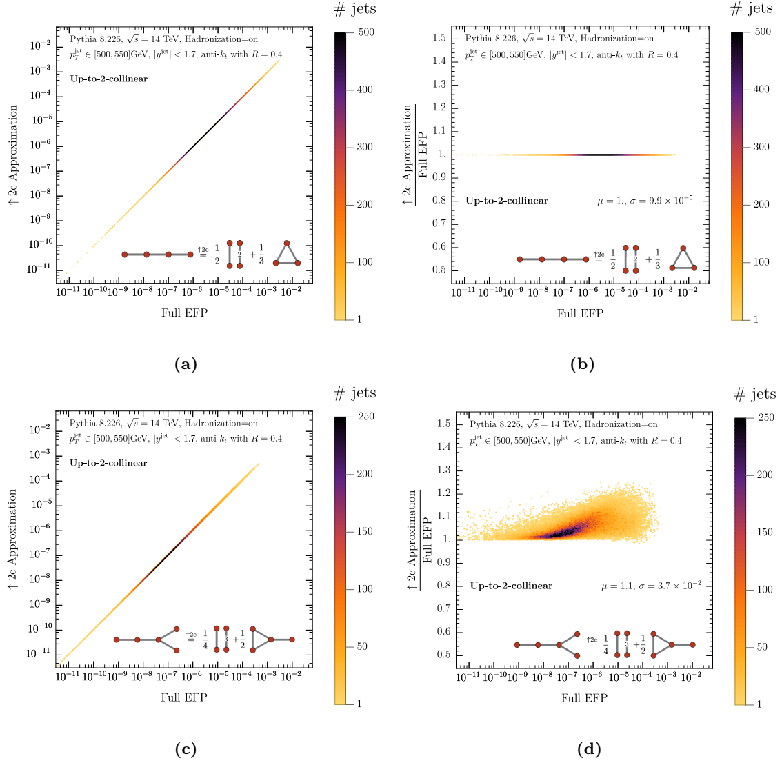
Figure 6. Same as figure 4, but using the relationships obtained from the up-to-2-collinear expansion, which are much more accurate.
