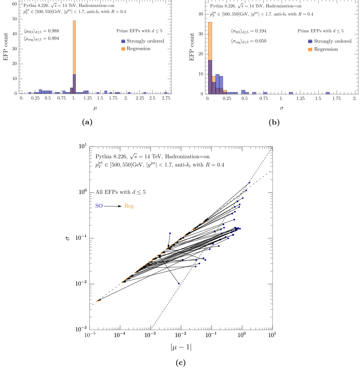
Figure 5. Histogram for the average \mu (a) and standard deviation \sigma (b) of the ratio between prime EFPs up to degree 5 and their expression in terms of SO basis elements. Here, the relationship was found using power counting (blue) and regression (orange). The improvement from using regression is visualized with arrows in the scatter plot (c) for |\mu - 1| and \sigma . The dashed line corresponds to \sigma = |\mu - 1| , and the dotted line corresponds to \sigma^2 = |\mu - 1| .
