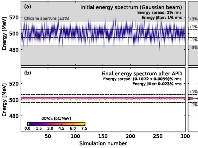
FIG. 3. (a) Initial energy spectrum of 300 Gaussian beams with a 1 % rms energy jitter and energy spread. The gray area represents the energies filtered out by the slit in the chicane. (b) Final energy spectrum after the APD.
