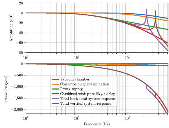
Figure 6: Open-loop transfer function of subsystems.
