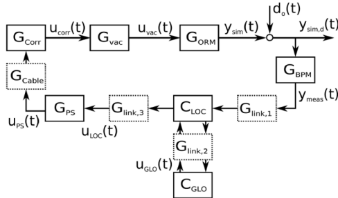
Figure 5: Closed-loop schematic of the FOFB system identifying the individual subsystems.
