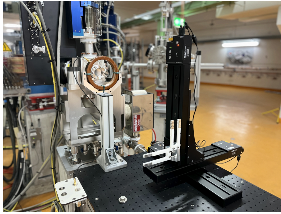
Figure 4: In-air experimental station equipped with ICT (copper ring) and a wirescanner setup on the linear stages. The electrons from the linac are extracted via a 50 \mu\text{m} thick titanium foil.
