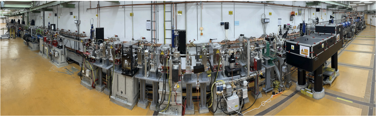
Figure 1: Fisheye-view of the ARES linac. The RF-gun is on the right, followed by two travelling wave structures, the first experimental area, including the optical table for the 2 micron laser is visible in the middle. Further downstream to the left bunch compressor and TDS are installed.
