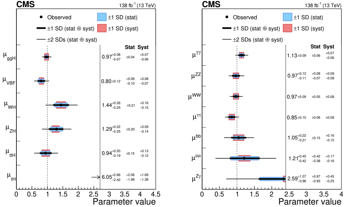
Figure 2: The agreement with the SM predictions for production modes and decay channels. Signal strength parameters extracted for (left) various production modes \mu_i , assuming \mathcal{B}^f = (\mathcal{B}^f)_{SM} , and (right) decay channels \mu^f , assuming \sigma_i = (\sigma_i)_{SM} . The thick (thin) black lines indicate the 1 (2) s.d. confidence intervals, with the systematic and statistical components of the 1 s.d. interval indicated by the red and blue bands, respectively. The vertical dashed line at unity represents the values of \mu_i and \mu^f in the SM. The covariance matrices of the fitted signal strength parameters are shown in Extended Data Fig. B.5. The p -value with respect to the SM prediction are 3.1% and 30.1% for the left and right plot, respectively. The p -value corresponds to the probability that a result deviates as much, or more, from the SM prediction as the observed one.
