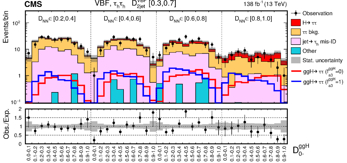
Figure 4: The observed and predicted 2D distribution of (D_0^{ggH}, D_{NN}) before the fit to data in the most sensitive VBF category region with 0.3 < D_{2jet}^{VBF} < 0.7 in the \tau_h\tau_h channel. The total H signal, including VBF, ggH, and VH processes, is shown stacked on top of the background in the solid red histogram. The ggH signal for the CP -even ( CP -odd) scenario is also shown overlaid by the red (blue) line. Only the statistical uncertainties are included in the uncertainty band.
