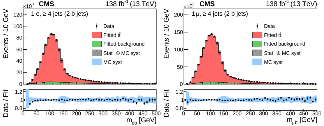
Figure 4: The m_{lb} invariant mass distributions in the electron (left) and muon (right) channels from data (points). The results of the fit to the t\bar{t} and background templates are shown by the red and green histograms, respectively. The vertical bars on the data points in the upper panels indicate the statistical uncertainties in the data and the hatched bands show the combined statistical and systematic uncertainties in the simulation. The lower panels give the ratio of the data to the sum of the fitted MC predictions. The blue bands represent the systematic uncertainties in the expected yield in the simulation for all sources of systematic uncertainty (Section 6).
