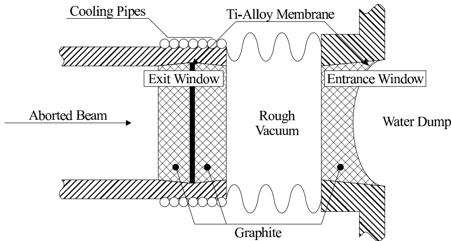
Figure 9.9.2: Concept of (vacuum) exit and (water) entrance window, using a titanium-graphite sandwich design.
