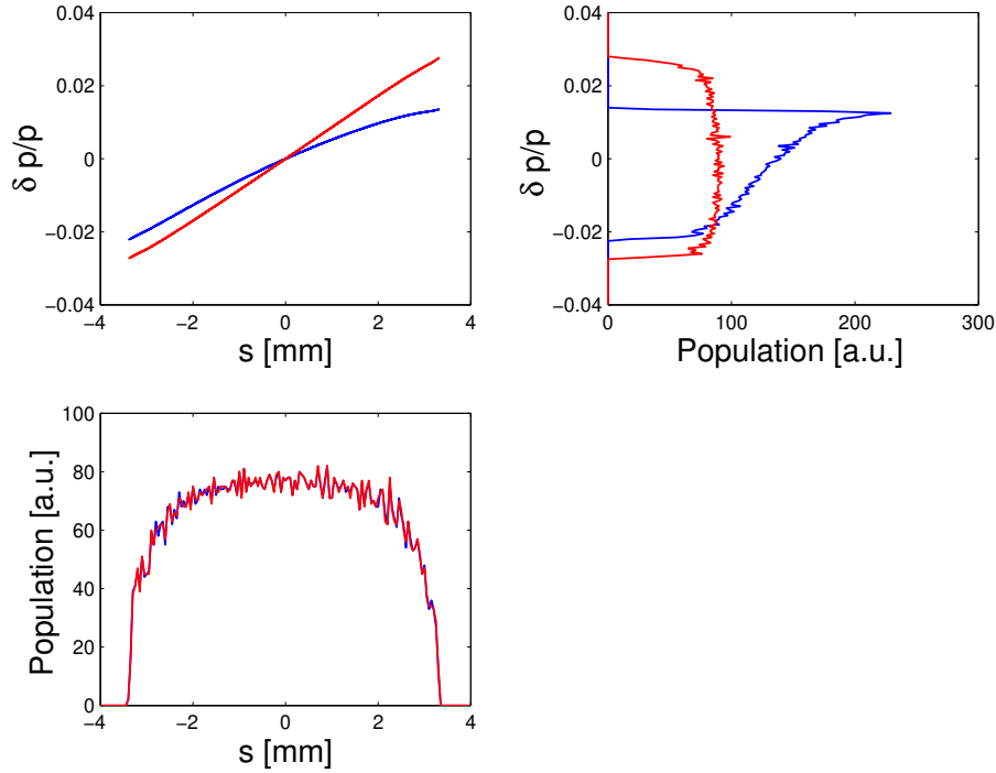
Figure 9.3.4: Longitudinal phase space upstream (blue) and downstream (red) of the third harmonic RF section. The longitudinal phase space distribution is linearised by the combined action of the first and third harmonic RF. The remaining curvature is matched to the second order compression factor of the bunch compressor.
