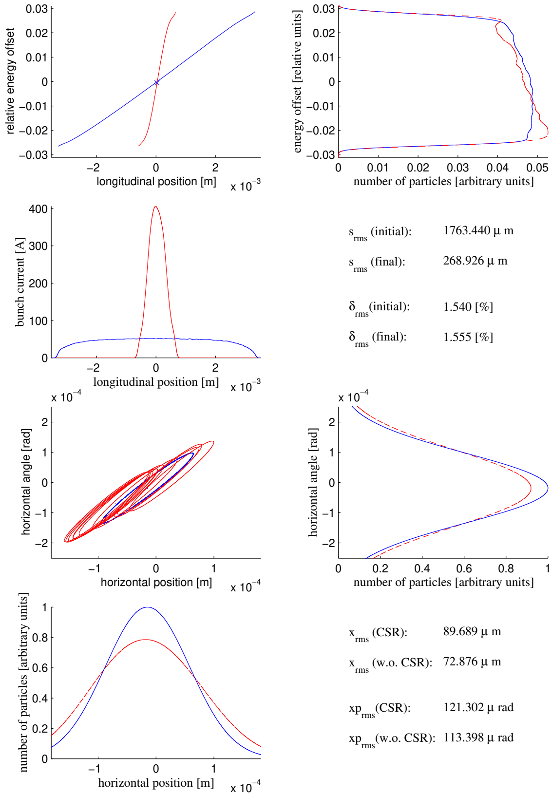
Figure 9.4.6: Longitudinal phase space before (blue) and after (red) Bunch Compressor 1 and transverse phase space at the compressor exit without (blue) and with (red) CSR, respectively.
