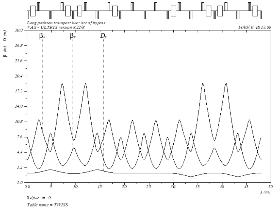
Figure 4.4.7: Optical functions along one bypass arc.
