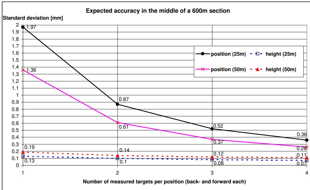
Figure 8.6.2: Expected accuracy in the middle of a 600 m long section versus number of measured targets.
