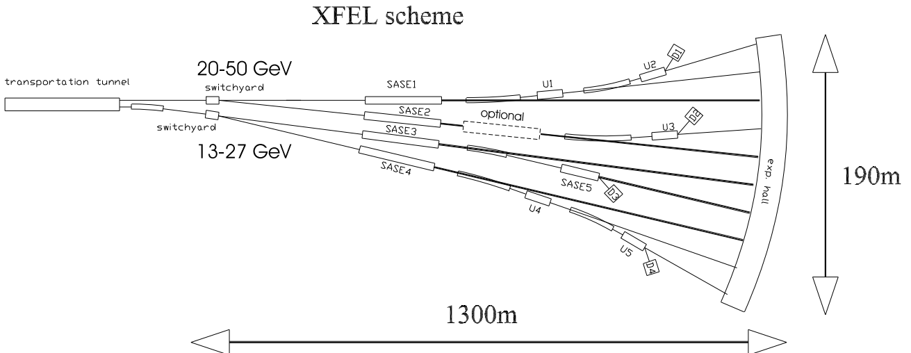
Figure 9.1.4: Beam switchyard distributing two electron beam lines of different energies to various undulators. SASE1 through SASE5 are FEL undulators while U1 through U5 are undulators for spontaneous radiation. The scheme sketched can be extended to serve many more undulators. It displays also the long drift lines necessary for the photon beams.
