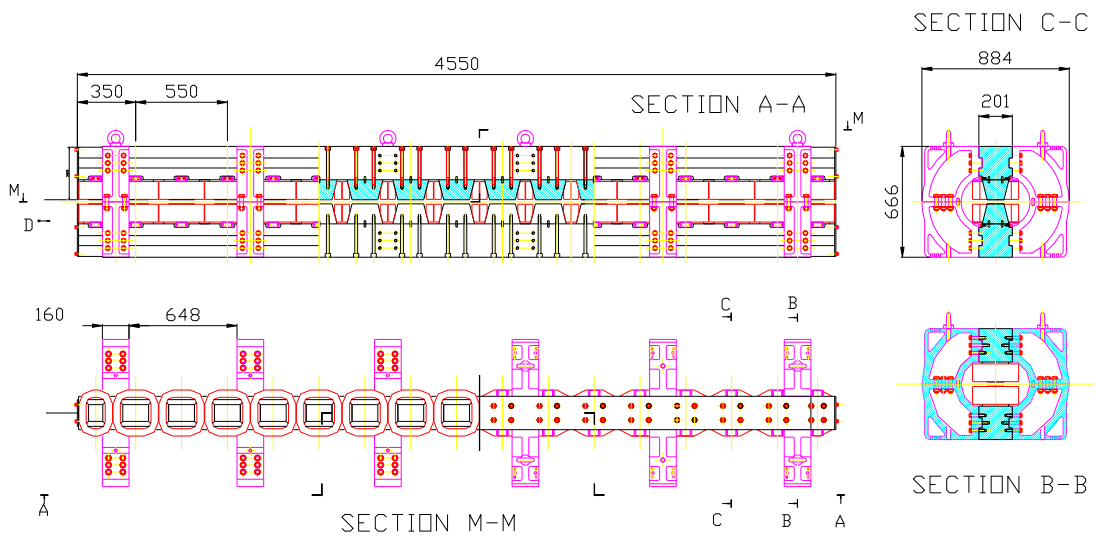
Figure 5.6.4: Electromagnetic wiggler.
