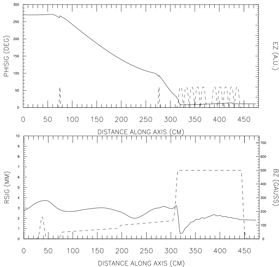
Figure 4.2.3: RMS beam radius and bunch length variation along the prebunching and bunching sections. The axial electric field (top) and the magnetic focusing field (bottom) are shown.
