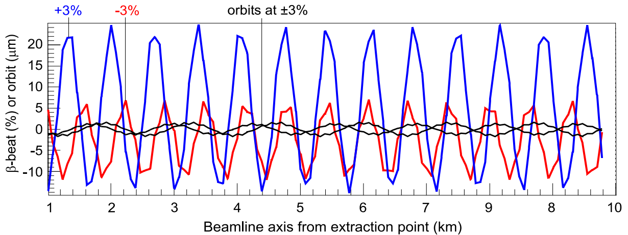
Figure 9.6.2: Chromatic beta beat \Delta\beta/\beta in % of the vertical beta function at 30 GeV for \Delta p/p = +3\% (blue) and -3\% (red) in the 12 km transfer line. The 2 curves of smaller amplitude (black) show examples of not perfectly corrected chromatic orbits at \Delta p/p = \pm 3\% (in \mu\text{m} ). Beta functions and orbits both have a chromatic phase dependency. The horizontal beta function (not shown) reaches 8% beat.
