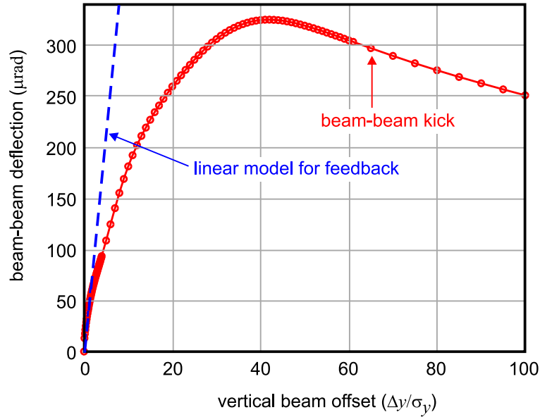
Figure 7.3.2: The beam-beam kick as a function of the relative offset for the nominal 250 GeV beam parameters (calculated using GUINEA-PIG[18]). The linear feedback model is also indicated.
