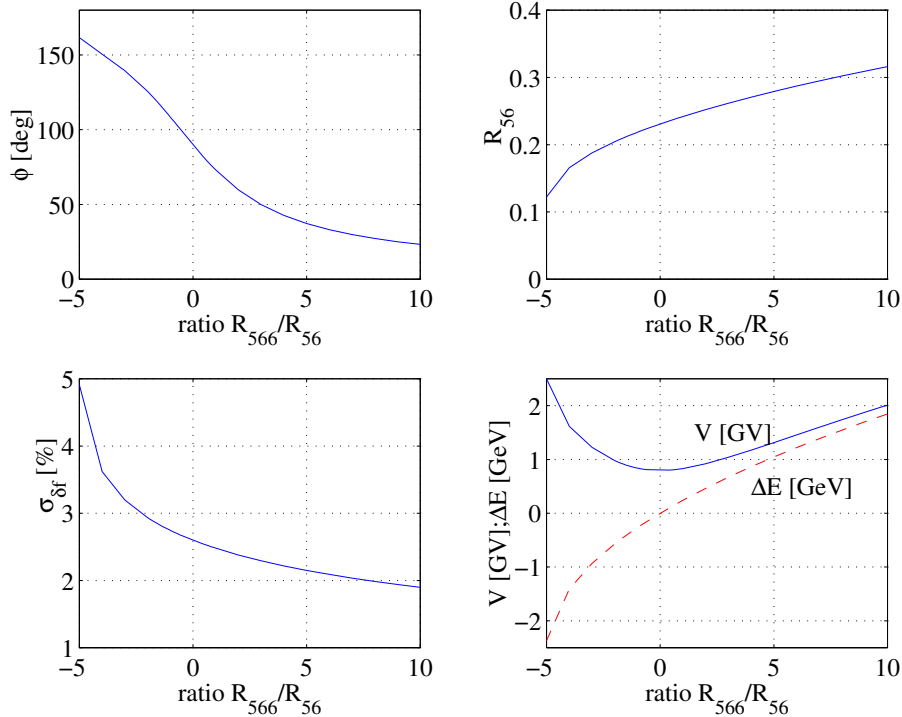
Figure 6.2.2: Accelerating phase (upper left), longitudinal dispersion R_{56} (upper right), final energy spread (lower left), and effective accelerating voltage (lower right) as a function of r = T_{566}/R_{56} . The final bunch length is 300 \mu\text{m} .
