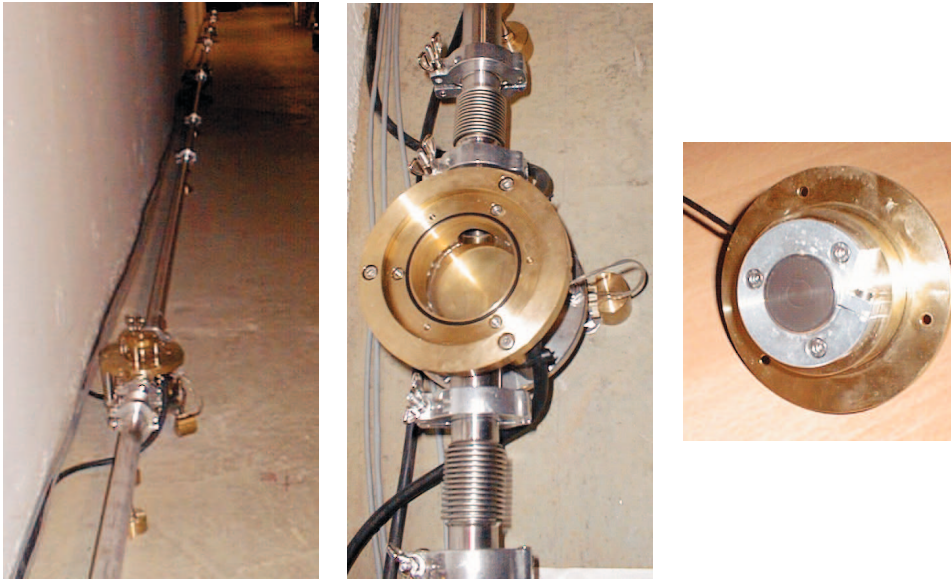
Figure 8.6.3: Test installation (42m section) of a hydrostatic levelling system.
