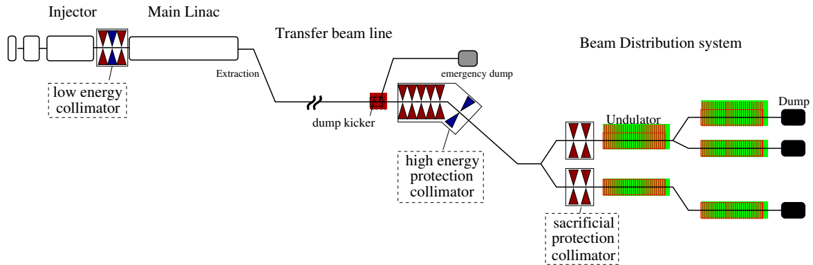
Figure 9.1.8: Schematic layout of the FEL collimator and protection system.
