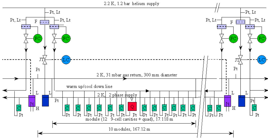
Figure 8.7.3: Cryogenic string.
