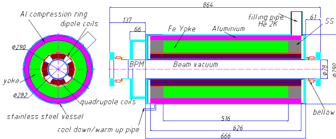
Figure 3.3.3: Cross-section and longitudinal cut of superconducting magnet package.
