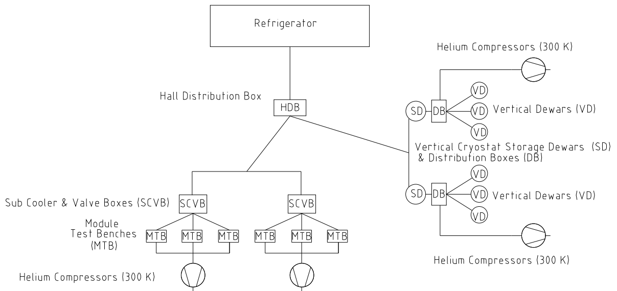
Figure 8.8.2: Block Diagram of the Cryogenic System.
