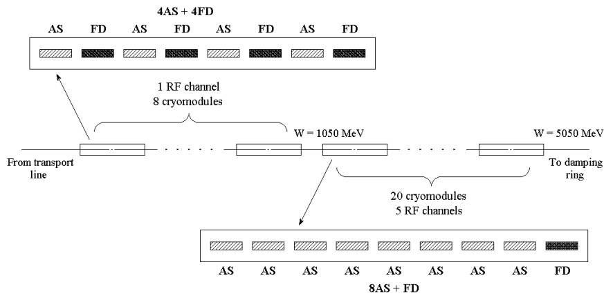
Figure 4.4.8: Conceptual layout of the sc positron injector linac (AS = accelerating structure, FD = quadrupole doublet).
