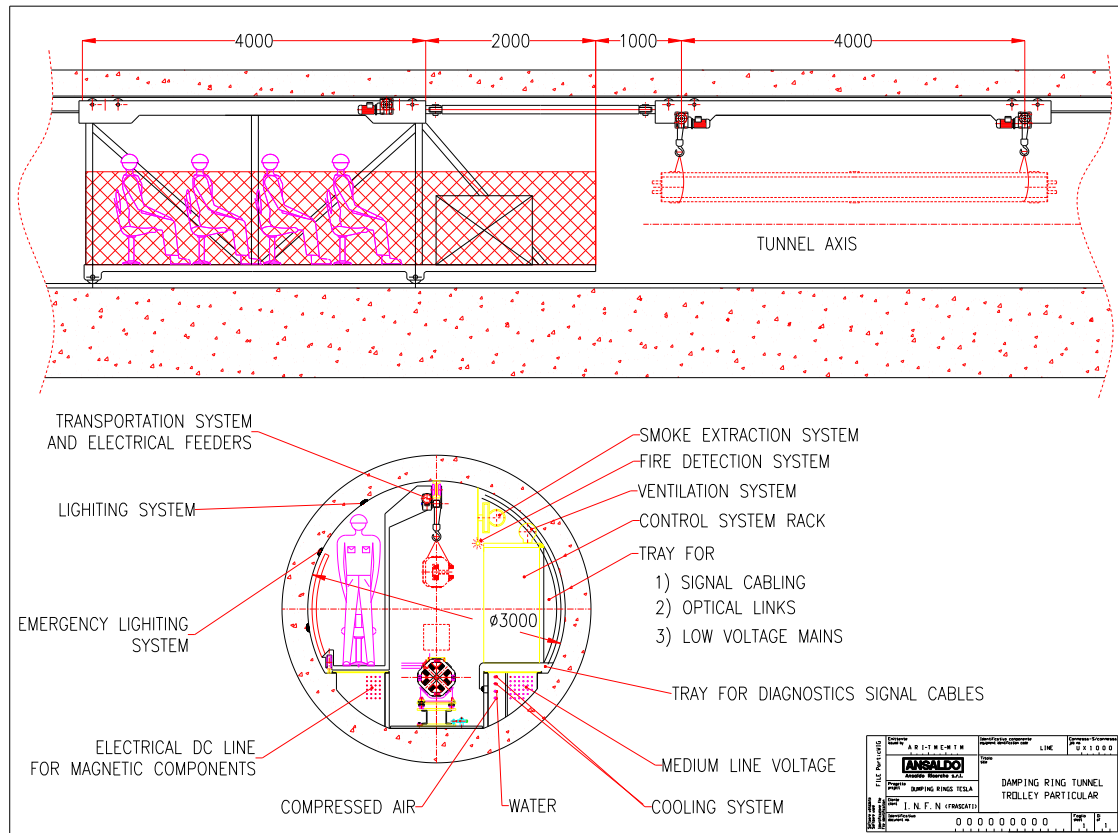
Figure 5.6.10: Arc tunnel cross section.
