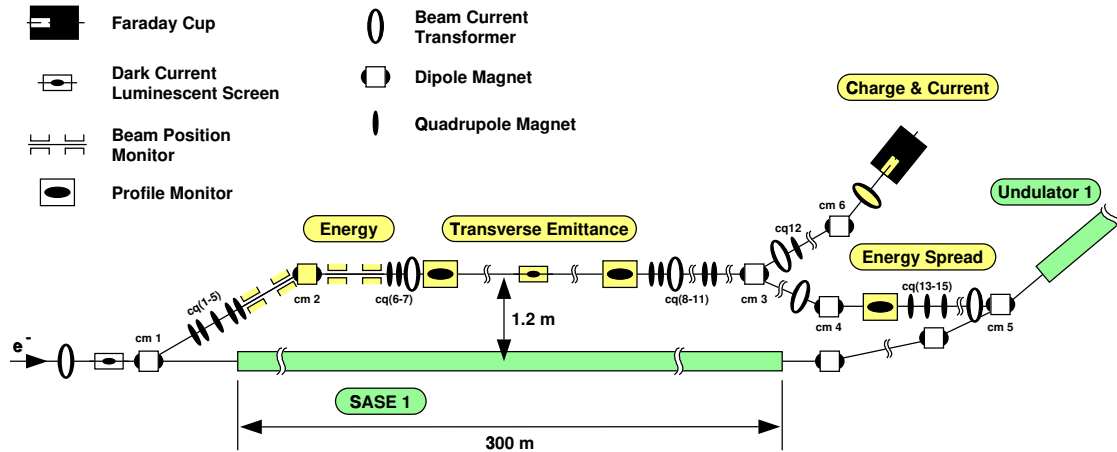
Figure 9.6.9: The layout of the Diagnostic Commissioning line (DCL).
