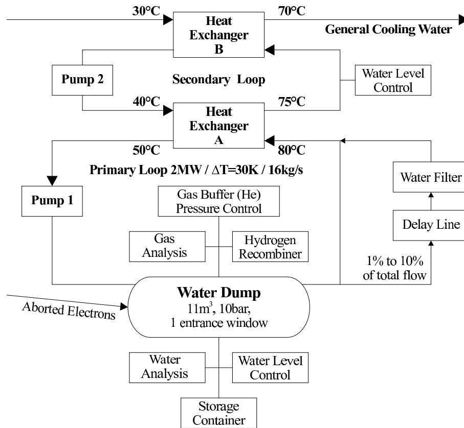
Figure 9.9.3: Schematic overview of the water system required for each of the four FEL electron beam dumps.
