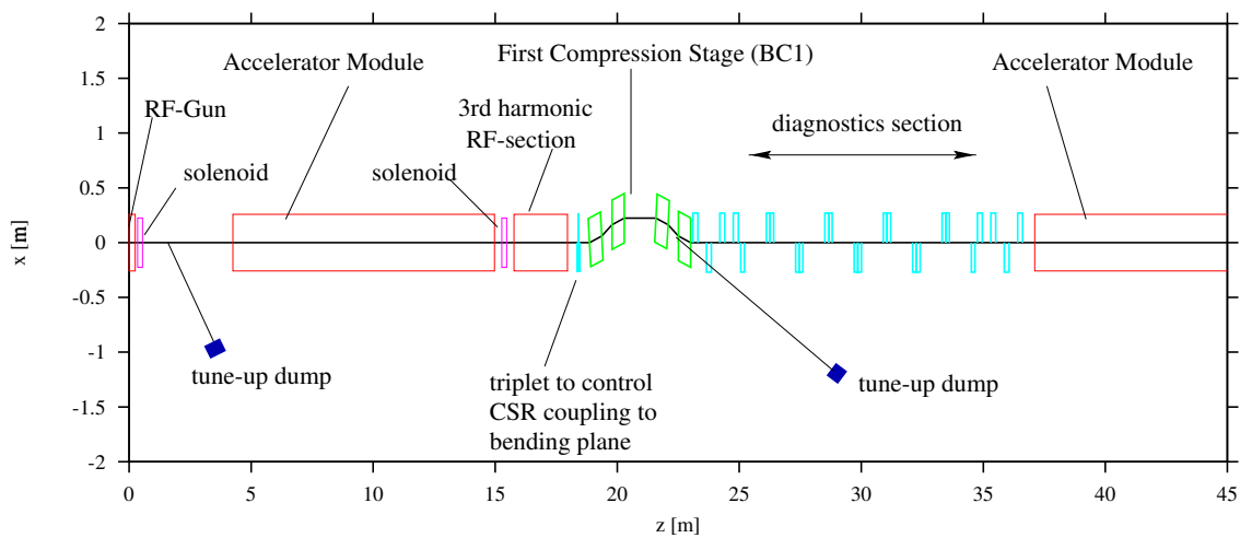
Figure 9.3.1: Schematic layout of the FEL injector.
