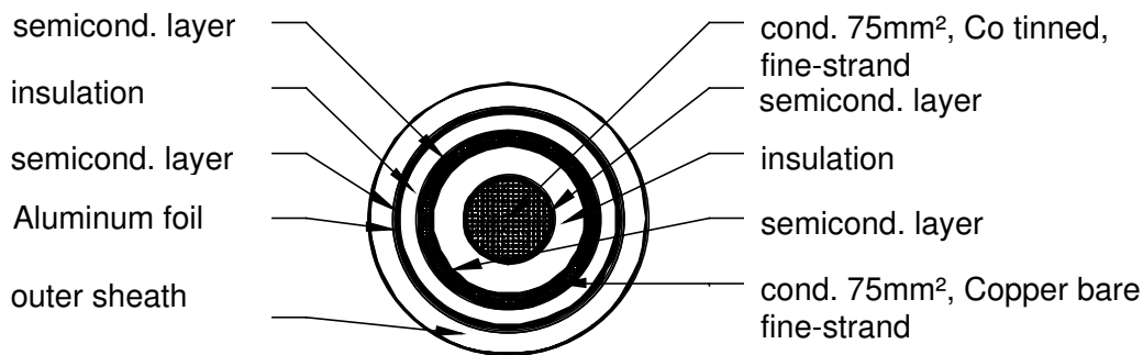
Figure 3.4.4: Construction of the pulse cable.
