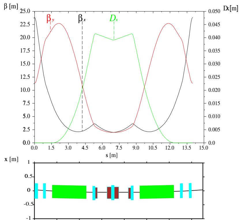
Figure 6.4.1: Optical functions and floor plan of one achromatic arc cell. Dipoles are green, quadrupoles blue and sextupole magnets are brown.
