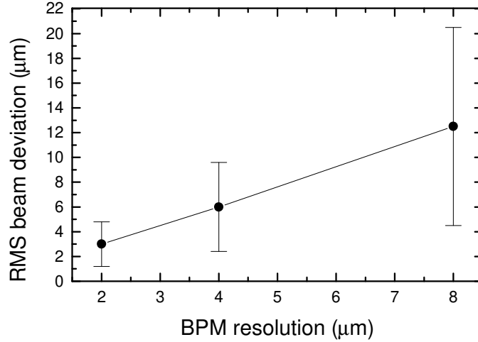
Figure 9.8.4: RMS value of the electron beam orbit deviation after beam based alignment along a 300 m long undulator for different values of the BPM resolution. Initial quadrupole offsets are within \pm 200 \mu\text{m} . Beam based alignment has been performed for 1000 samples of random quadrupole offsets for each BPM resolution.
