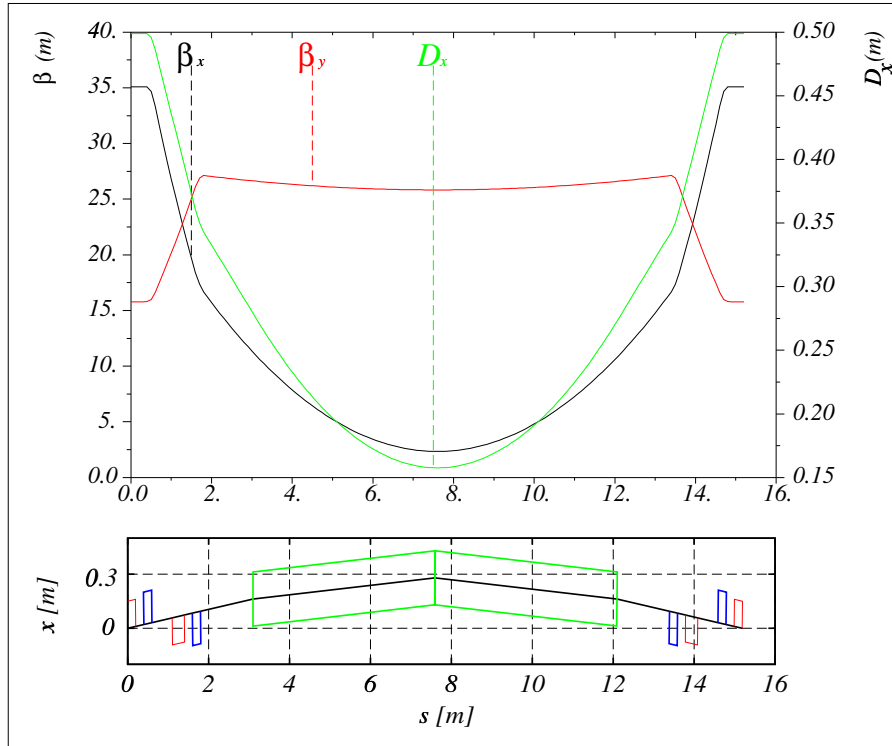
Figure 5.2.1: Upper plot: horizontal (black), vertical (red) \beta -functions and horizontal dispersion (green). Lower plot: arc cell geometry showing the location of dipoles (green), quadrupoles (blue) and sextupoles (red).
