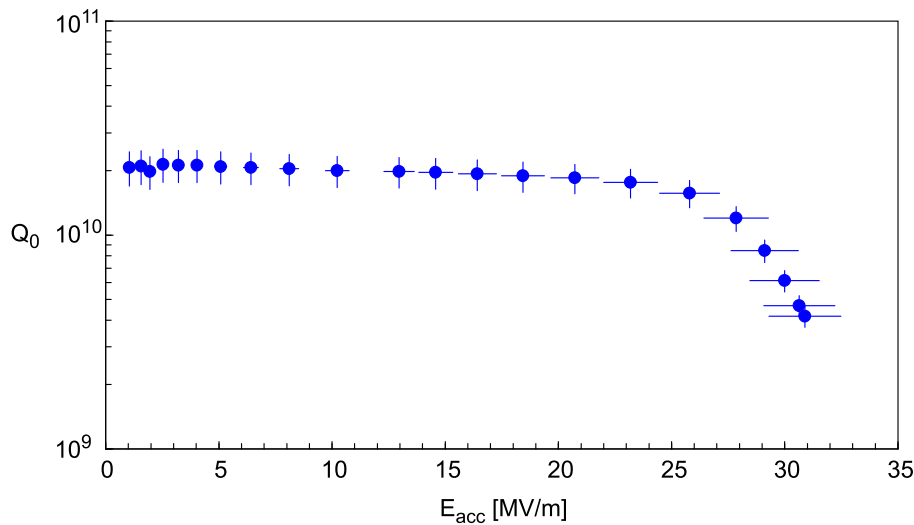
Figure 2.1.5: Excitation curve of a high-performance 9-cell cavity. The cavity was cooled by superfluid helium of 2K. The systematic rms errors in the determination of the accelerating field and the quality factor are indicated.
