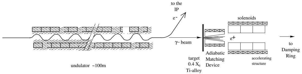
Figure 4.3.1: Sketch of the positron source layout.
