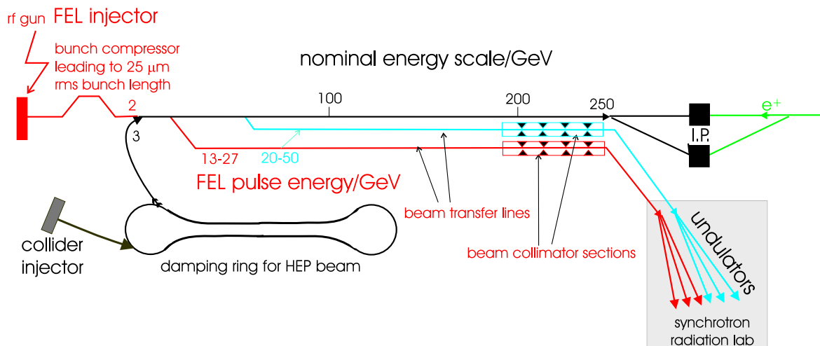
Figure 9.1.3: Sketch of a coherent X-ray source laboratory based on the TESLA linear collider installation. The XFEL electron beam is produced by a dedicated injector followed by a sequence of bunch compressors. The beam can in principle be extracted at any energy between 2 and 250 GeV and is transferred inside the linac tunnel to the X-ray lab located close to the interaction points (I.P.). Multiple extraction lines can be utilised in parallel, so that various beam energies are available in the X-ray lab quasi-simultaneously. In the present design, two beam lines with electron energies up to 50 GeV are foreseen.
