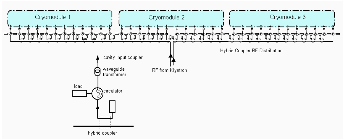
Figure 3.4.5: RF waveguide distribution of one RF station.
