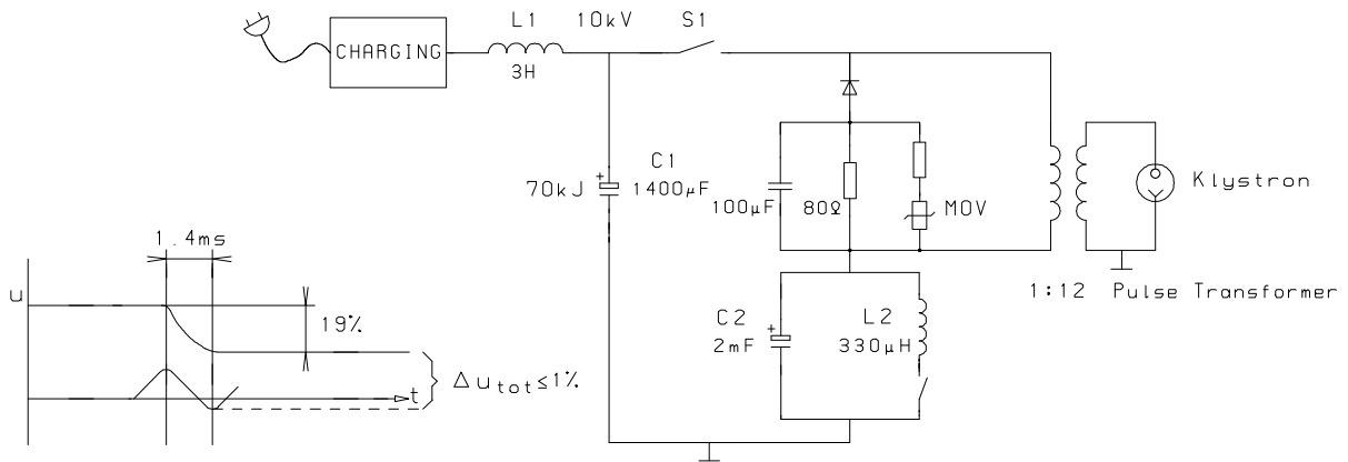
Figure 3.4.3: Modulator circuit (conceptual).
