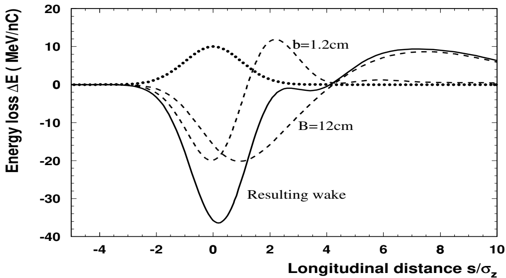
Figure 9.7.1: Longitudinal resistive wake potentials of the FEL beam in the transfer line ( \sigma_z = 25 \mu\text{m} ). Shown are the wakes in the small pipe ( b = 1.2 \text{ cm} ), the large pipe ( B = 12 \text{ cm} ) and the resulting induced wake potential. The dotted line indicated the longitudinal Gaussian bunch profile. The bunch tail is to the right.
