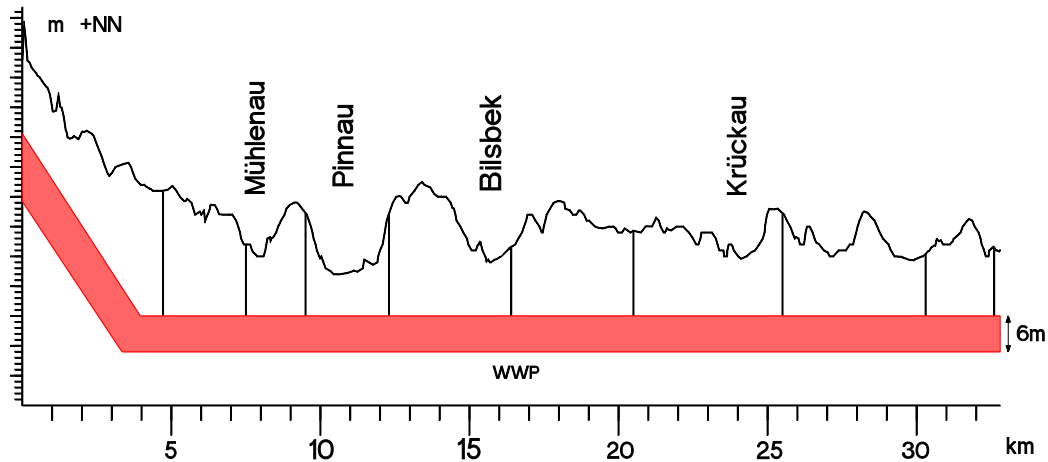
Figure 8.2.3: Elevation of the linac tunnel.
