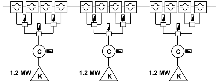
Figure 5.4.1: Damping ring RF system based on single cell SC cavities.
