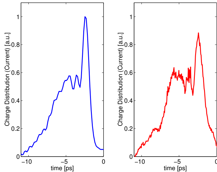
Figure 9.2.4: Longitudinal profile of the electron bunches as measured with two different methods. Left: A measurement using the coherent transition radiation interferometry method. Right: Projection of the longitudinal phase-space reconstructed by means of the tomography method. Both measurements were taken with a few days separation.
