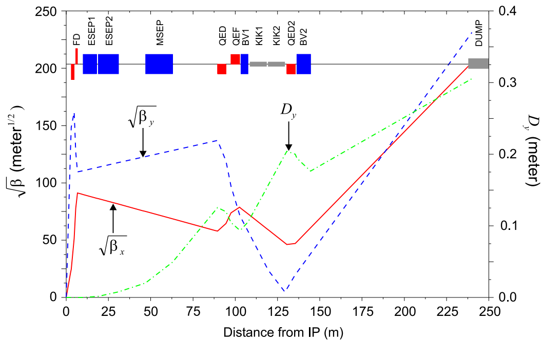
Figure 7.6.2: Optics of the charge particle extraction line.
