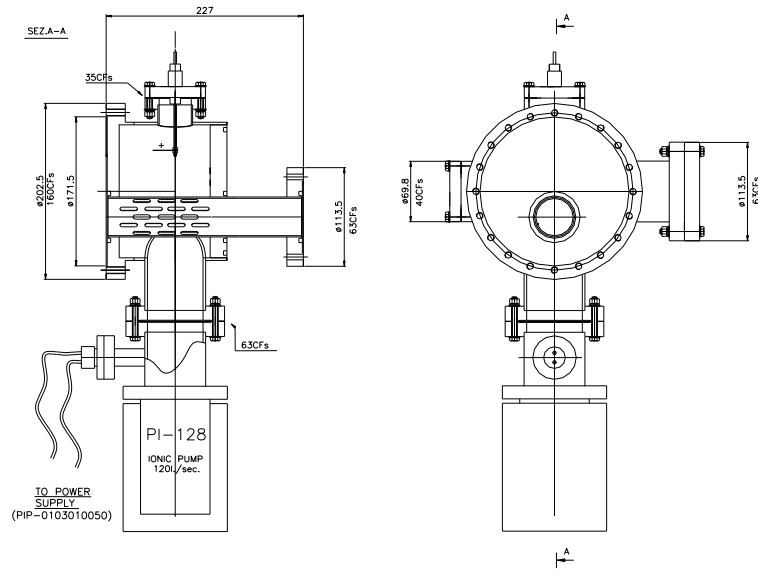
Figure 5.6.8: Typical pumping station.
