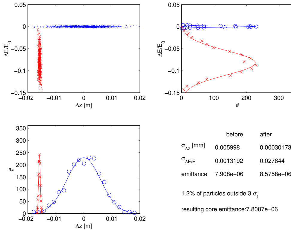
Figure 6.2.3: Longitudinal phase space before (blue) and after (red) the bunch compressor.
