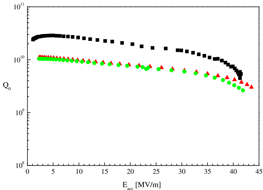
Figure 2.1.14: Excitation curves of three electropolished single-cell cavities without heat treatment at 1400°C. The tests have been performed in different cryostats and under slightly different conditions (magnetic shielding, helium temperature).
