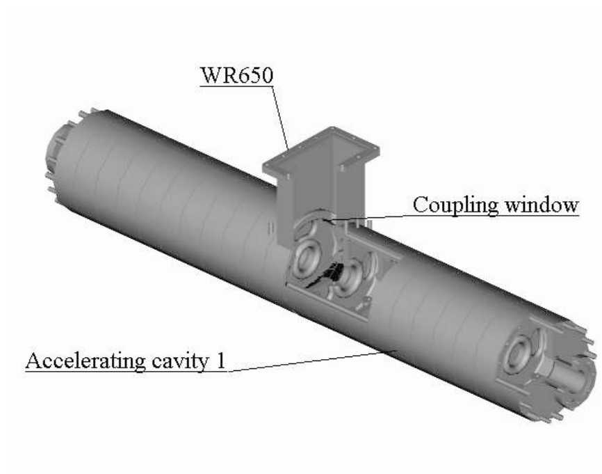
Figure 4.4.2: Short accelerating cavity for the first part of the PPA.
