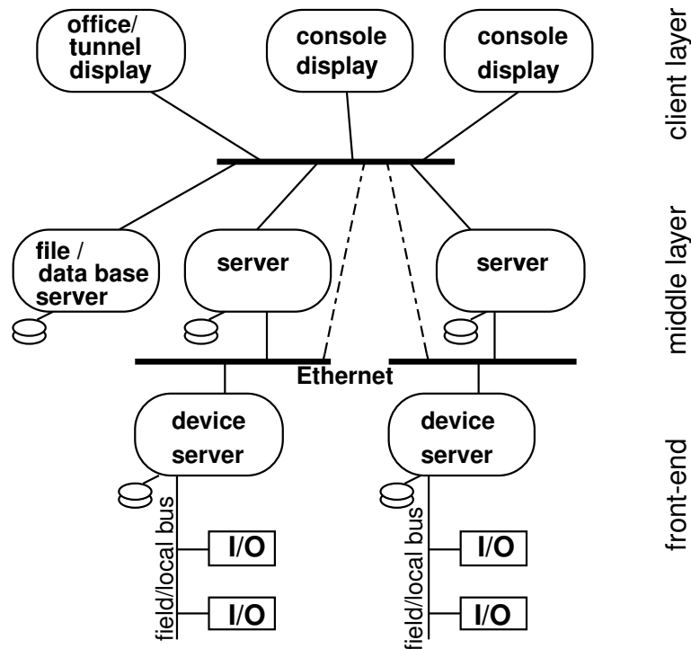
Figure 8.9.1: Sketch of the control system layers.
