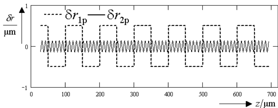
Figure 9.7.5: Periodic approximations \delta r_{1p} and \delta r_{2p} of the slowly and rapidly varying contributions to the surface function.
