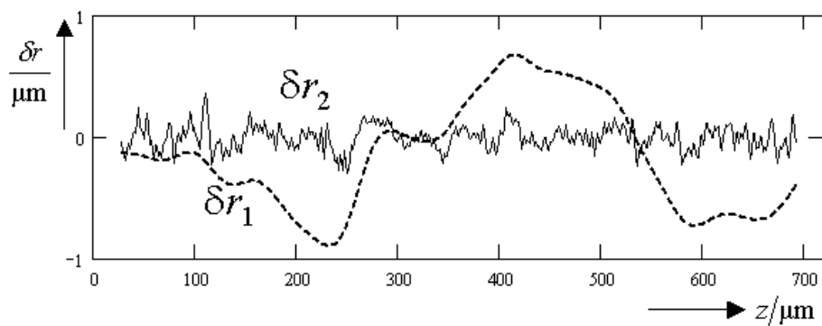
Figure 9.7.4: The slowly and rapidly varying contributions \delta r_1 and \delta r_2 .
