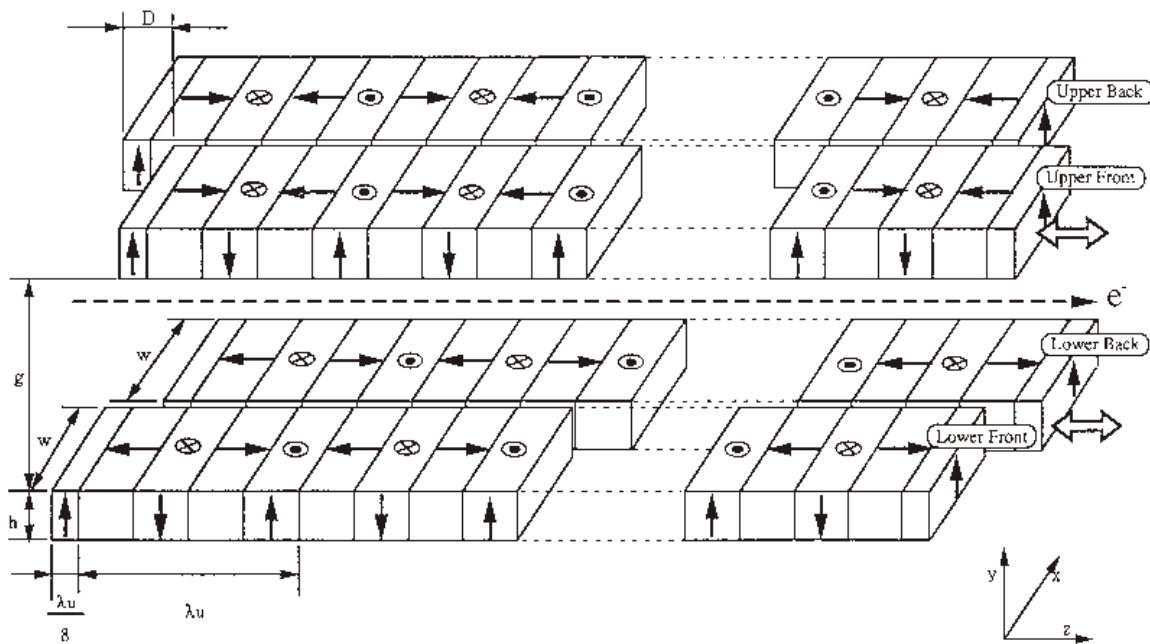
Figure 9.8.3: Magnetic design principle of a Sasaki type undulator, a planar helical structure providing adjustable polarization.
