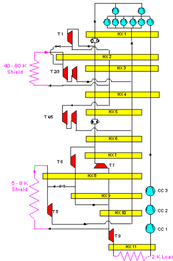
Figure 8.7.4: Flow diagram of model refrigerator.
