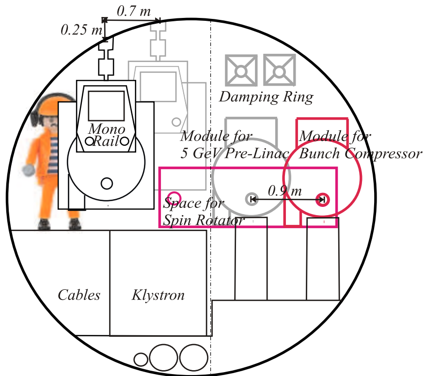
Figure 6.5.2: Cross-section of the TESLA tunnel in the electron damping ring injection/ejection region, looking upstream towards the injector. The RF modules of the two beam lines are interleaved (see figure 6.5.1).
