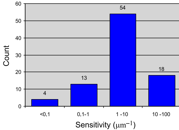
Figure 7.3.4: Summary of quadrupole sensitivity calculations. The sensitivity ( \mu\text{m}^{-1} ) is calculated as the inverse of the vertical quadrupole motion required to increase \sigma_y^* by 2%.
