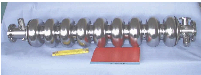
Figure 1.1.1: The 9-cell niobium cavity for TESLA.
