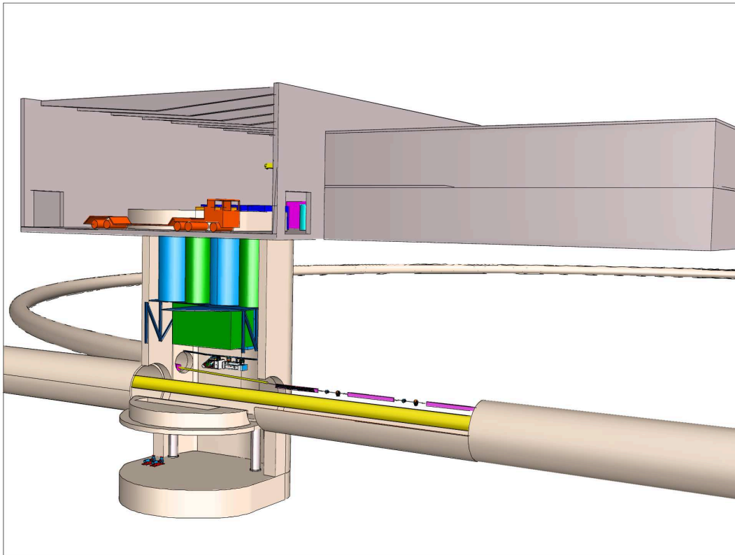
Figure 8.2.4: Access shaft and damping ring tunnel.
