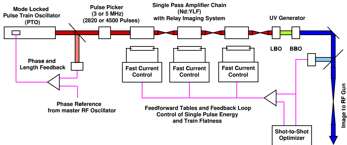
Figure 4.2.2: Schematic of the laser system for the unpolarised RF gun source.
