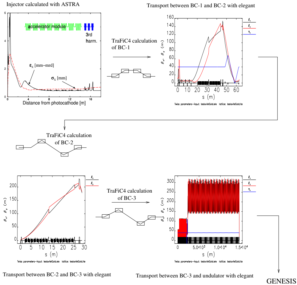
Figure 9.4.5: Complete beam dynamics simulation for TESLA XFEL.
