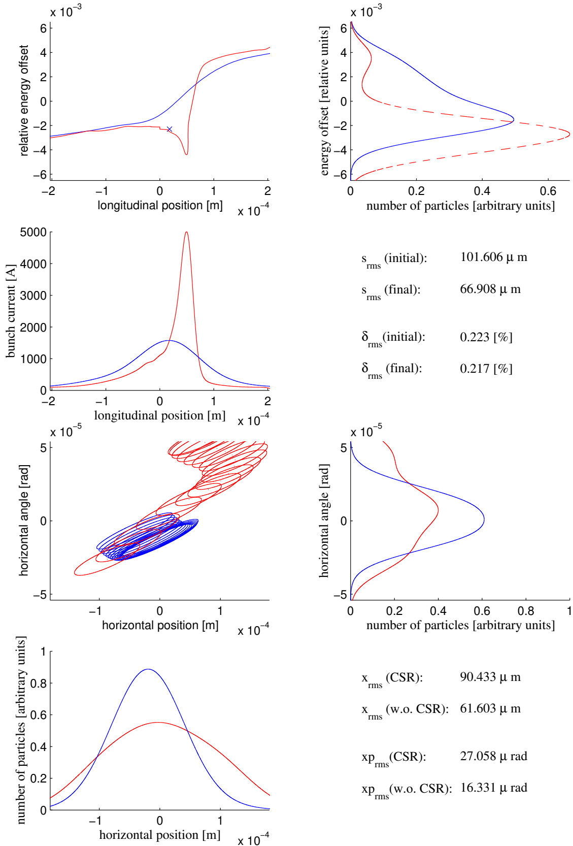
Figure 9.4.8: Longitudinal phase space before (blue) and after (red) Bunch Compressor 3 and transverse phase space at the compressor exit without (blue) and with (red) CSR, respectively.
