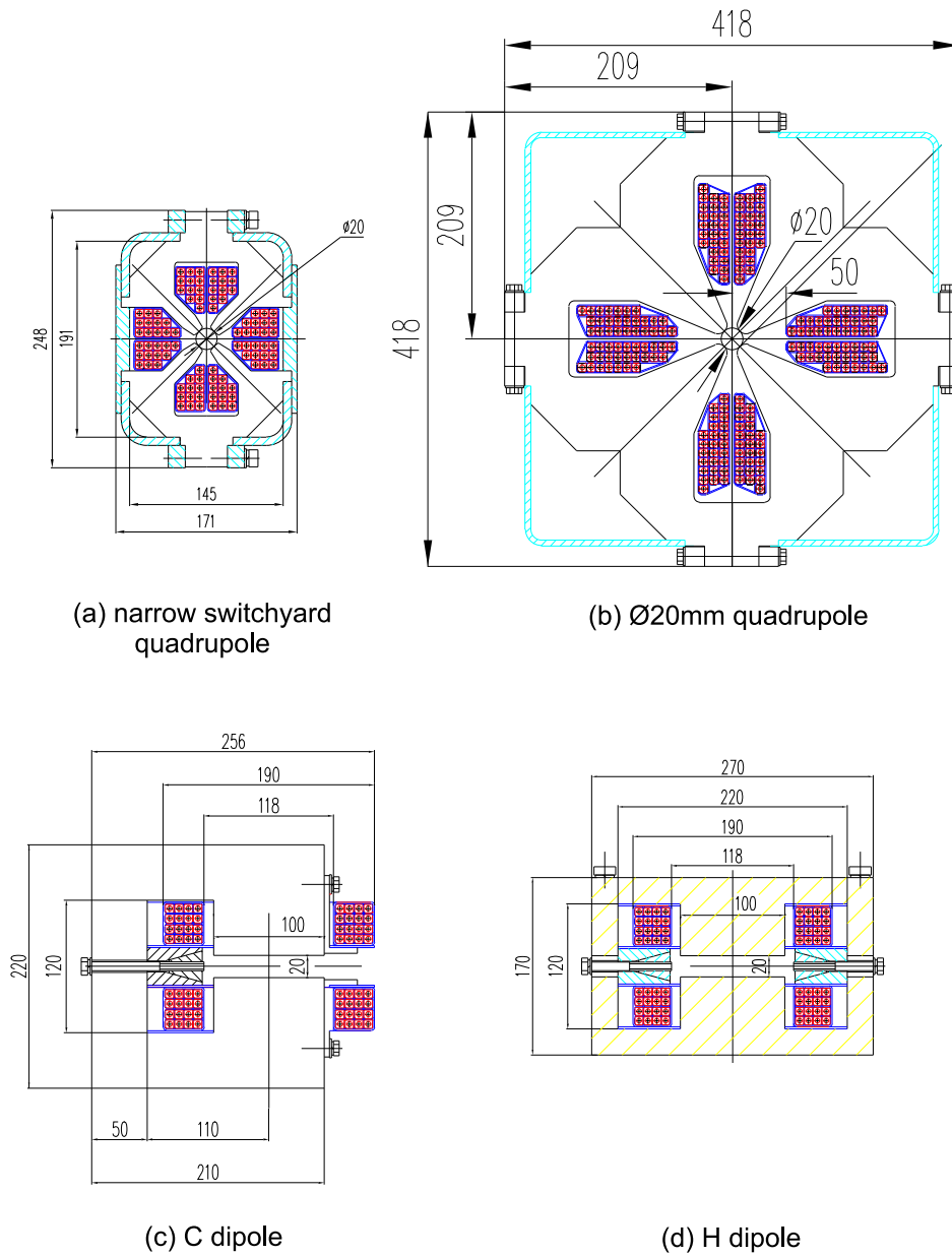
Figure 7.2.8: Cross-sections of four of the BDS magnets (taken from [11]): (a) Special narrow quadrupole used in the switchyard arcs (20 mm) (section 7.2.2); (b) standard 20 mm quadrupole; (c) C dipole (20 mm); (d) H dipole (20 mm). Dimensions are in mm.
