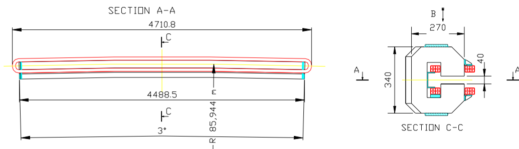
Figure 5.6.1: Bending magnet.
