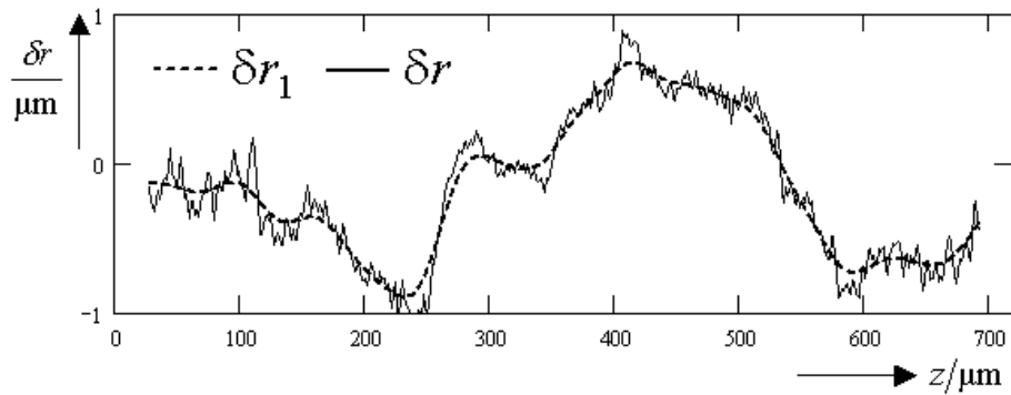
Figure 9.7.3: Measured surface function \delta r and the slowly varying contribution \delta r_1 .
