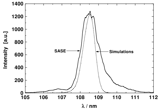
Figure 9.2.2: Typical wavelength spectrum of the central SASE FEL radiation cone (collimation angle \pm 0.2 mrad), taken at the TESLA Test Facility. The dotted line is the result of numerical simulations. The bunch charge is 1 nC. The larger width of the measured spectrum is consistent with the energy spread of the beam.
