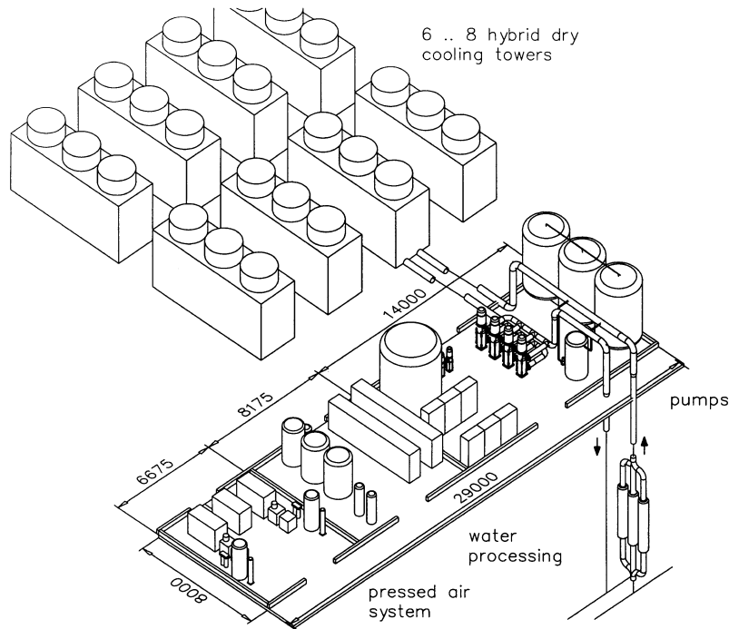
Figure 8.5.1: Sketch of the cooling station for one service hall.
