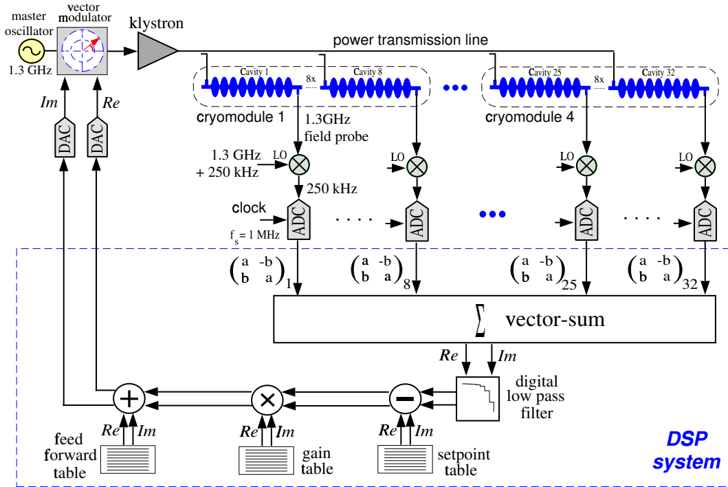
Figure 3.4.7: Schematic of the digital RF feedback system.
