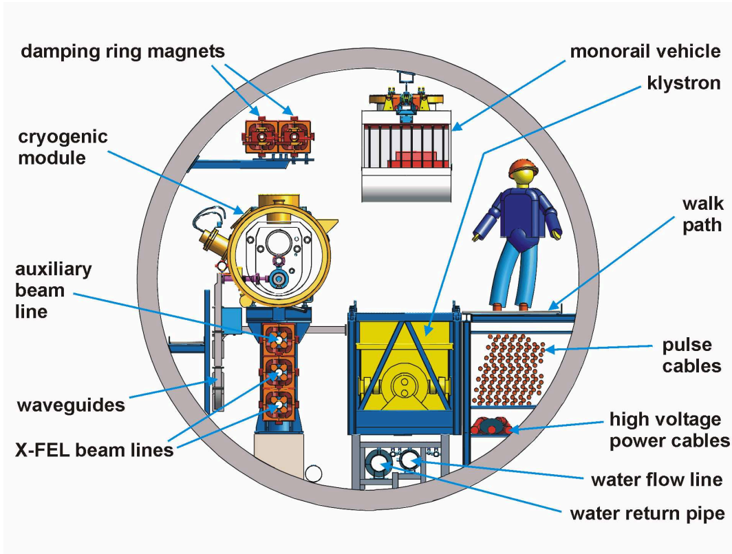
Figure 8.2.7: Cross-section of the TESLA tunnel.
