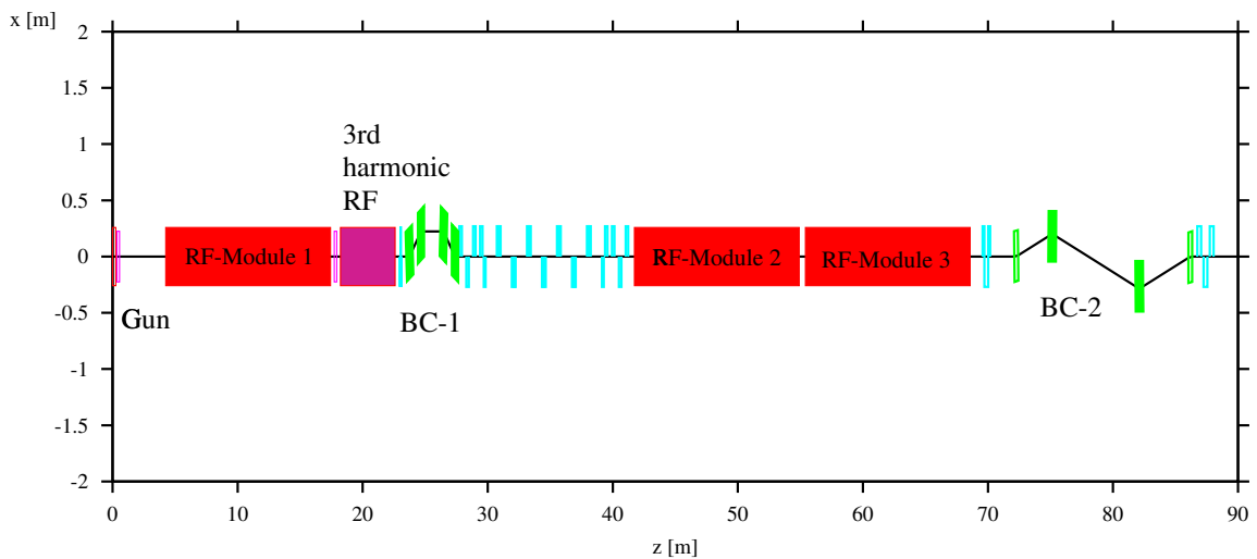
Figure 9.4.3: Floor plan of the 500 MeV XFEL pre-injection linac with the first two bunch compression stages.
