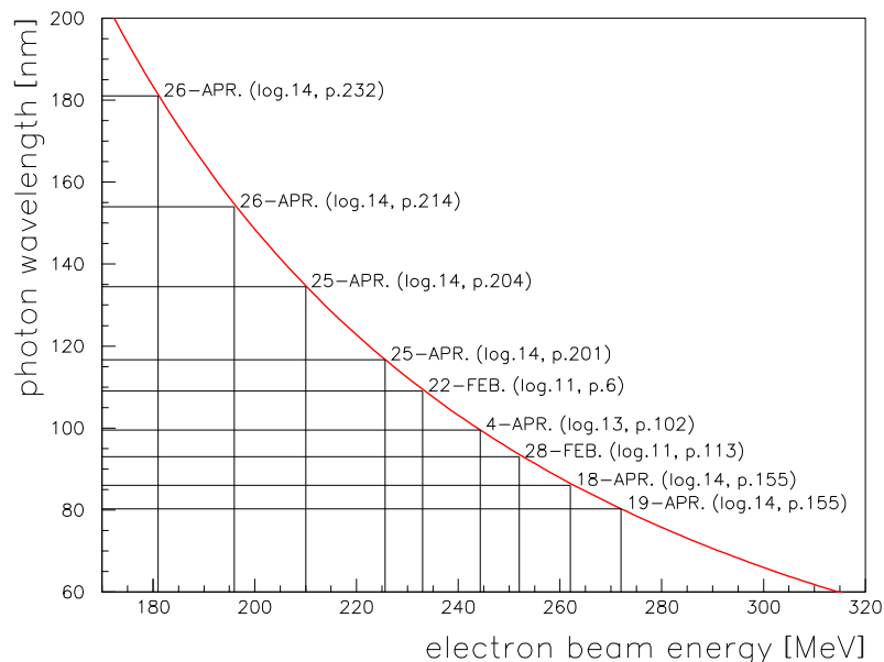
Figure 9.2.1: SASE FEL wavelengths obtained at TTF FEL versus electron beam energy. The red curve is the prediction according to eq. 9.1.1.
