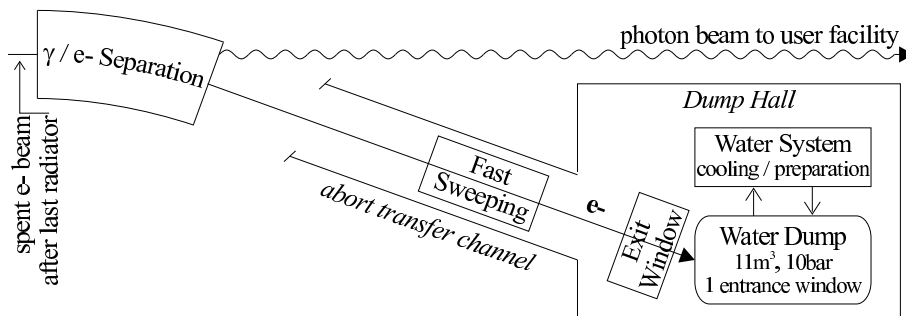
Figure 9.9.1: Schematic view of the beam dump system for the electron beams at the FEL facility.
