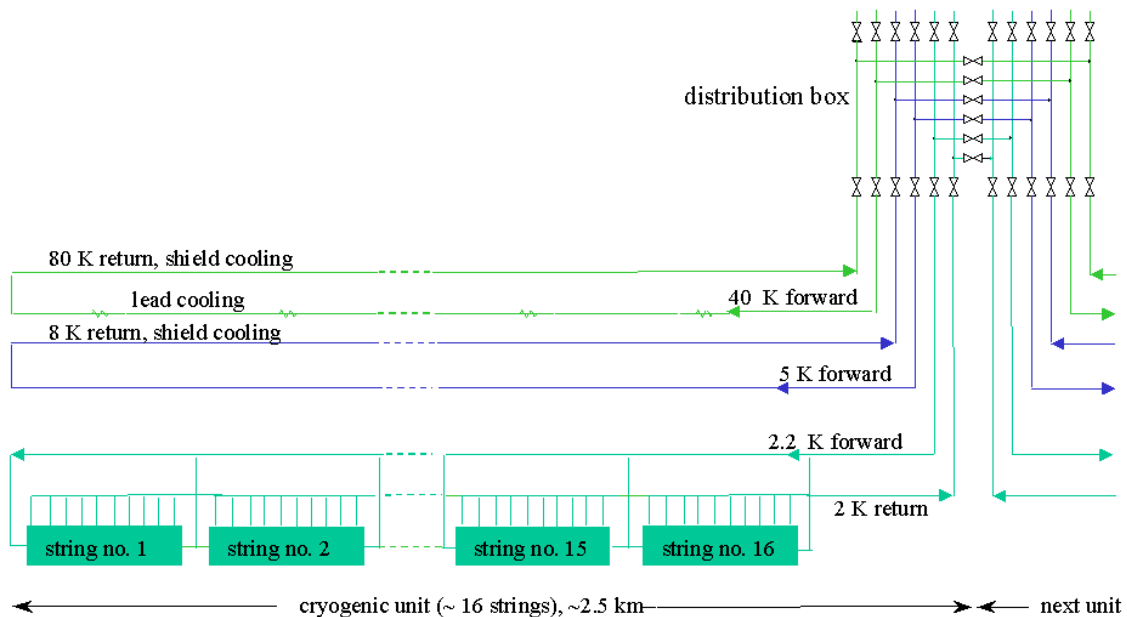
Figure 8.7.2: Cryogenic unit.
