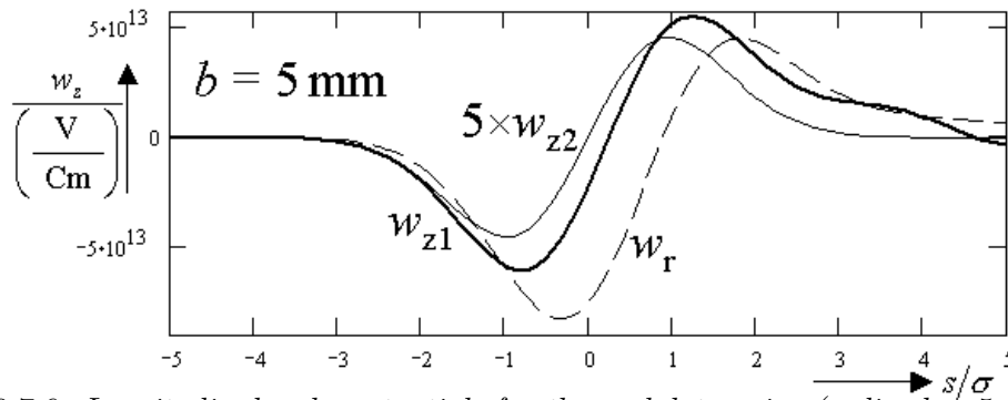
Figure 9.7.6: Longitudinal wake potentials for the undulator pipe (radius b = 5 \text{ mm} ). w_{z1} and w_{z2} are the wakes caused by the model surface structures \delta r_{1p} and \delta r_{2p} (figure 9.7.5) describing the measured surface shown in figure 9.7.3. For comparison, the resistive wake potential w_r is shown. The bunch tail is to the right.
