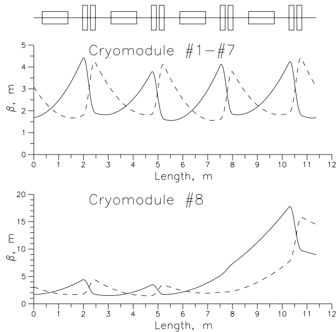
Figure 4.4.9: \beta -functions for the eight CM-1 modules.
