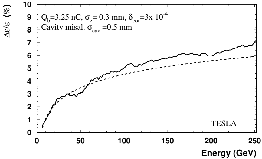
Figure 3.2.5: Vertical emittance growth obtained from computer simulation of 50 random seeds of cavity misalignments ( \delta y_c=0.5 mm rms). The dashed curve is the analytical prediction from a two-particle model.
