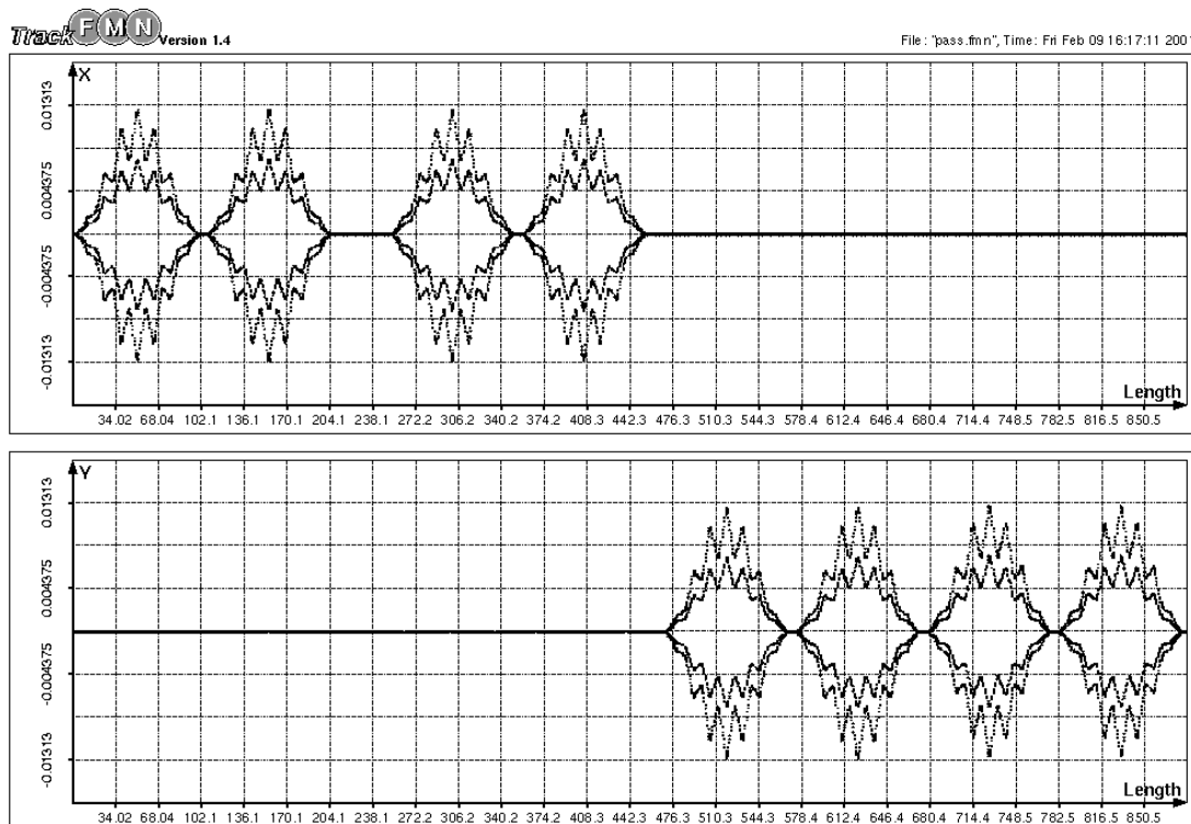
Figure 9.6.7: Tracked trajectories of off-energy particles, taking into account all non-linearities, along the complete arc deflecting and elevating the XFEL electron beam from the TESLA collider tunnel. The energy deviation is \pm 3\% (inner trajectories) and \pm 5\% .
