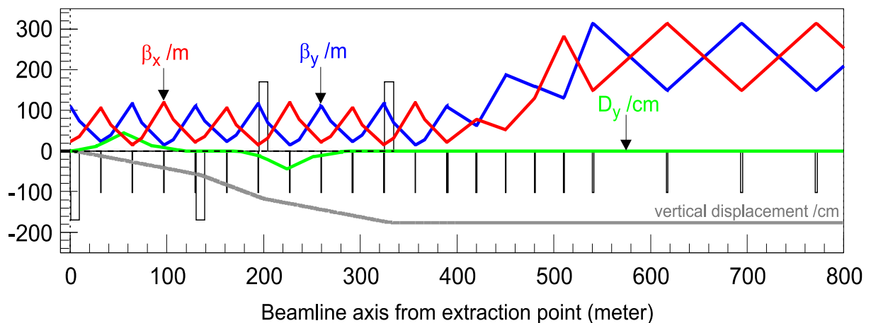
Figure 9.6.1: Electron optics in the first part of the transfer line. Quadrupoles and dipoles are marked by vertical boxes (dipole boxes are field sign dependent). The vertical orbit displacement (black curve, scale in cm) is shown versus the distance from the extraction point in the lower part of the figure. The achromat ranges from 0 to 390 m, the matching cells extend up to 540 m followed by the first cells of the transfer line.
