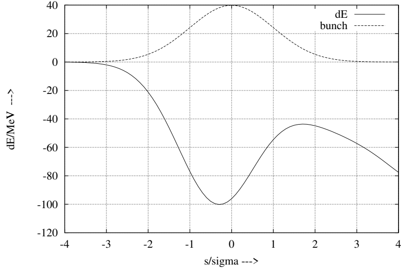
Figure 9.1.7: Accumulated longitudinal wake potential at the undulator entrance versus the longitudinal position s (in unit of rms bunch length) inside the bunch. The broken line indicates a Gaussian bunch profile with \sigma = 25 \mu\text{m} bunch length (1 nC charge) which was used in the calculation. The bunch tail is to the right.
