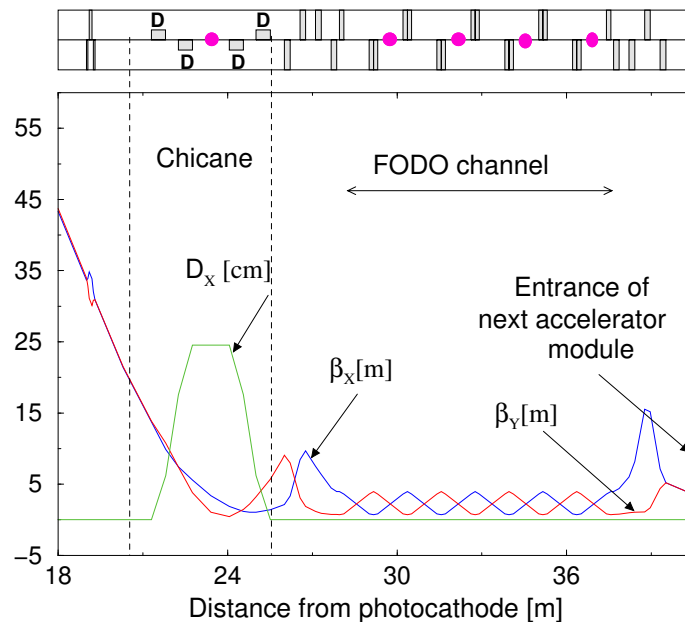
Figure 9.3.5: Optical lattice functions along the compressor and matching/diagnostic section. The dipoles and quadrupoles are indicated by rectangular boxes (D: dipole) and beam profile monitors by magenta bullets in the upper part.
