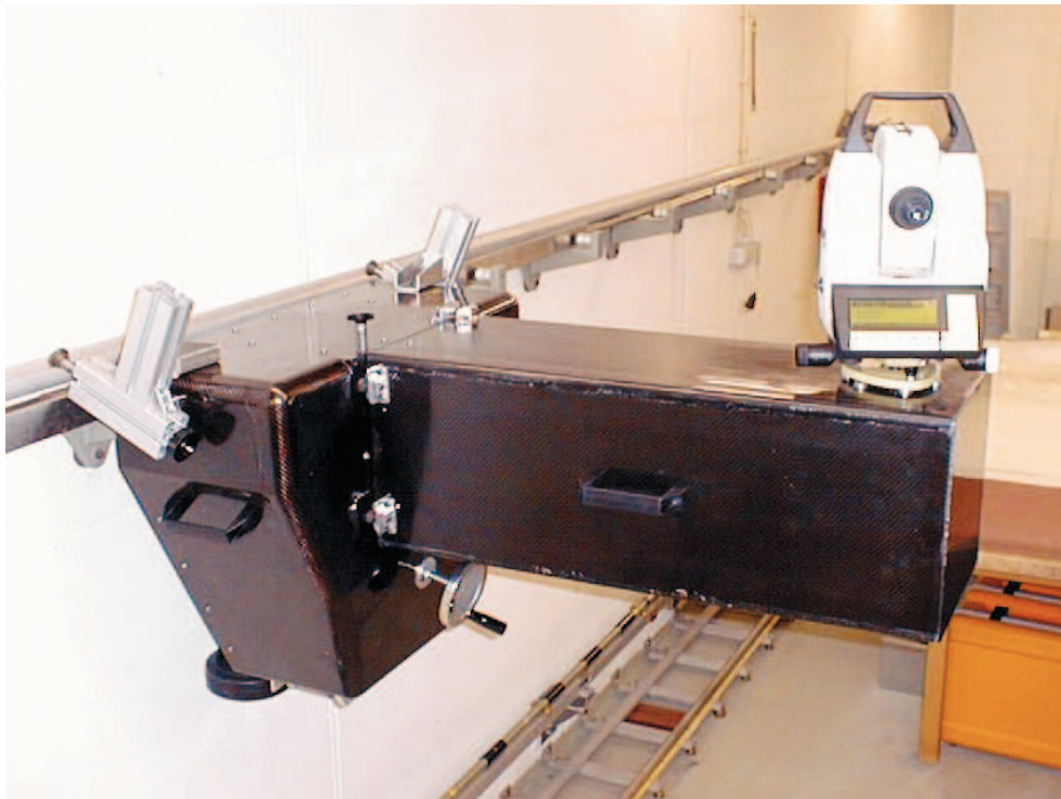
Figure 8.6.1: Installation of the tachymeter on a moveable carriage.
