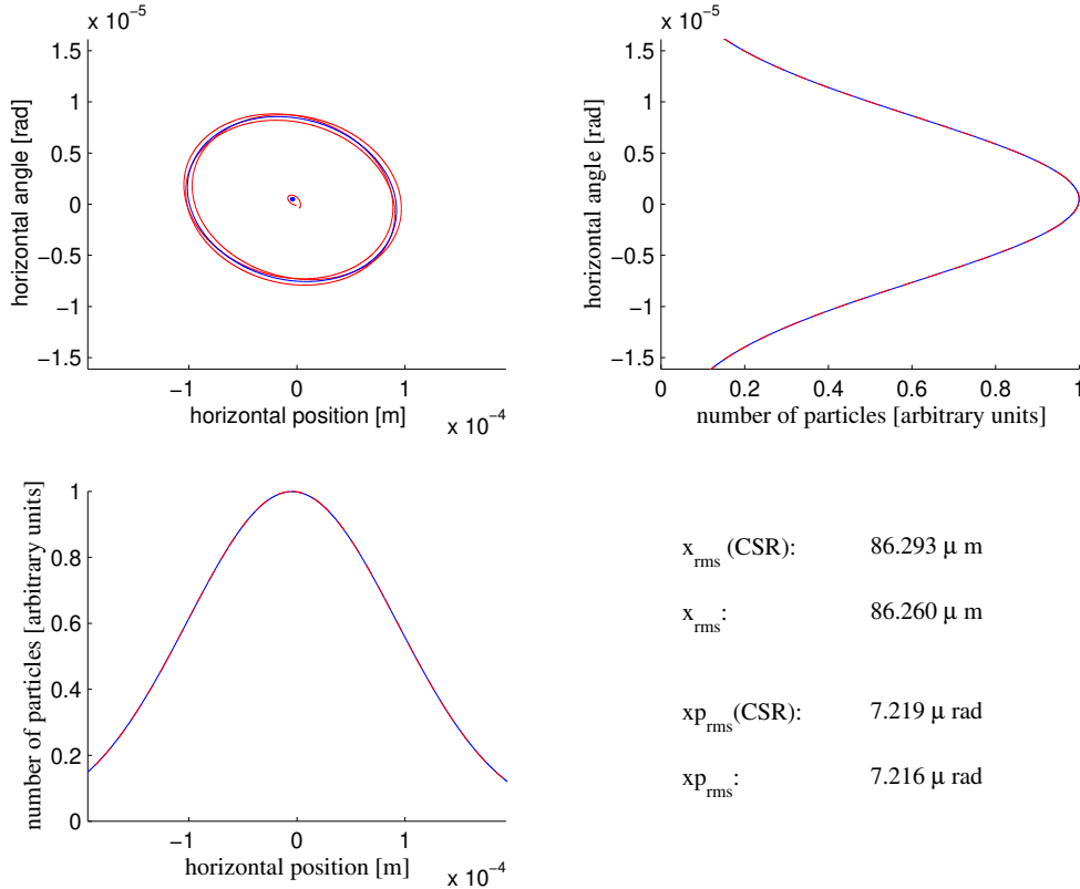
Figure 6.2.4: TraFiC4 -calculation of emittance growth due to Coherent Synchrotron Radiation effects. Shown are horizontal phase space and projections (red lines/dots: with CSR, blue lines/dots: without CSR). Upper left: horizontal phase space with longitudinal bunch slice centres and 1\sigma -ellipses. Upper right: projection of particle angles. Lower left: projection of particle positions.
