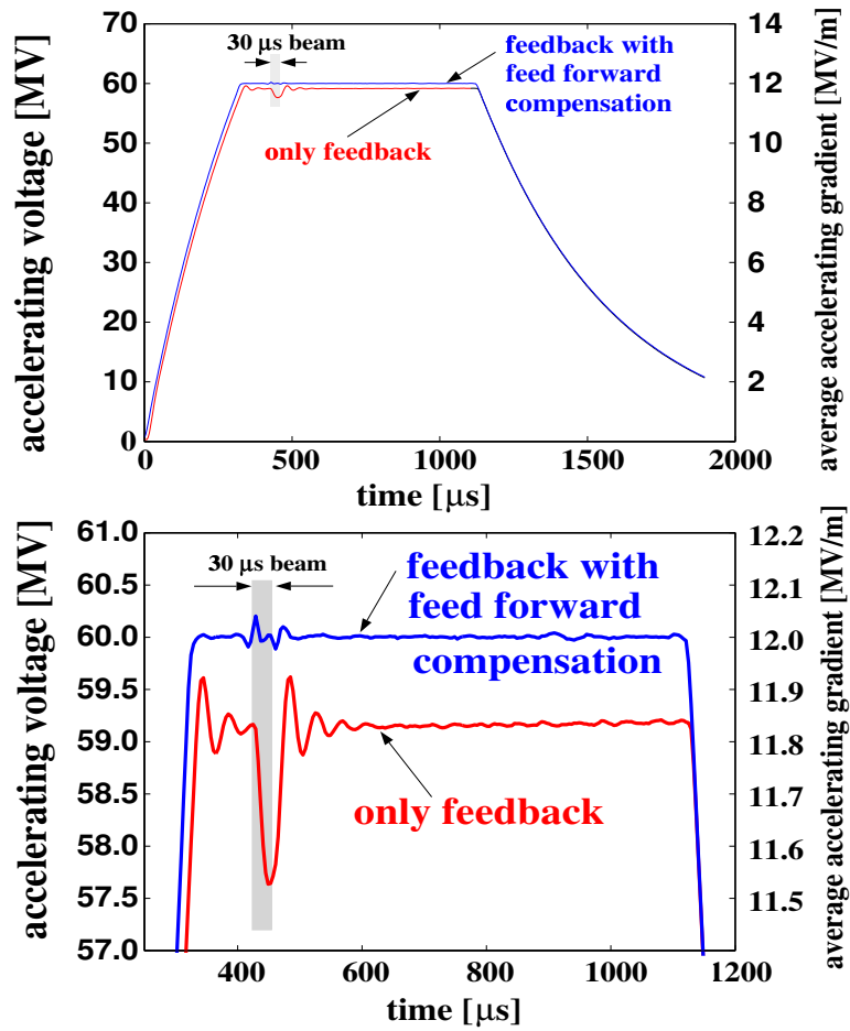
Figure 3.4.8: Field stability with and without adaptive feed forward.
