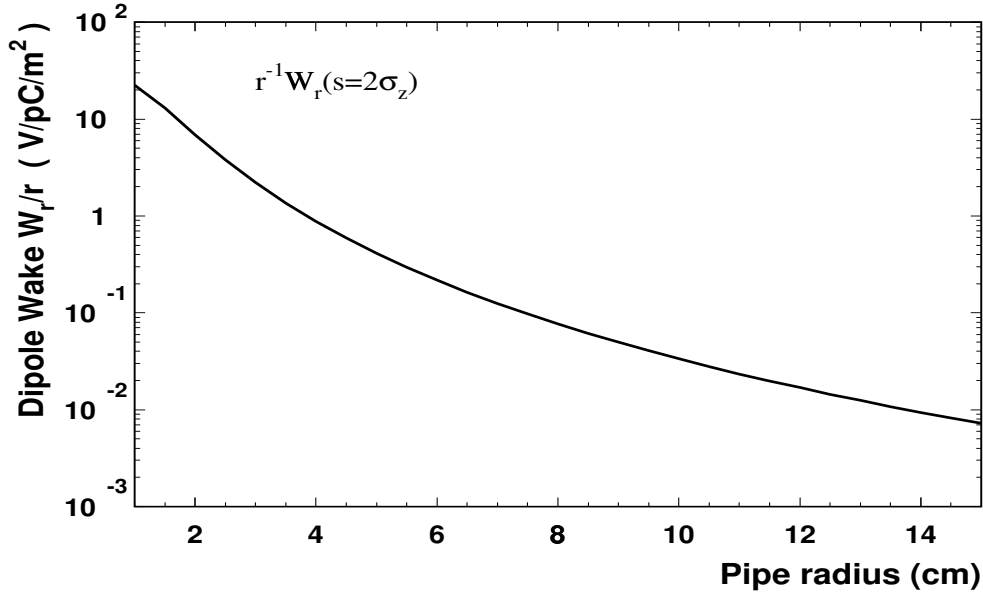
Figure 9.7.2: Transverse resistive wake potential W_{\perp} ( s = 2\sigma_z ) versus tube radius. It is normalised to 1 m transverse orbit displacement and 1 m tube length.
