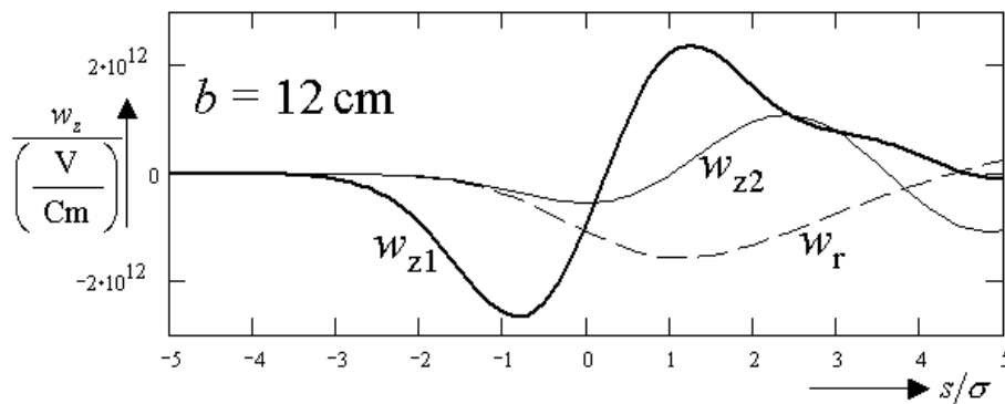
Figure 9.7.7: Longitudinal wake potentials for the transfer pipe ( b = 12 \text{ cm} ).
