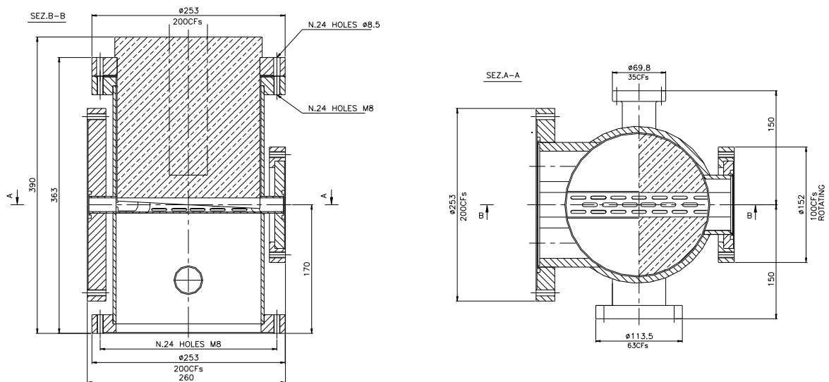
Figure 5.6.7: Synchrotron radiation absorber.
