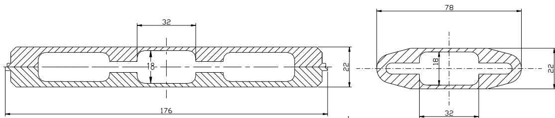
Figure 5.6.6: Wiggler vacuum chamber with ante-chamber (left), and wiggler cell quadrupole vacuum chamber (right).
