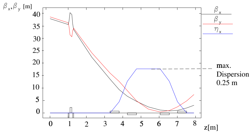
Figure 9.4.2: Optics in the region of Bunch Compressor 1.
