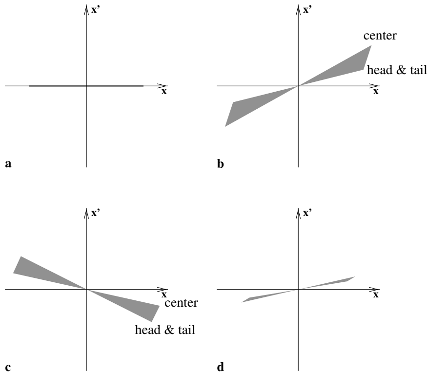
Figure 9.3.2: Transverse phase space plots showing schematically transverse emittance growth and reduction due to space charge forces. (a) Initial phase space with small (zero) emittance at the gun. (b) Phase space after transport up to the solenoid lens, showing the growth of the projected emittance due to the different focusing strength at the bunch centre and the tails. (c) The phase space distribution has been rotated by an external focusing kick. (d) Phase space after a drift behind the lens. The projected emittance is decreased due to the action of the space charge forces.
