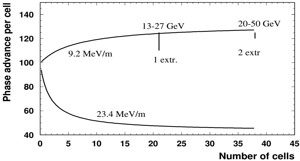
Figure 9.5.1: Phase advance per FODO cell (in degrees) of the main linac for the FEL beam operating at different acceleration gradients.
