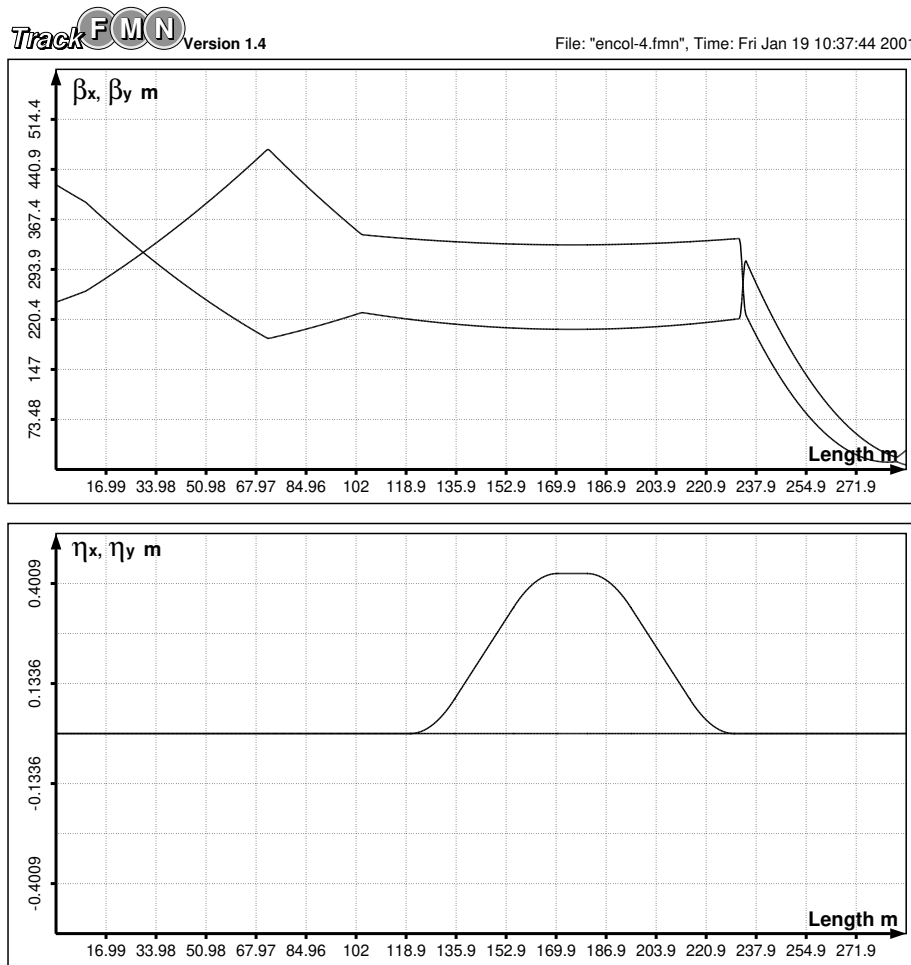
Figure 9.6.5: Optical functions in the energy collimation section and the matching telescope, connecting the transverse collimation section (on the left side) and the beam elevation arc (on the right side).
