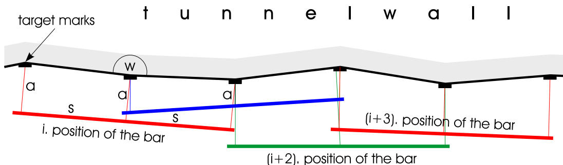
Figure 8.6.4: Straightness measurements with multi-point alignment.
