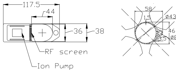
Figure 5.6.5: Dipole vacuum chamber with distributed ion pump (left), and quadrupole vacuum chamber (right).
