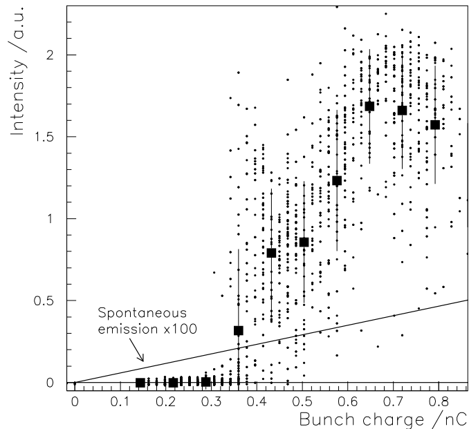
Figure 9.2.3: SASE FEL intensity versus bunch charge. The straight line is the spontaneous intensity multiplied by a factor of 100. To guide the eye, mean values of the radiation intensity are shown for some bunch charges (full squares). The vertical error bars indicate the standard deviation of intensity fluctuations, which are not an indication of machine instability but are due to the statistical character of the SASE process. For this measurement all accelerator settings were kept constant, except for the bunch charge. Above 0.6 nC there is no further increase of gain without readjustment of accelerator settings which would be necessary to compensate for the changed phase space distribution of the electron bunch.
