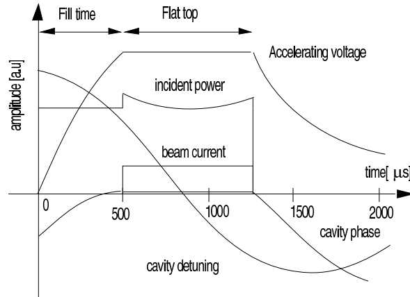
Figure 3.4.6: Various parameters related to the pulsed cavity fields in the superconducting cavities of the TESLA Test Facility.
