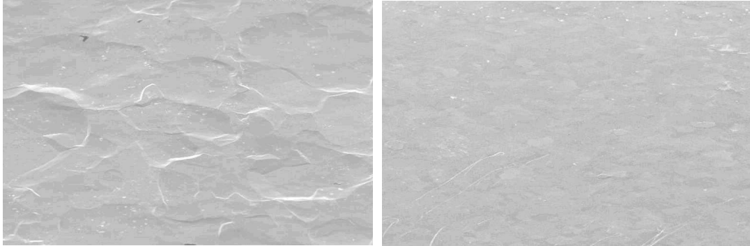
Figure 2.1.13: SEM micrographs of niobium surface after BCP (left) and EP (right). The average surface roughness is 1\ \mu\text{m} in the left and 0.1\ \mu\text{m} in the right sample. Height of micrograph is 500\ \mu\text{m} (Courtesy of CERN).
