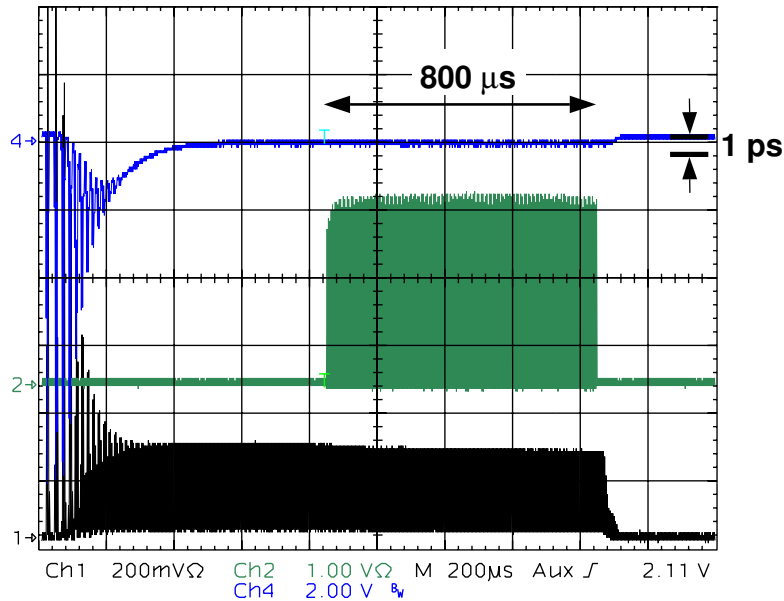
Figure 9.3.7: Oscilloscope trace of the output of the pulse train oscillator (PTO) (trace 1), the phase of the pulses relative to the reference (trace 4), and the pulse train after amplification measured in the green with a fast photodiode (trace 2). The data have been taken at the TTF laser system, which is running with 800\ \mu\text{s} long pulse trains. Note, that due to the scale ( 200\ \mu\text{s} per div.) individual pulses in the train are not resolved.
