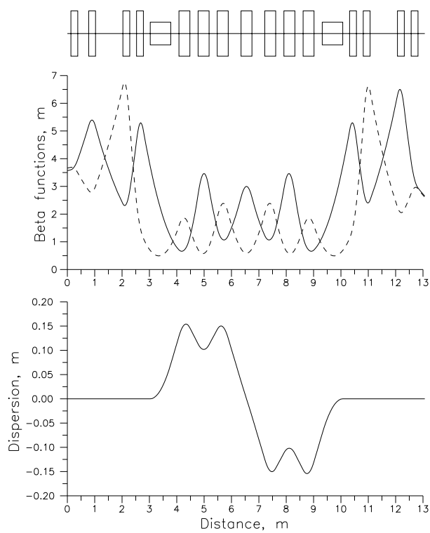
Figure 4.4.3: Optical functions in the separator section.
