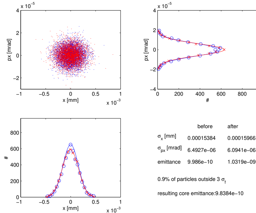
Figure 6.4.2: Horizontal phase space before (blue) and after (red) tracking through the fifteen-degree arc. The rms energy spread of the beam is 3%.
