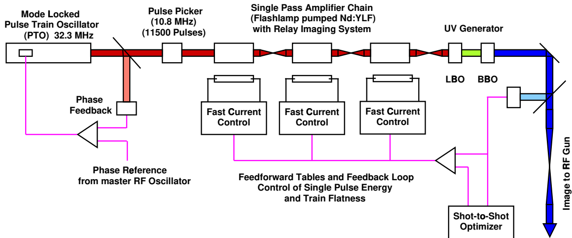
Figure 9.3.6: Schematic overview of the photoinjector laser system.
