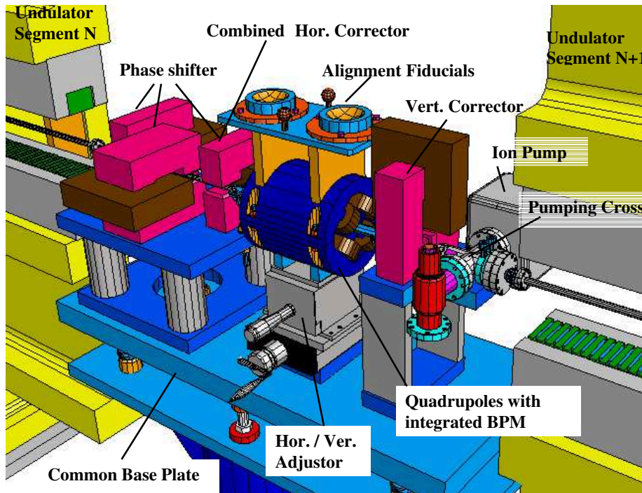
Figure 9.8.2: 3D view of an undulator intersection.
