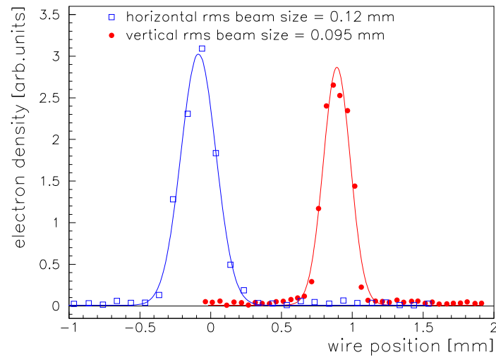
Figure 9.2.5: Typical transverse beam profiles measured with the wire scanners installed at the undulator section.
