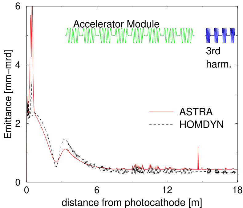
Figure 9.3.3: Development of the transverse emittance in the gun, the accelerator module and the third harmonic section.
