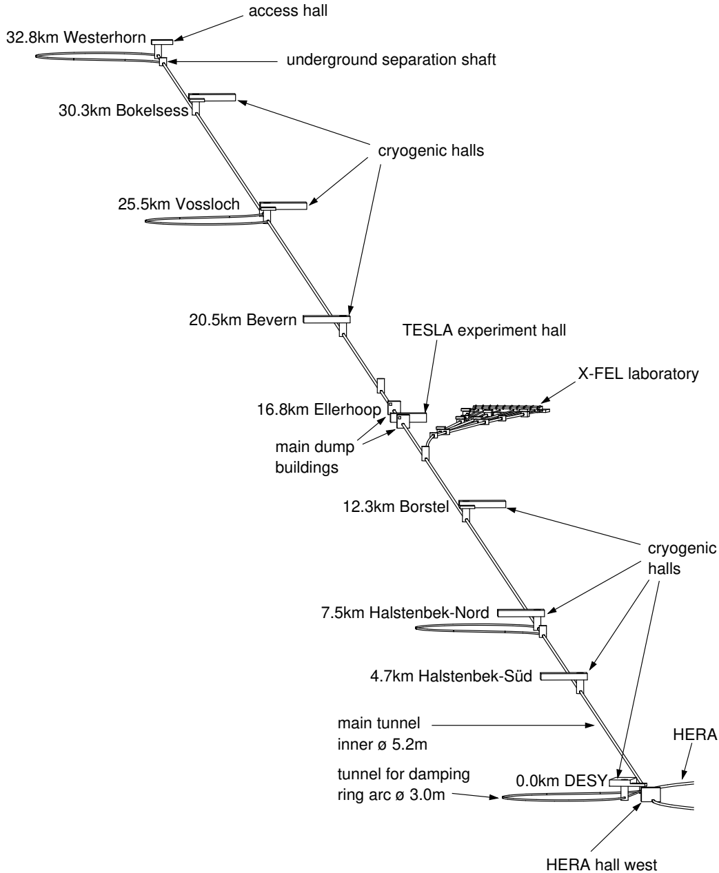
Figure 8.1.1: Schematic layout of the TESLA facility.
