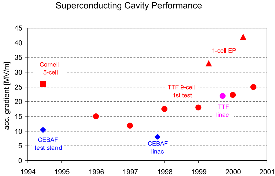
Figure 1.1.2: Evolution of superconducting cavity performance: red dots show the average gradient achieved with TESLA 9-cell cavities for the years 1995–2000 (first test, no additional processing), the red square shows results for 5-cell cavities at Cornell and the magenta dot depicts the average gradient measured with beam for a complete accelerator module installed at the TTF linac. Red triangles show gradients obtained with electropolished single-cell resonators (see text). Test stand and linac operation results from Jefferson Lab (CEBAF) are included for comparison (blue diamonds).
