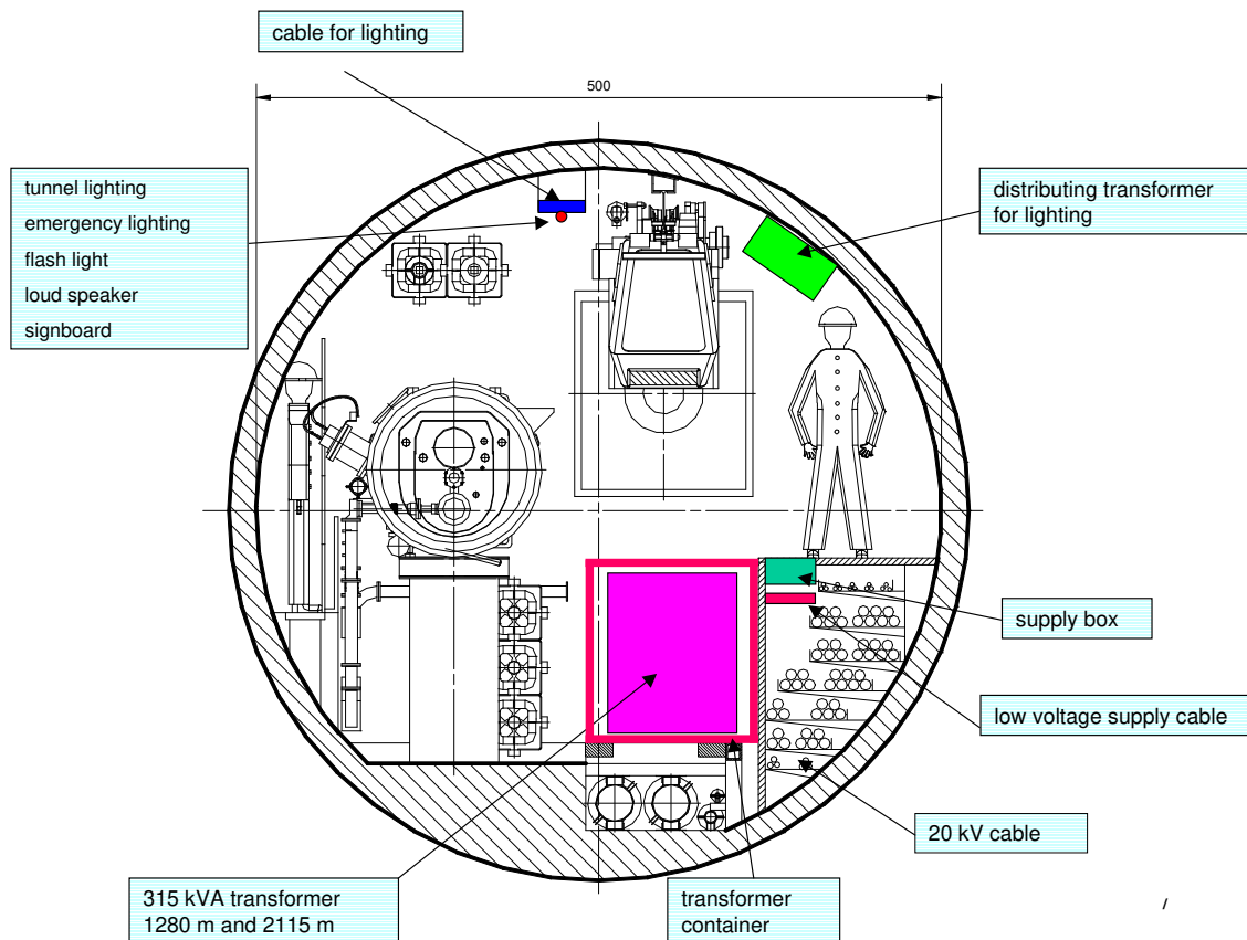
Figure 8.4.2: Power distribution in the tunnel.
