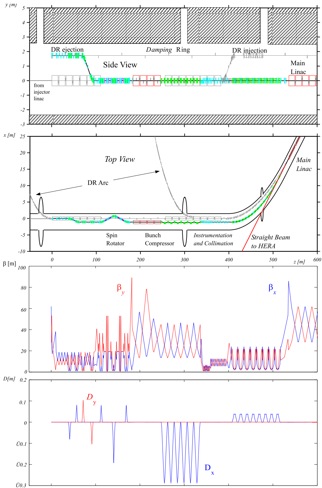
Figure 6.5.1: Floor plan, betatron functions and dispersion for the complete beamline. In the floor plan, bending magnets are green, quadrupoles blue, RF cavities red and solenoid magnets magenta. The damping ring components and those of the injector linac are shaded in grey.
