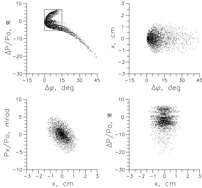
Figure 4.4.5: Positrons phase space plots at the PPA exit.
