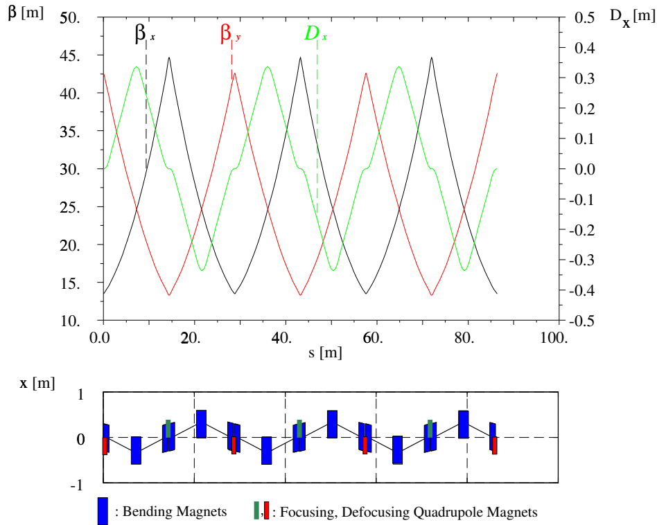
Figure 6.2.1: Optical functions and floor plan of the wiggler bunch compressor: horizontal (black) and vertical (red) betatron function and horizontal dispersion (green).
