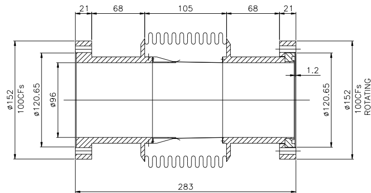
Figure 5.6.9: RF screened bellows.
