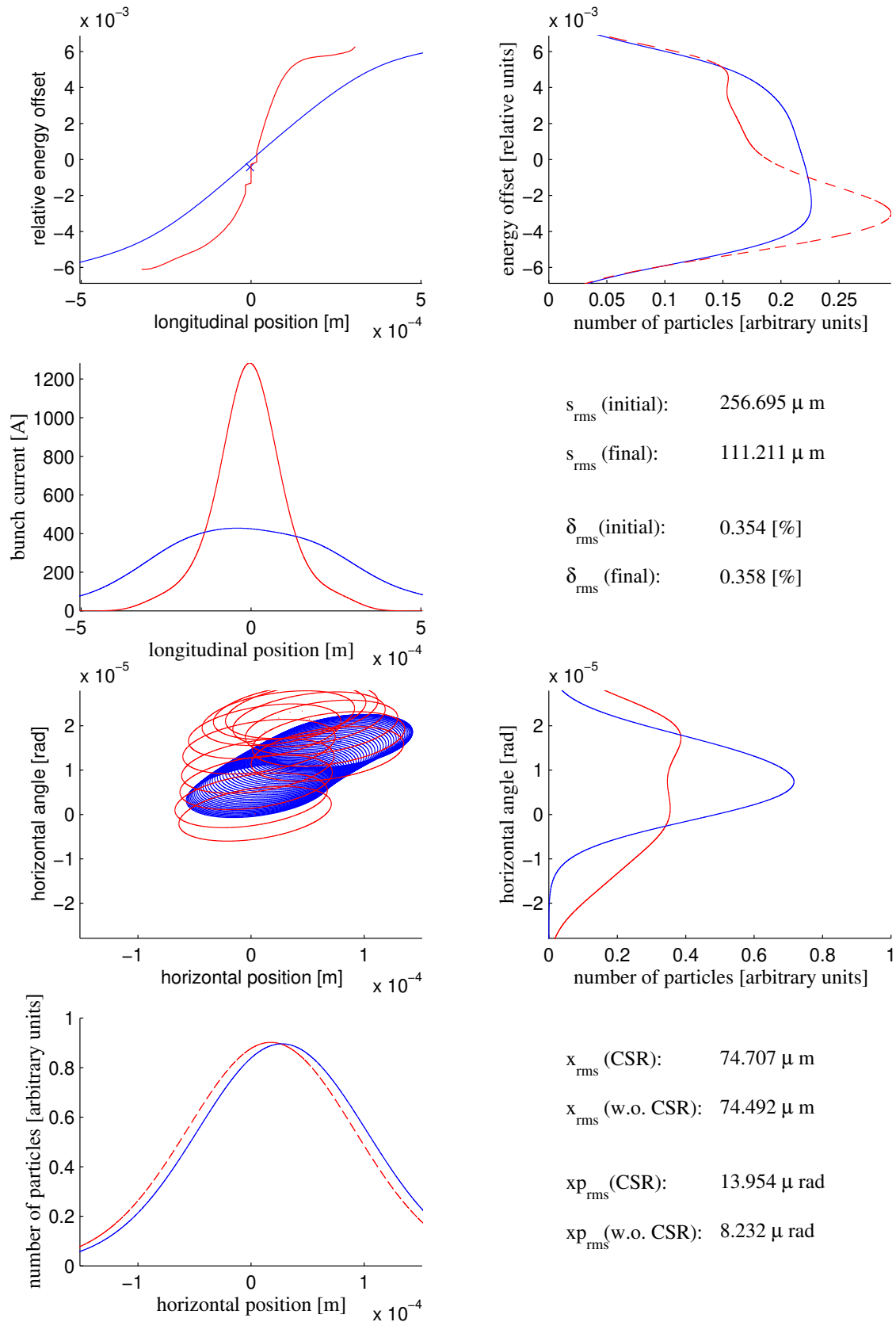
Figure 9.4.7: Longitudinal phase space before (blue) and after (red) Bunch Compressor 2 and transverse phase at the compressor exit space without (blue) and with (red) CSR, respectively.
