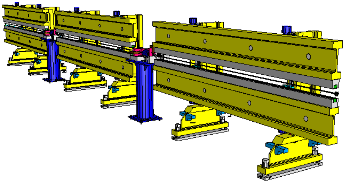
Figure 9.8.1: 3D view of 3 cells of the undulator system.
