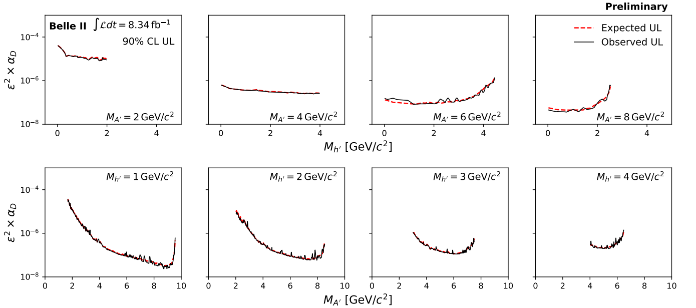
FIG. S8: Observed 90% CL upper limits on \varepsilon^2 \times \alpha_D (solid black line) and their expected values (dotted red line) ( top ) as functions of M_{h'} for four values of M_{A'} and ( bottom ) as functions of M_{A'} for four values of M_{h'} .
