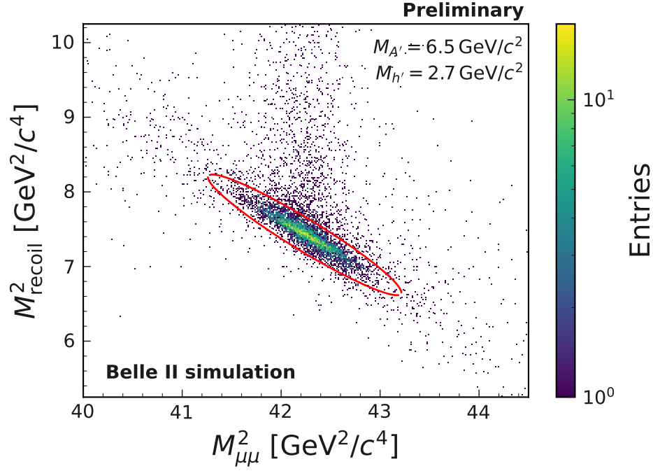
FIG. S1: Example of a two-dimensional squared mass distribution for a given signal hypothesis ( M_{A'}=6.5 \text{ GeV}/c^2 , M_{h'}=2.7 \text{ GeV}/c^2 ). The upward tail in the squared recoil mass distribution is due to ISR. Also shown is the elliptical search window contour.
