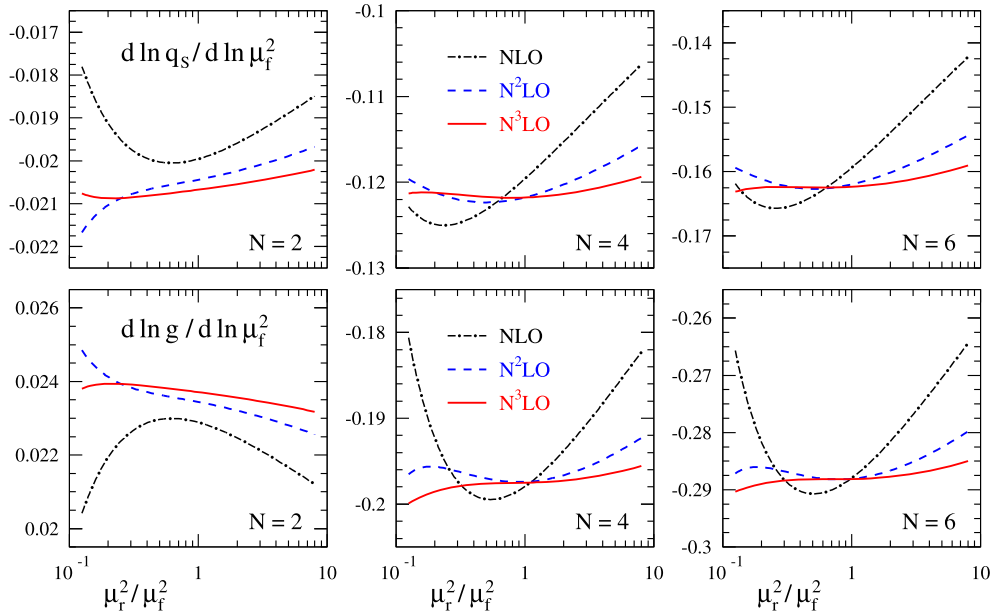
Fig. 2. The dependence of the logarithmic factorization-scale derivatives of the singlet PDFs on the renormalization scale \mu_r at N = 2 (where the very small scaling violations of q_s and g are related by the momentum sum rule), N = 4 and N = 6 for the initial distributions (37).
